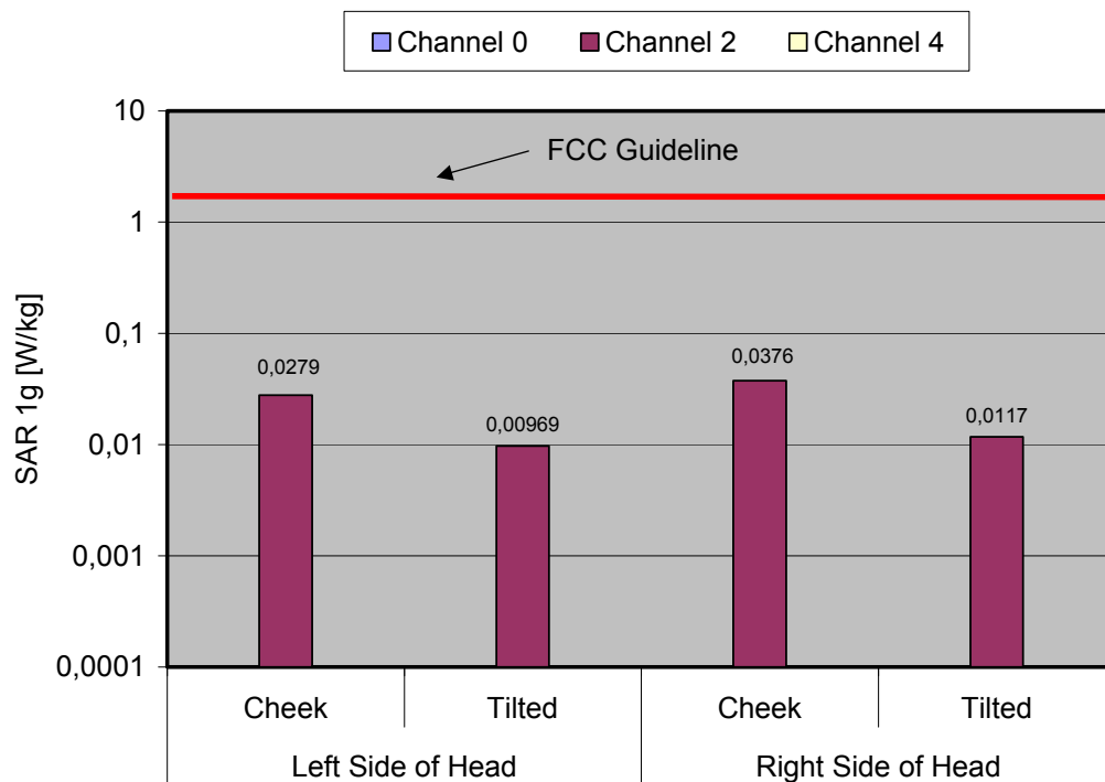
Fig. 8: The measured head phantom SAR values for the Bang & Olufsen BeoCom4 Handset, for the US DECT standard in comparison to the FCC exposure limit.
