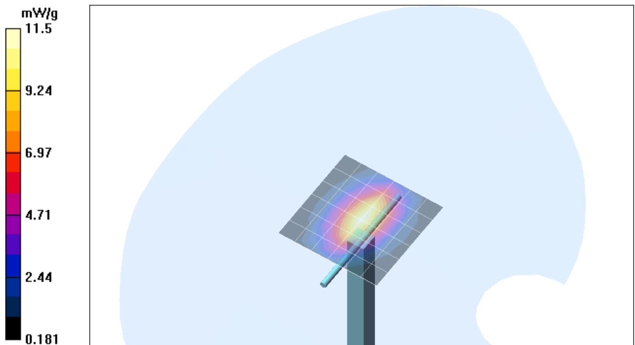
Fig. 10: Validation measurement 1900 MHz Head (June 27, 2006), coarse grid. Ambient Temperature: 22.0° C, Liquid Temperature: 21.4° C.
