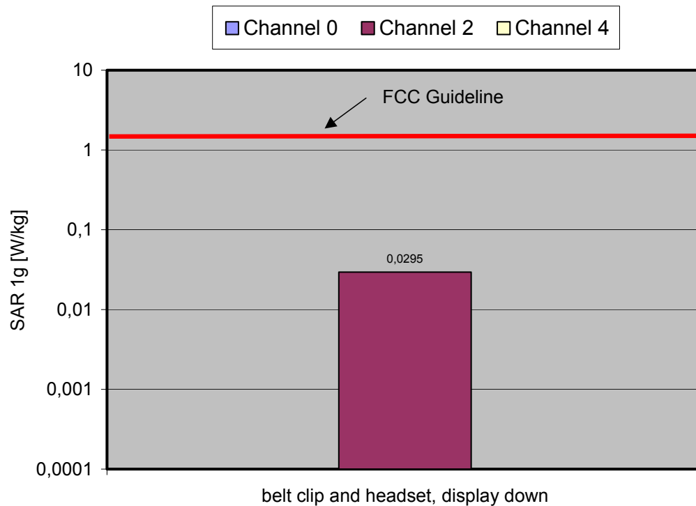
Fig. 9: The measured SAR values in body-worn configuration for the Bang & Olufsen BeoCom4 Handset for the US DECT standard in comparison to the FCC exposure limit.
