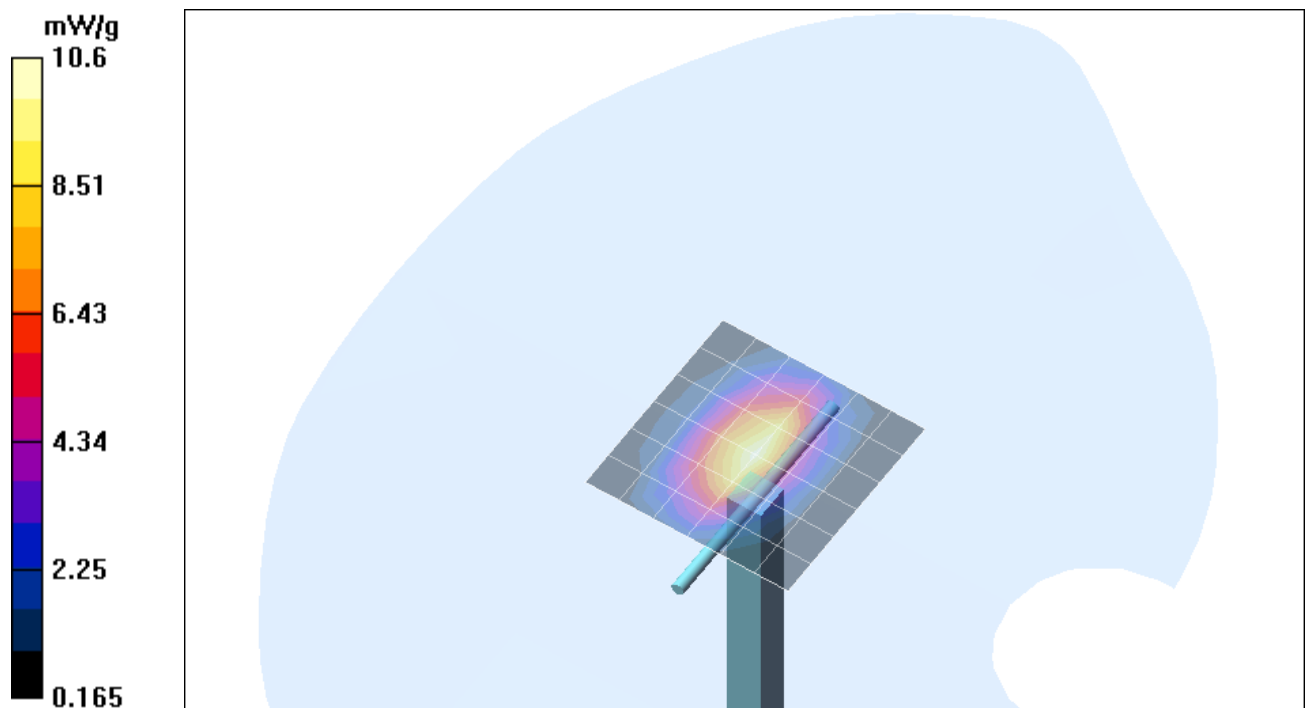
Fig. 11: Validation measurement 1900 MHz body (June 26, 2006), coarse grid. Ambient Temperature: 22.0° C, Liquid Temperature: 21.1° C.
