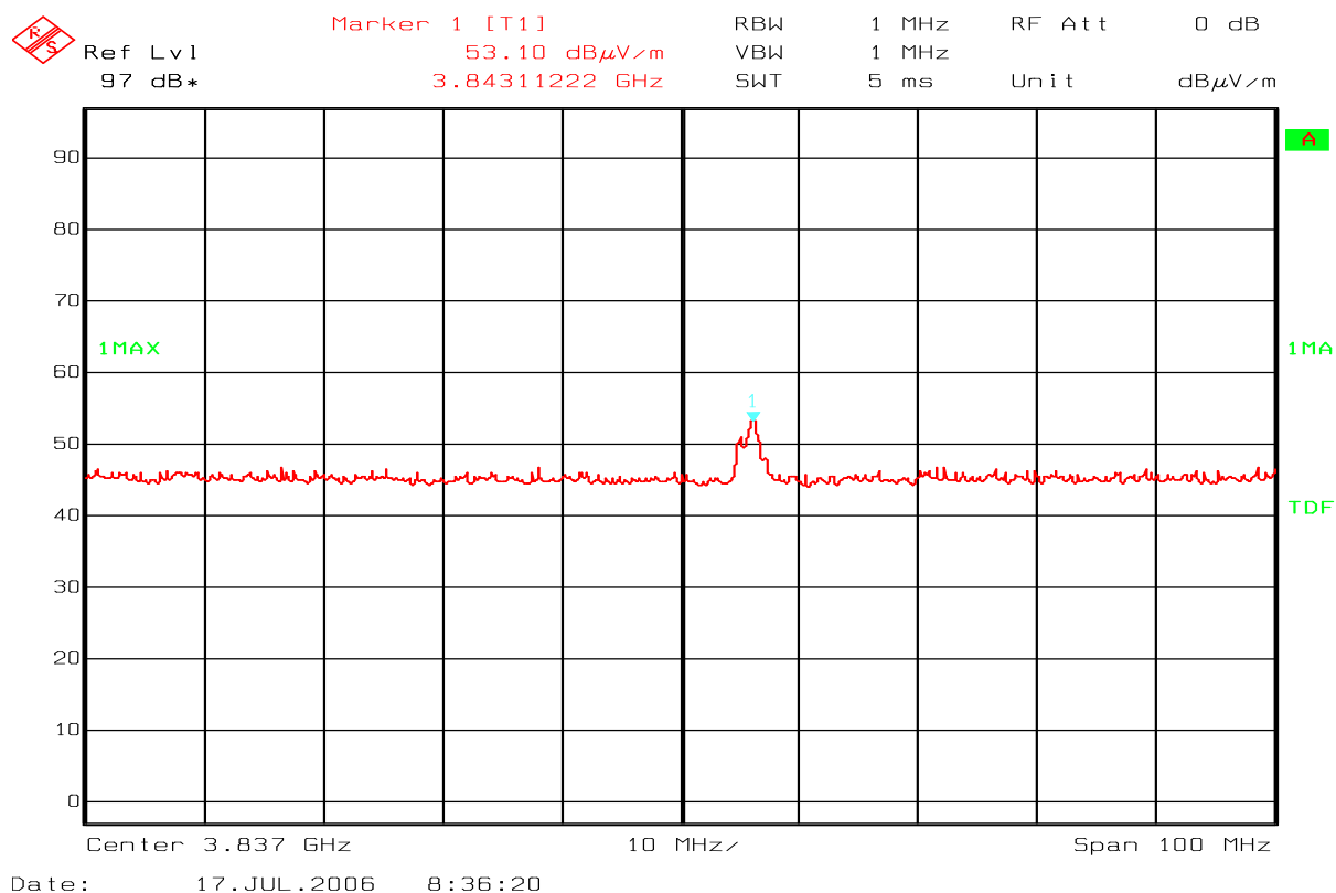
Spurious Emissions 3.84 GHz (Second Harmonic)
