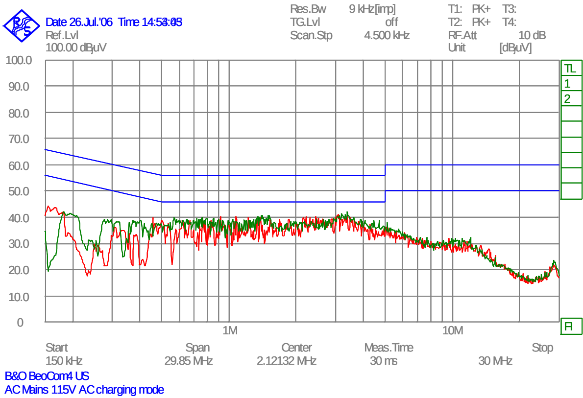
Power Line Conducted Emissions, Phase L1 and N, Handset Charging, Peak Detector
