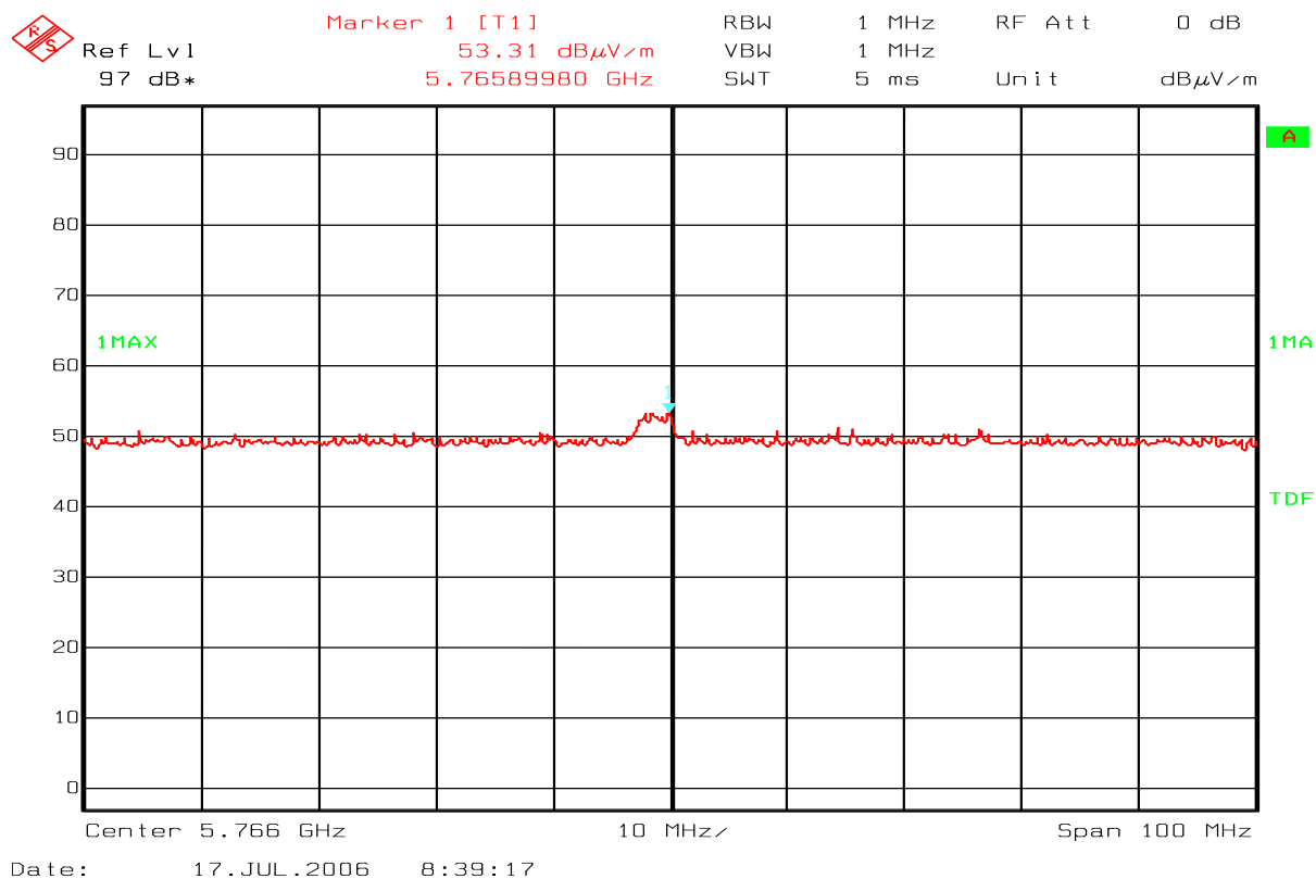
Spurious Emissions 5.76 GHz (Third Harmonic)
