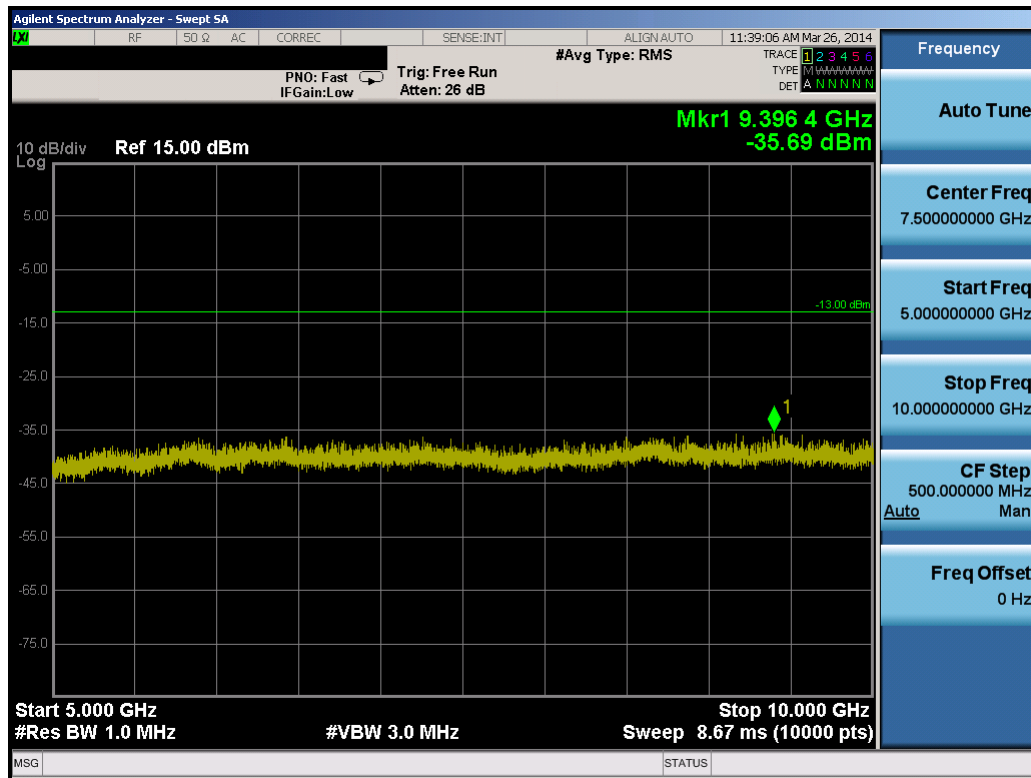
Plot 8-8. Conducted Spurious Plot
