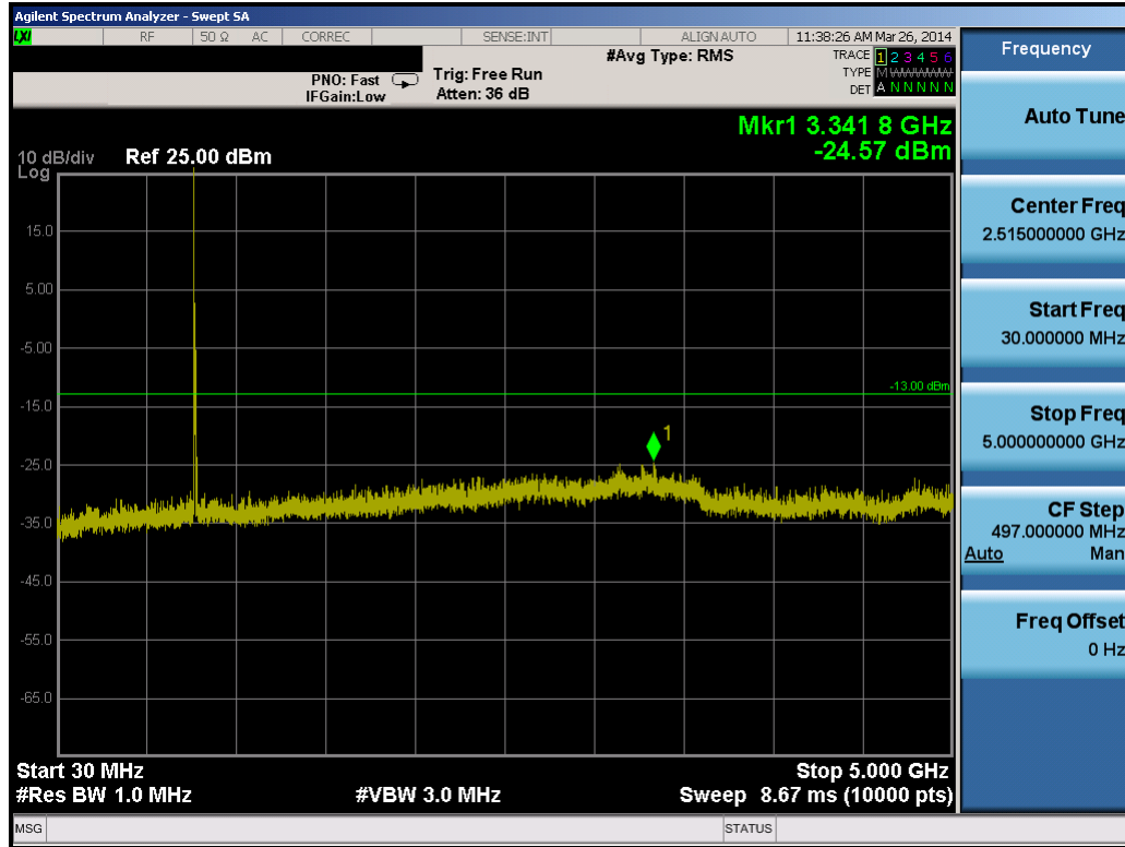
Plot 8-7. Conducted Spurious Plot
