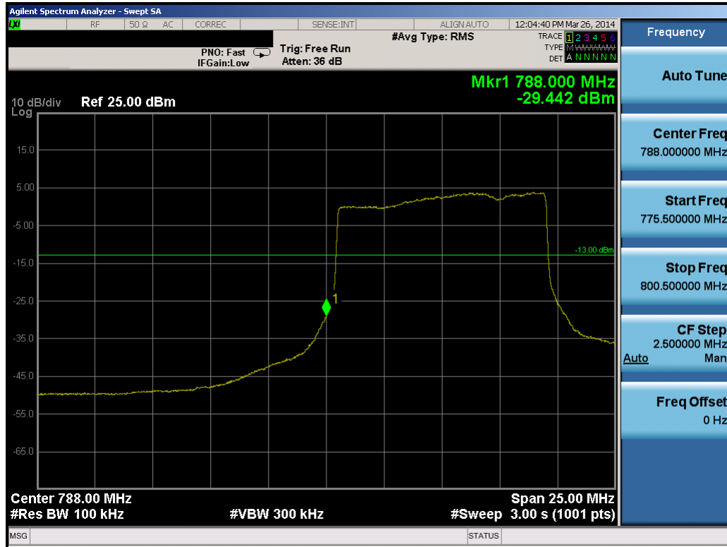
Plot 8-1. Lower Band Edge Plot (QPSK, 50RB)
