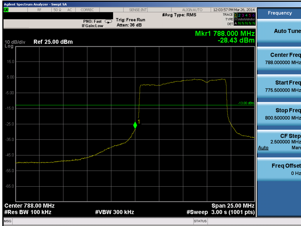
Plot 8-2. Lower Band Edge Plot (16QAM, 50RB)
