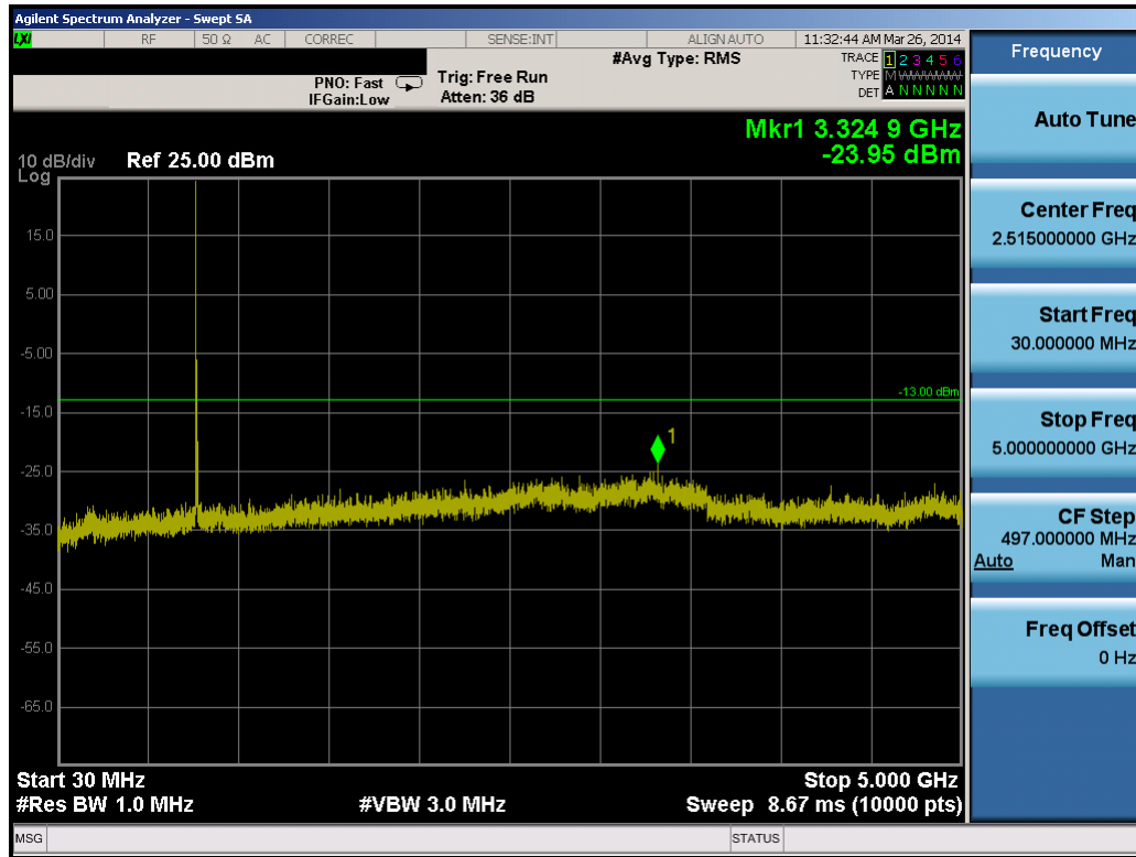
Plot 7-7. Conducted Spurious Plot
