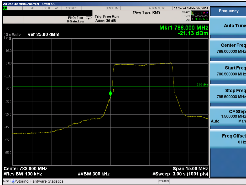
Plot 7-1. Lower Band Edge Plot (QPSK, 25RB)
