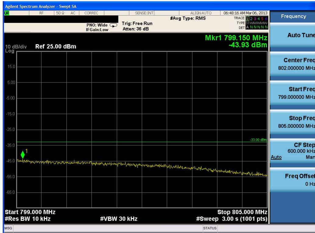
Plot 8-9. Conducted Emissions Mask (799-805 MHz) Plot (QPSK, 50RB)
