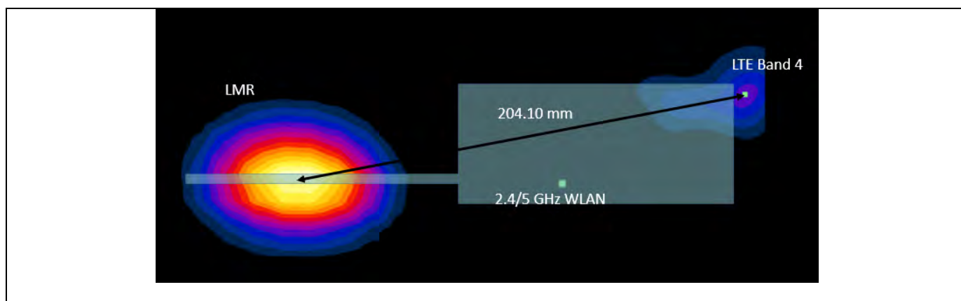
Figure 11-4 Back Side SAR to Peak Location Separation Ratio Plots
