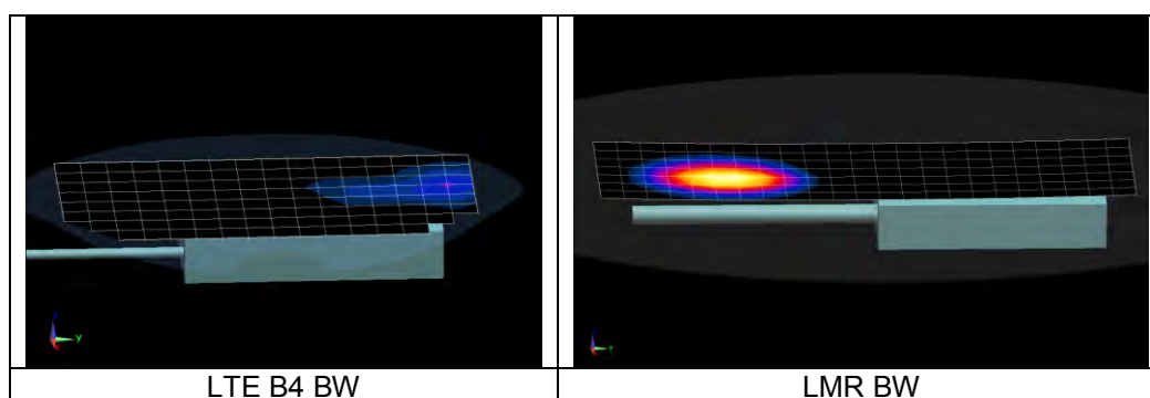
Figure 11-4 Back Side SAR to Peak Location Separation Ratio Plots
