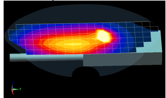
Figure 11-2 VHF Body-Worn Worst Case Area Scan
