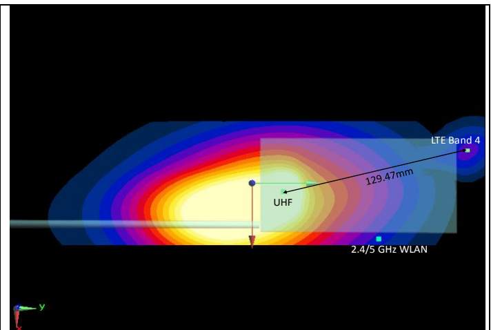
Figure 11-4 Back Side SAR to Peak Location Separation Ratio Plots
