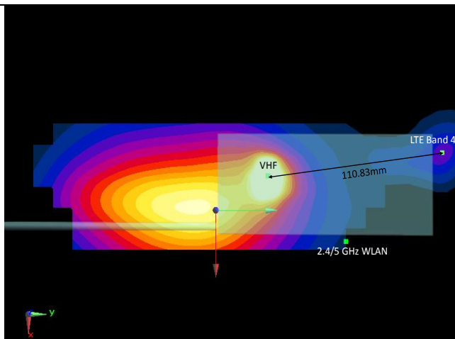
Figure 11-4 Back Side SAR to Peak Location Separation Ratio Plots
