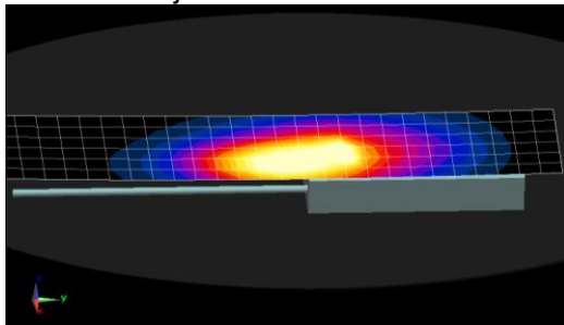
Figure 11-4 Back Side SAR to Peak Location Separation Ratio Plots
