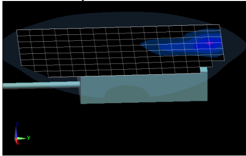
Figure 11-1 LTE B4 Body-Worn Worst Case Area Scan
