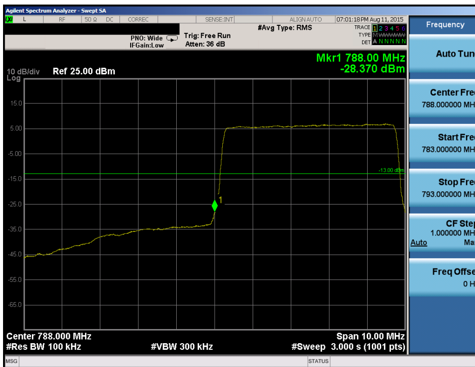
Plot 7-2. Lower Band Edge Plot (16QAM, 25RB)
