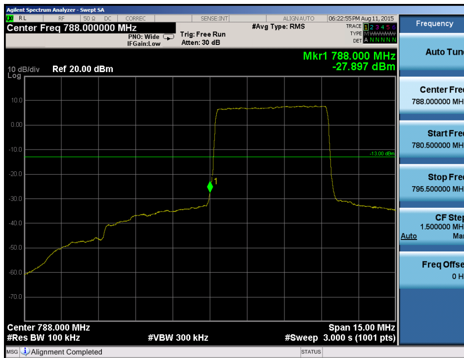
Plot 7-1. Lower Band Edge Plot (QPSK, 25RB)
