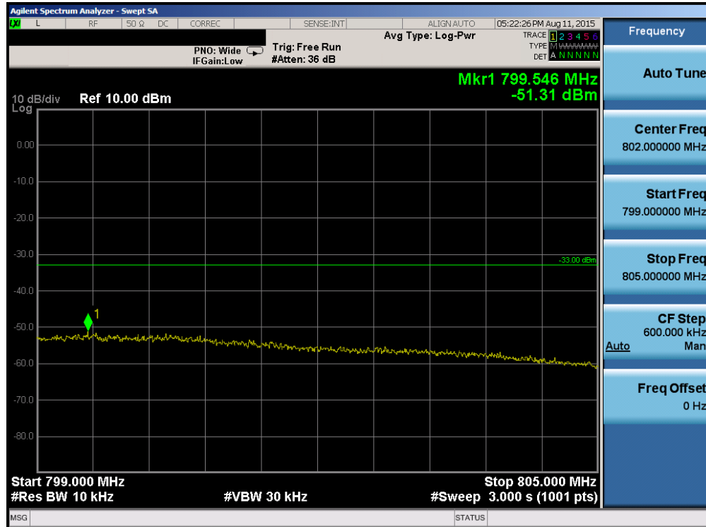
Plot 8-7. Upper Conducted Emissions Mask (799-805 MHz) Plot (QPSK, 50RB)
