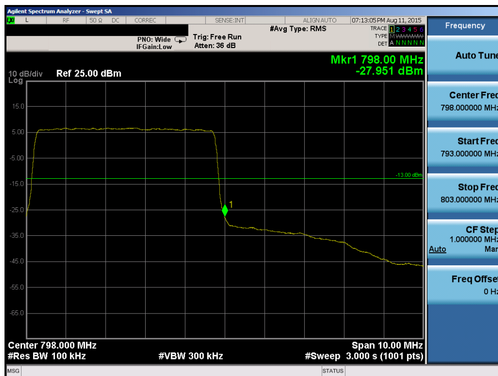
Plot 7-4. Upper Band Edge Plot (16QAM, 25RB)
