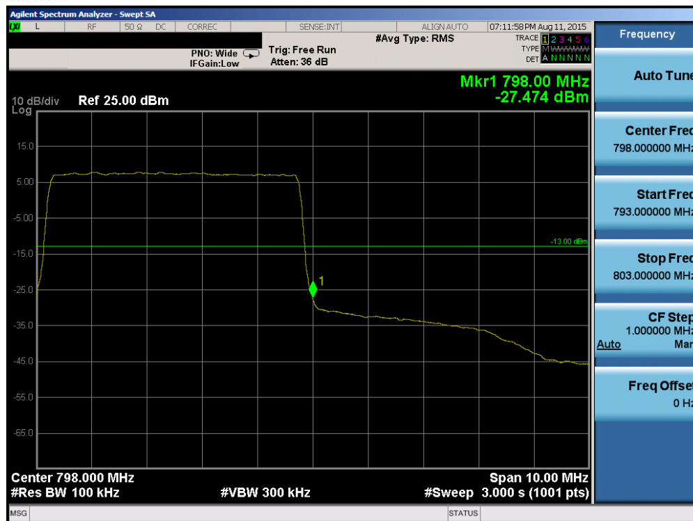
Plot 7-3. Upper Band Edge Plot (QPSK, 25RB)
