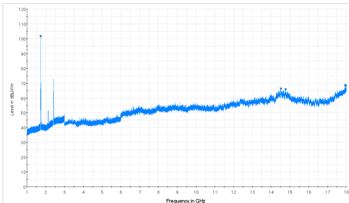
Plot 7-3. Radiated Spurious Plot from 1GHz – 18GHz (Whip Antenna: 14035-4000-01) (Pol. V)
