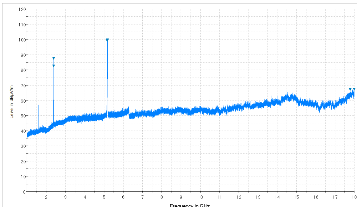
Plot 7-12. Radiated Spurious Plot from 1GHz – 18GHz (Whip Antenna: 14035-4420-01) (Pol. H)
