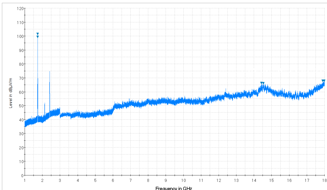
Plot 7-21. Radiated Spurious Plot from 1GHz – 18GHz (Whip Antenna: 14035-4420-01) (Pol. V)
