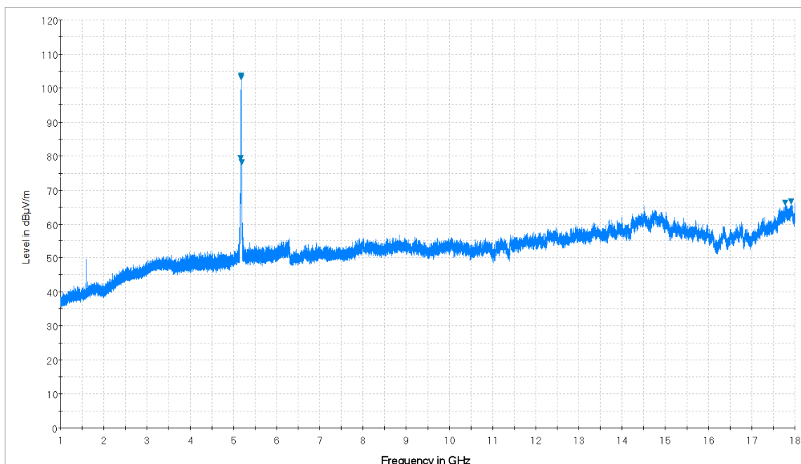
Plot 7-15. Radiated Spurious Plot from 1GHz – 18GHz (Whip Antenna: 14035-4440-01) (Pol. V)
