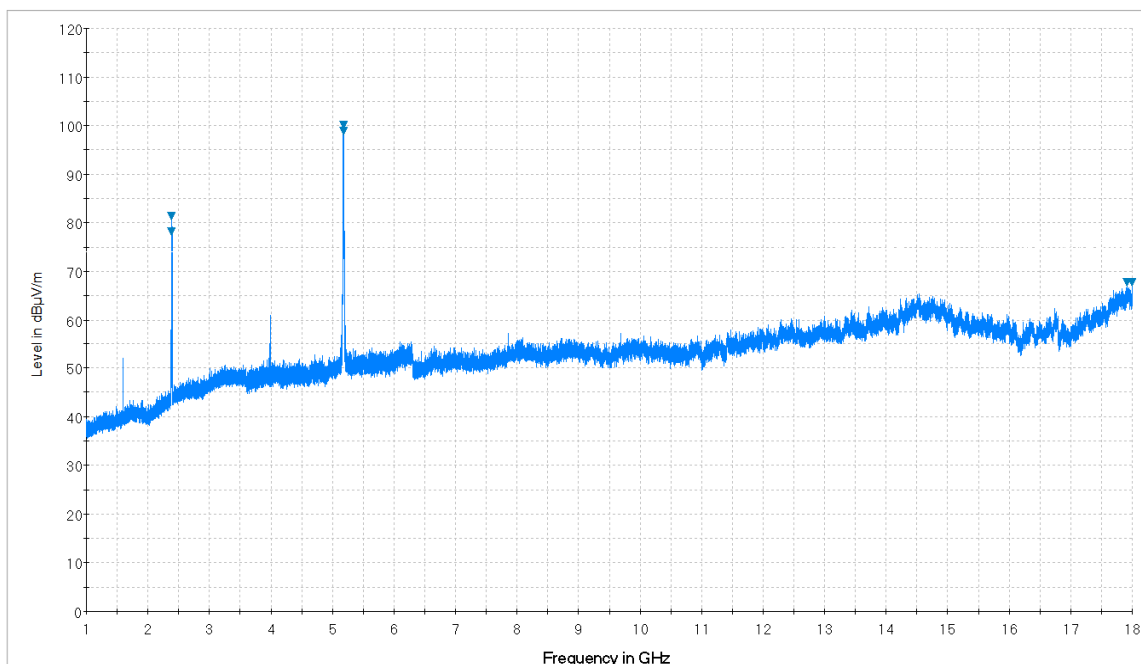
Plot 7-10. Radiated Spurious Plot from 1GHz – 18GHz (Whip Antenna: 14035-4000-01) (Pol. H)
