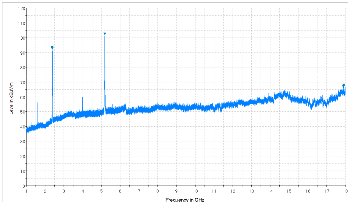
Plot 7-17. Radiated Spurious Plot from 1GHz – 18GHz (Whip Antenna: 14035-4440-02) (Pol. V)
