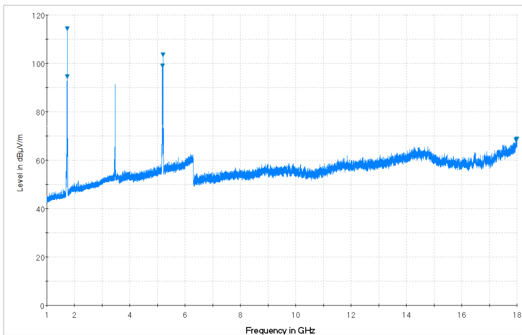
Plot 7-29. Radiated Spurious Plot from 1GHz – 18GHz (Whip Antenna: 14035-4420-01) (Pol. V)
