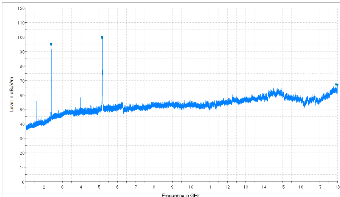
Plot 7-16. Radiated Spurious Plot from 1GHz – 18GHz (Whip Antenna: 14035-4440-02) (Pol. H)
