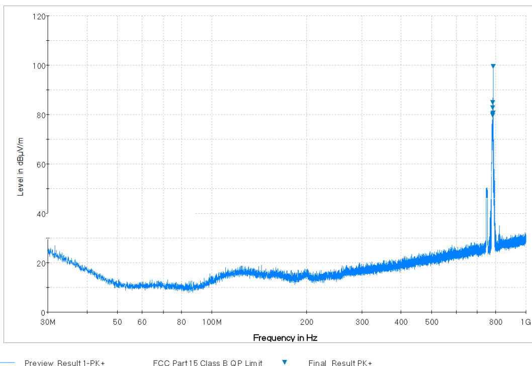
Plot 7-36. Radiated Spurious Plot from 30MHz - 1GHz (Whip Antenna: 14035-4420-01) (Pol. H)
