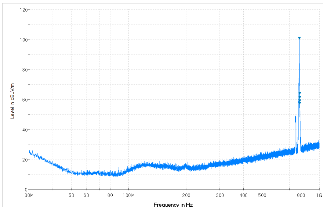
Plot 7-41. Radiated Spurious Plot from 30MHz - 1GHz (Whip Antenna: 14035-4440-02) (Pol. V)
