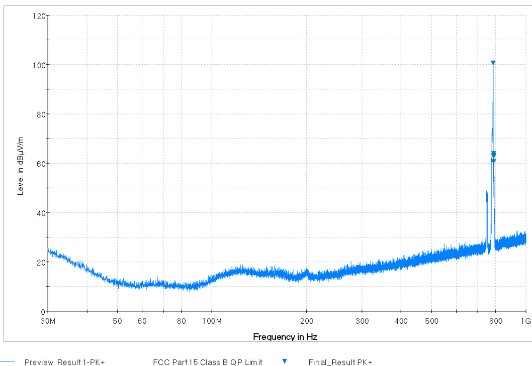
Plot 7-37. Radiated Spurious Plot from 30MHz - 1GHz (Whip Antenna: 14035-4420-01) (Pol. V)
