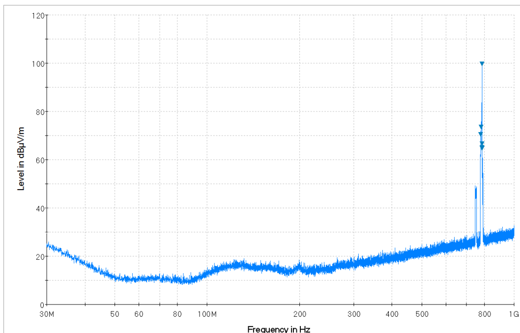
Plot 7-39. Radiated Spurious Plot from 30MHz - 1GHz (Whip Antenna: 14035-4440-01) (Pol. V)
