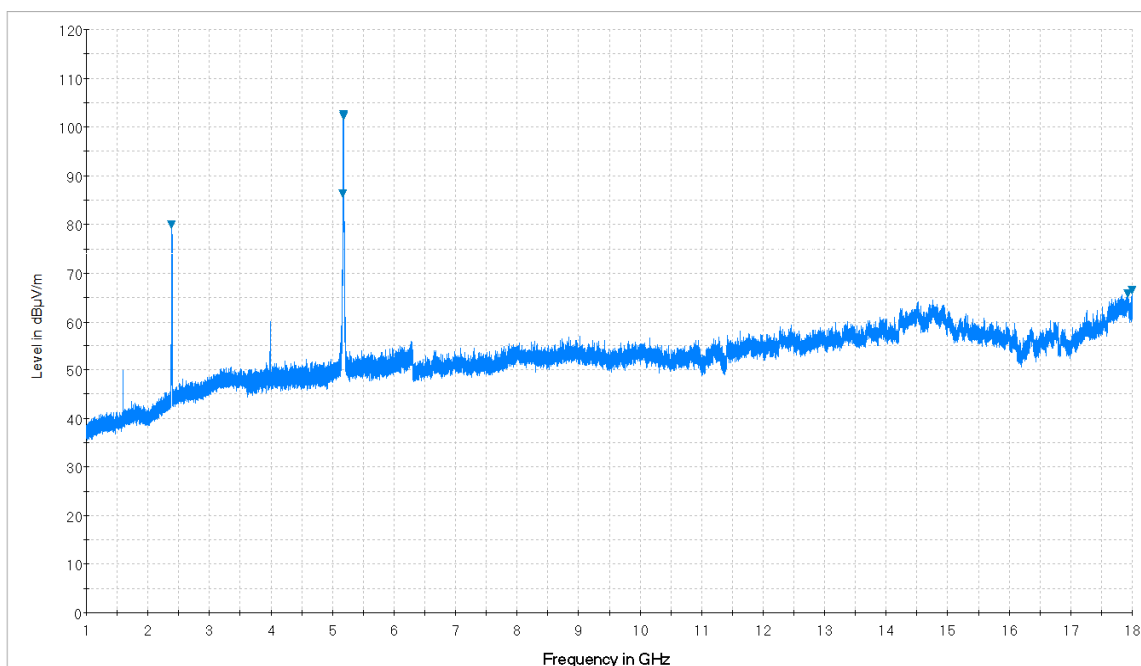
Plot 7-11. Radiated Spurious Plot from 1GHz – 18GHz (Whip Antenna: 14035-4000-01) (Pol. V)
