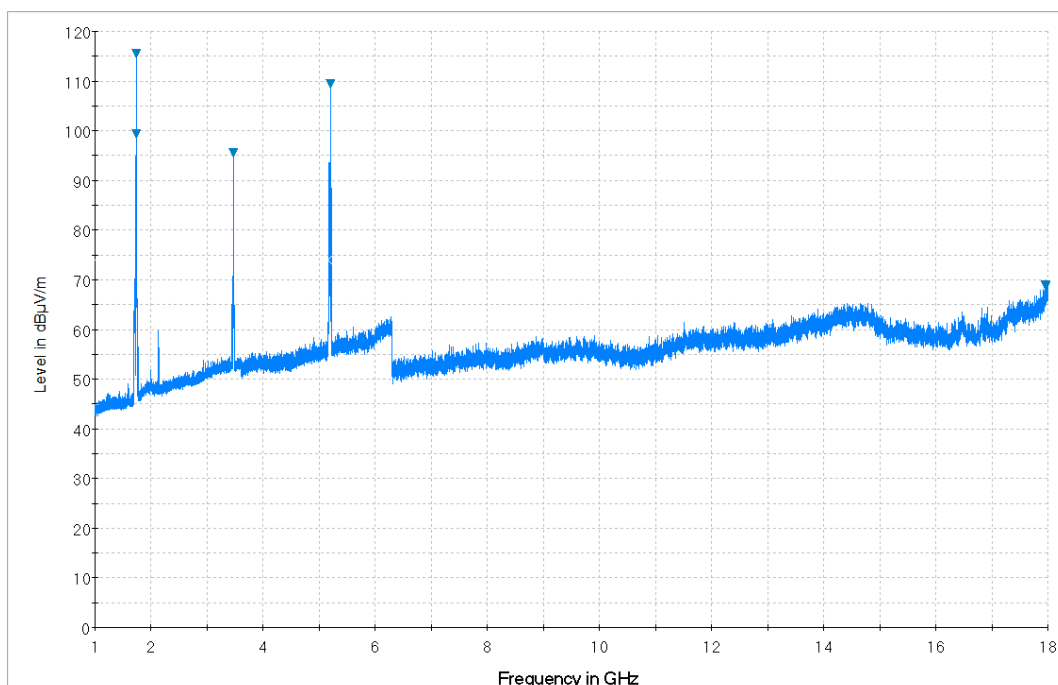
Plot 7-26. Radiated Spurious Plot from 1GHz – 18GHz (Whip Antenna: 14035-4000-01) (Pol. H)
