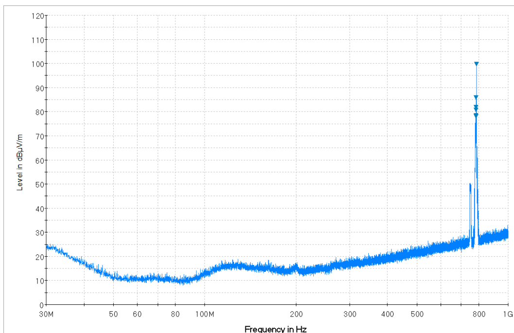
Plot 7-40. Radiated Spurious Plot from 30MHz - 1GHz (Whip Antenna: 14035-4440-02) (Pol. H)
