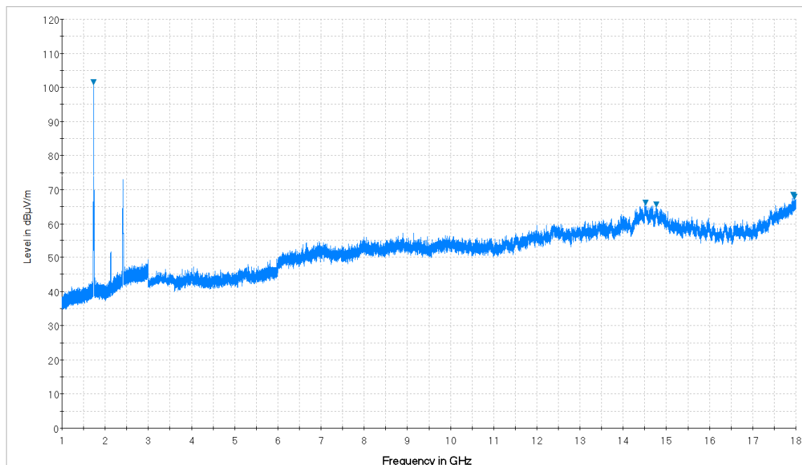
Plot 7-19. Radiated Spurious Plot from 1GHz – 18GHz (Whip Antenna: 14035-4000-01) (Pol. V)
