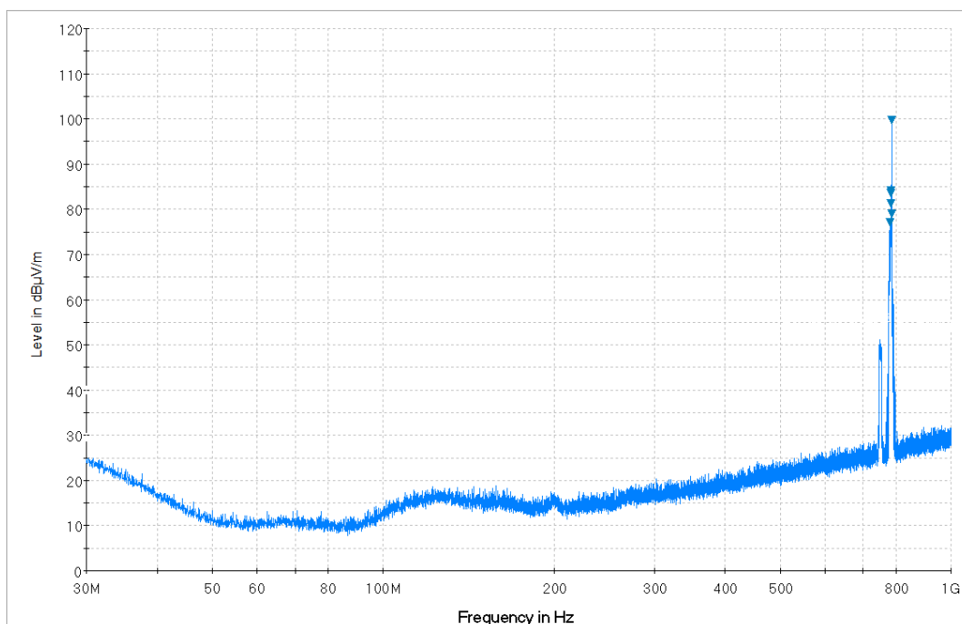
Plot 7-38. Radiated Spurious Plot from 30MHz - 1GHz (Whip Antenna: 14035-4440-01) (Pol. H)
