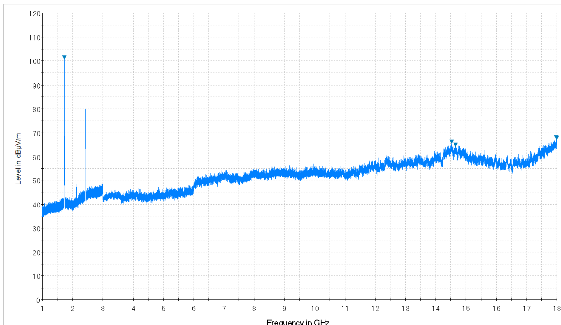
Plot 7-6. Radiated Spurious Plot from 1GHz – 18GHz (Whip Antenna: 14035-4440-01) (Pol. H)
