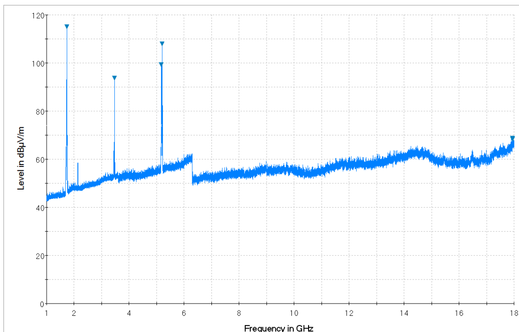
Plot 7-31. Radiated Spurious Plot from 1GHz – 18GHz (Whip Antenna: 14035-4440-01) (Pol. V)
