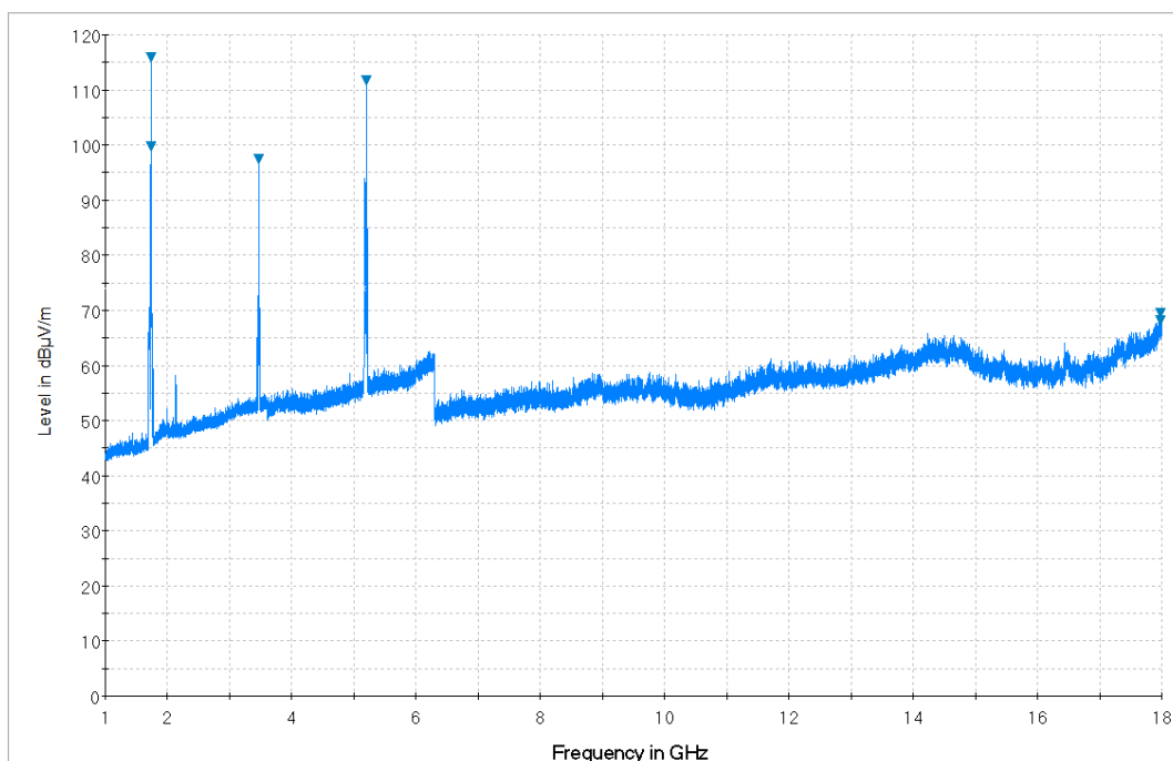
Plot 7-28. Radiated Spurious Plot from 1GHz – 18GHz (Whip Antenna: 14035-4420-01) (Pol. H)
