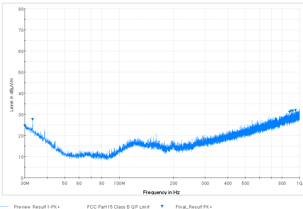
Plot 7-45. Radiated Spurious Plot from 30MHz - 1GHz (Whip Antenna: 14035-4420-01) (Pol. V)
