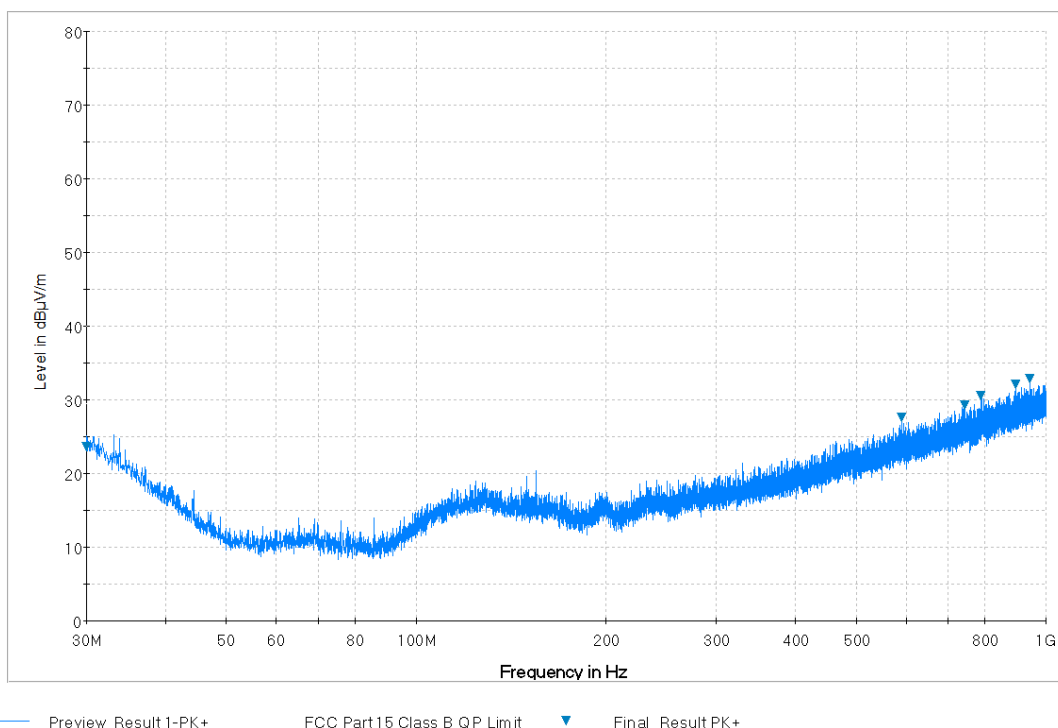
Plot 7-44. Radiated Spurious Plot from 30MHz - 1GHz (Whip Antenna: 14035-4420-01) (Pol. H)
