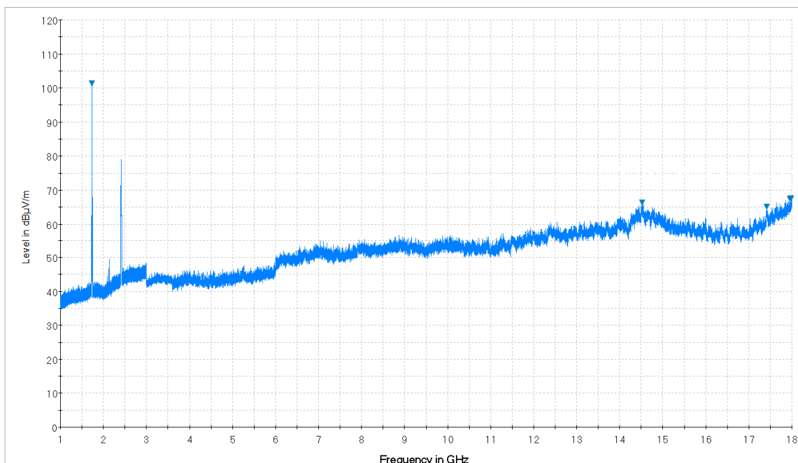
Plot 7-24. Radiated Spurious Plot from 1GHz – 18GHz (Whip Antenna: 14035-4440-02) (Pol. H)
