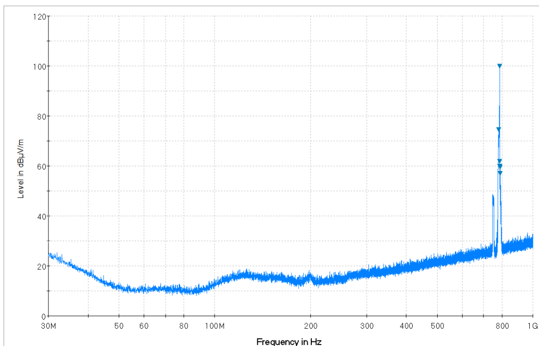
Plot 7-35. Radiated Spurious Plot from 30MHz - 1GHz (Whip Antenna: 14035-4000-01) (Pol. V)
