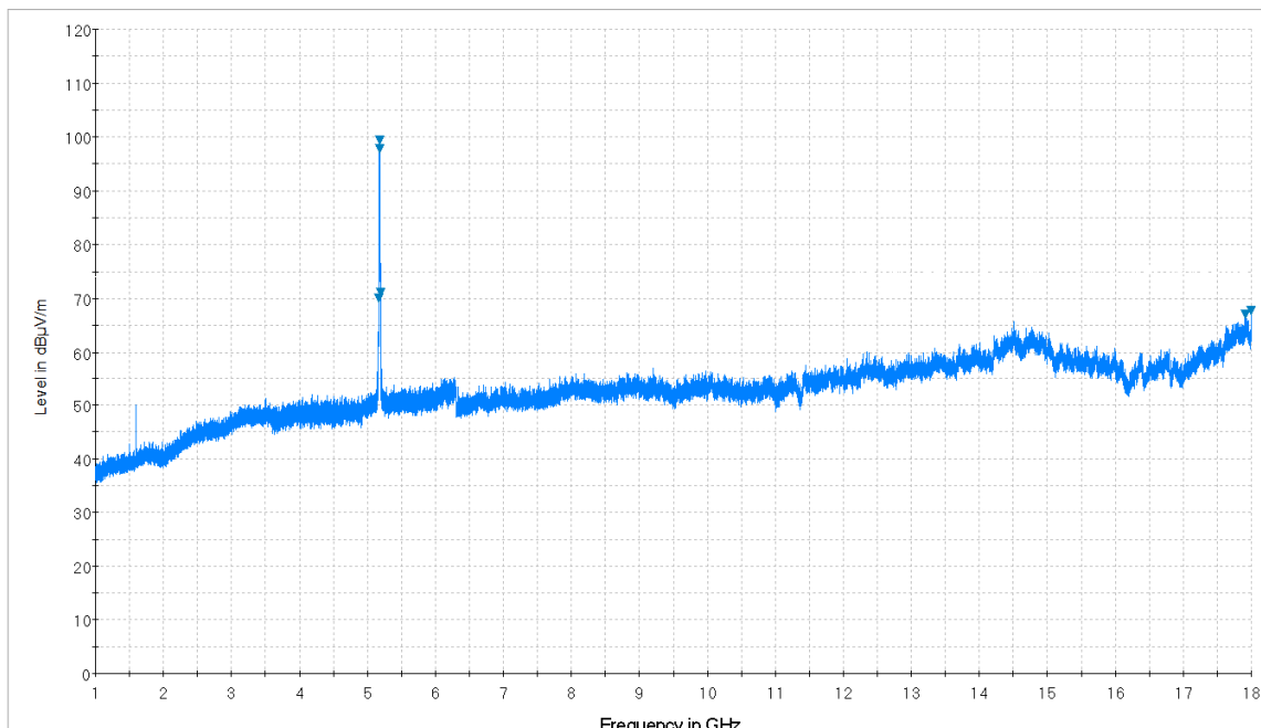
Plot 7-14. Radiated Spurious Plot from 1GHz – 18GHz (Whip Antenna: 14035-4440-01) (Pol. H)
