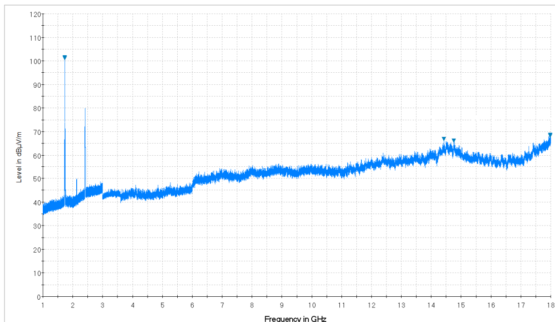
Plot 7-2. Radiated Spurious Plot from 1GHz – 18GHz (Whip Antenna: 14035-4000-01) (Pol. H)
