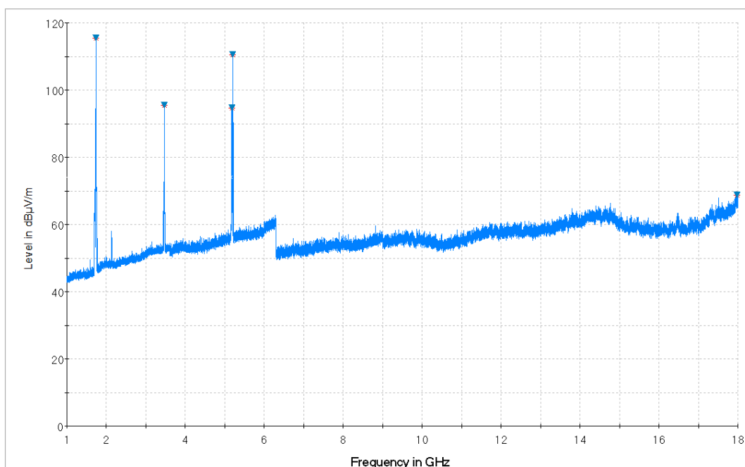
Plot 7-30. Radiated Spurious Plot from 1GHz – 18GHz (Whip Antenna: 14035-4440-01) (Pol. H)
