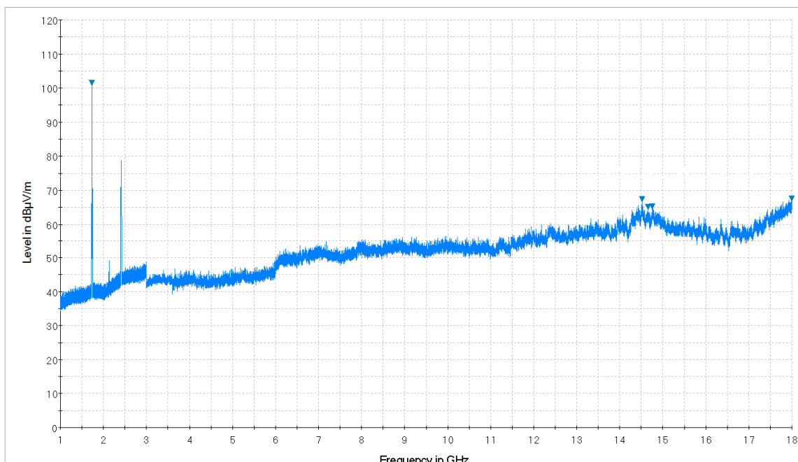
Plot 7-4. Radiated Spurious Plot from 1GHz – 18GHz (Whip Antenna: 14035-4420-01) (Pol. H)
