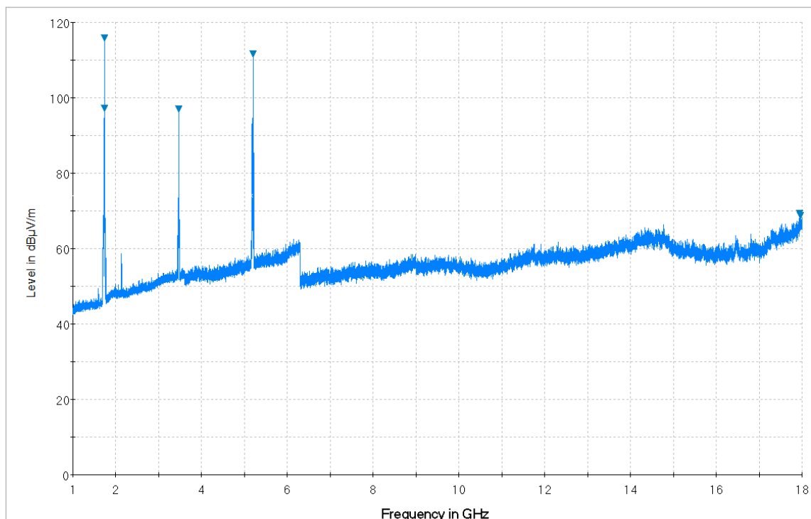
Plot 7-32. Radiated Spurious Plot from 1GHz – 18GHz (Whip Antenna: 14035-4440-02) (Pol. H)
