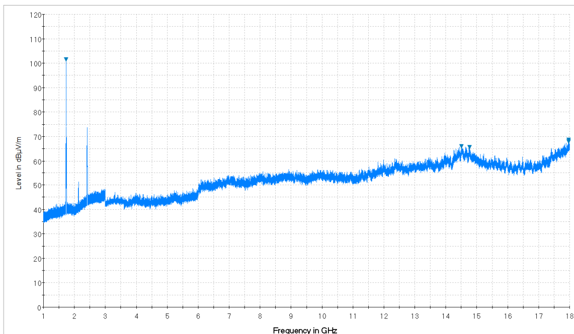
Plot 7-25. Radiated Spurious Plot from 1GHz – 18GHz (Whip Antenna: 14035-4440-02) (Pol. V)
