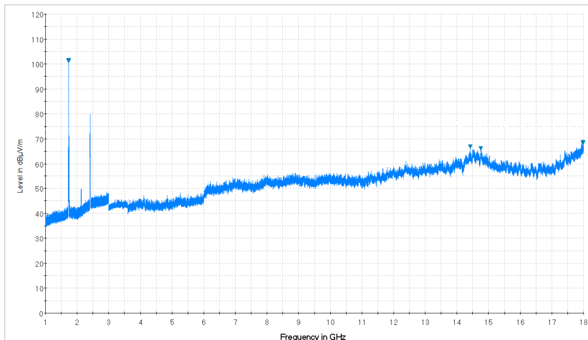
Plot 7-18. Radiated Spurious Plot from 1GHz – 18GHz (Whip Antenna: 14035-4000-01) (Pol. H)
