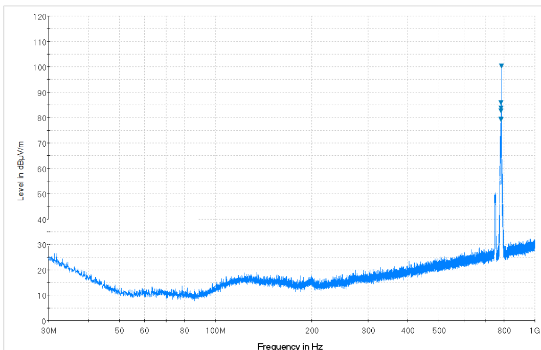
Plot 7-34. Radiated Spurious Plot from 30MHz - 1GHz (Whip Antenna: 14035-4000-01) (Pol. H)
