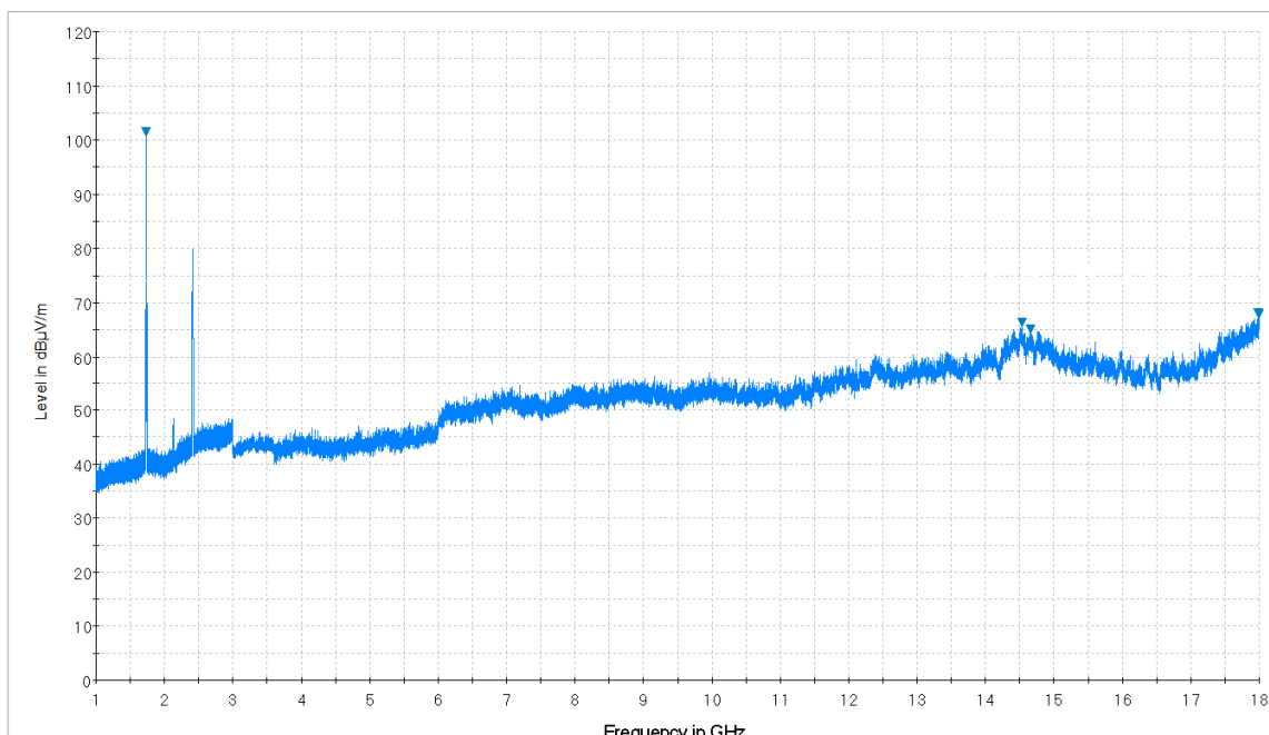
Plot 7-22. Radiated Spurious Plot from 1GHz – 18GHz (Whip Antenna: 14035-4440-01) (Pol. H)
