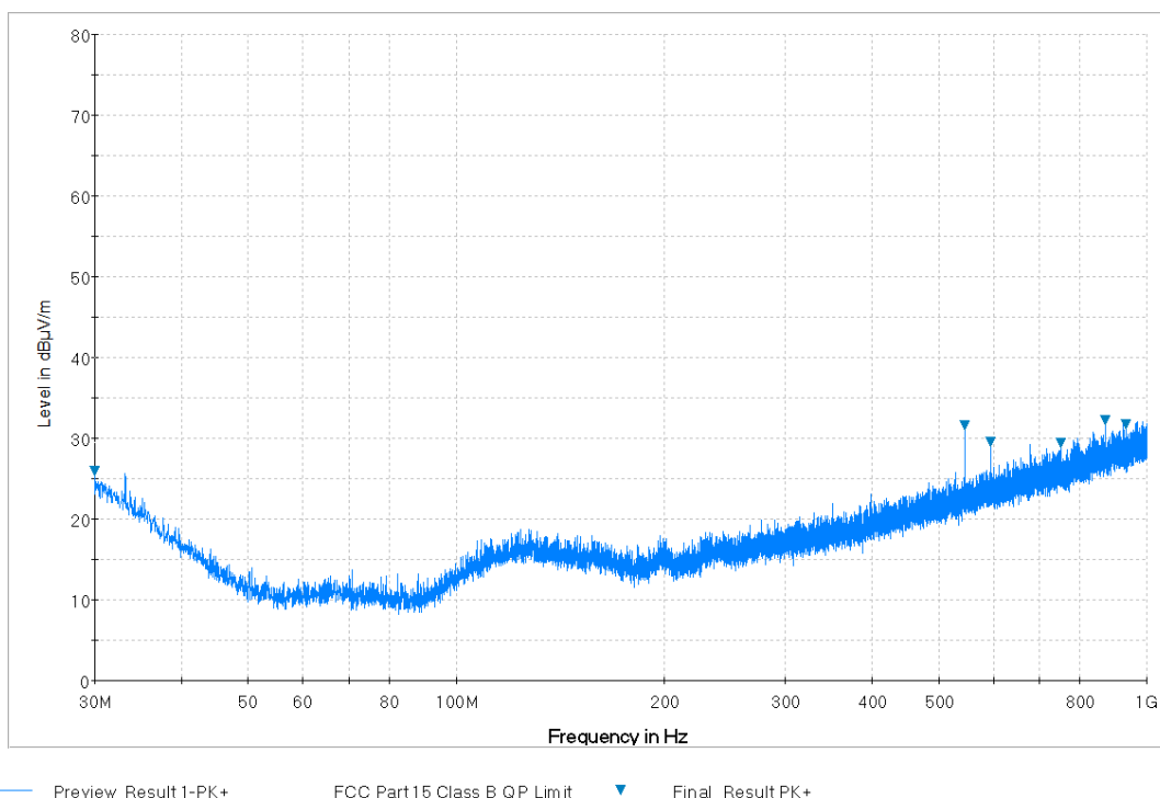
Plot 7-48. Radiated Spurious Plot from 30MHz - 1GHz (Whip Antenna: 14035-4440-02) (Pol. H)
