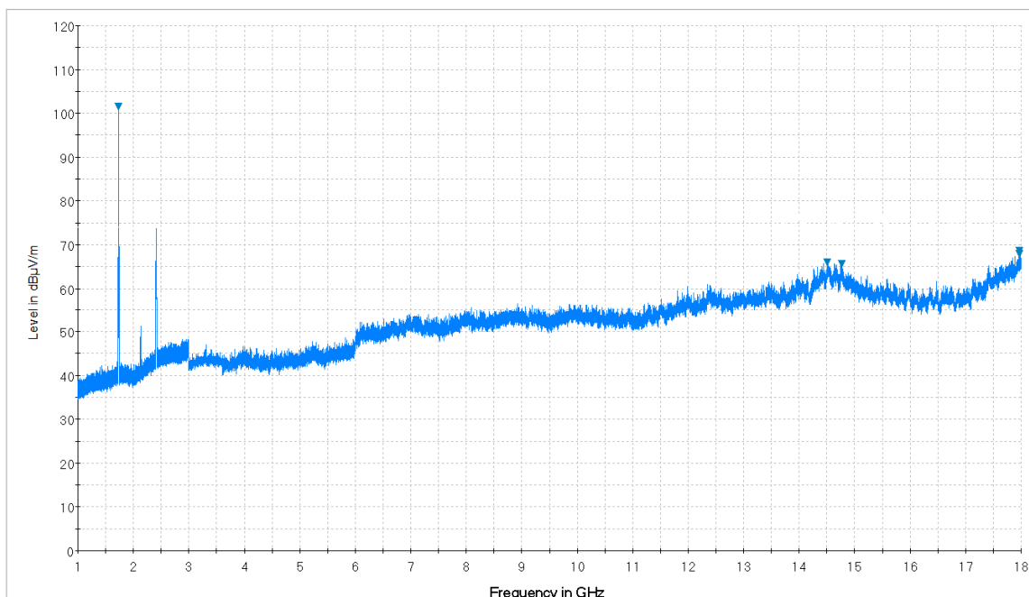
Plot 7-9. Radiated Spurious Plot from 1GHz – 18GHz (Whip Antenna: 14035-4440-02) (Pol. V)
