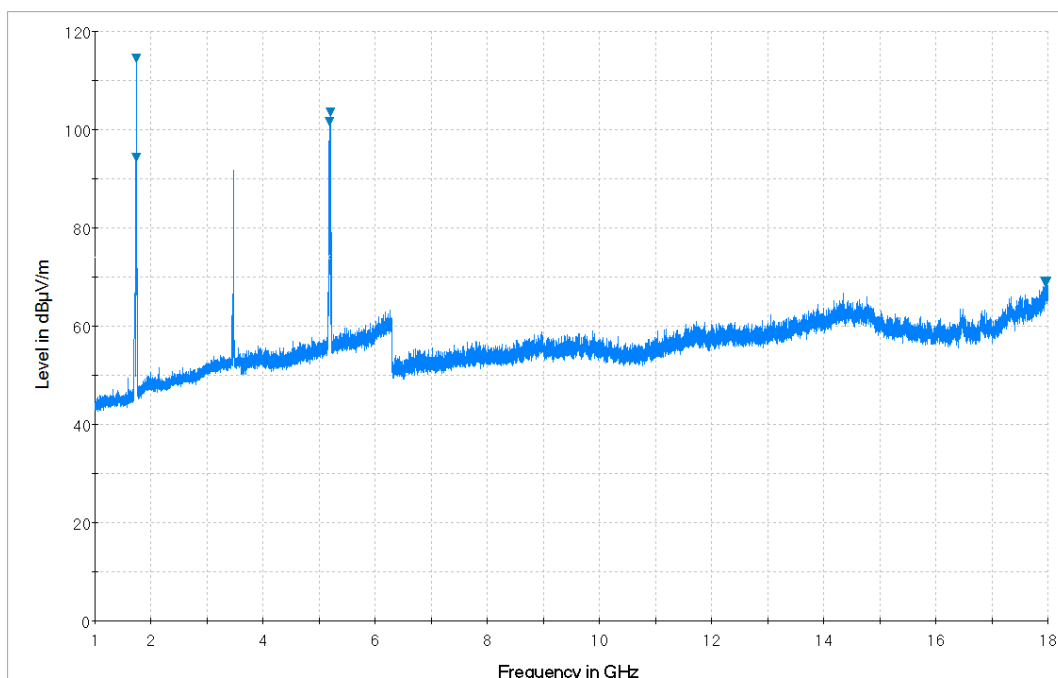
Plot 7-27. Radiated Spurious Plot from 1GHz – 18GHz (Whip Antenna: 14035-4000-01) (Pol. V)
