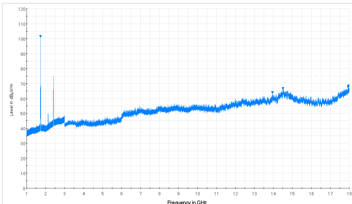
Plot 7-7. Radiated Spurious Plot from 1GHz – 18GHz (Whip Antenna: 14035-4440-01) (Pol. V)
