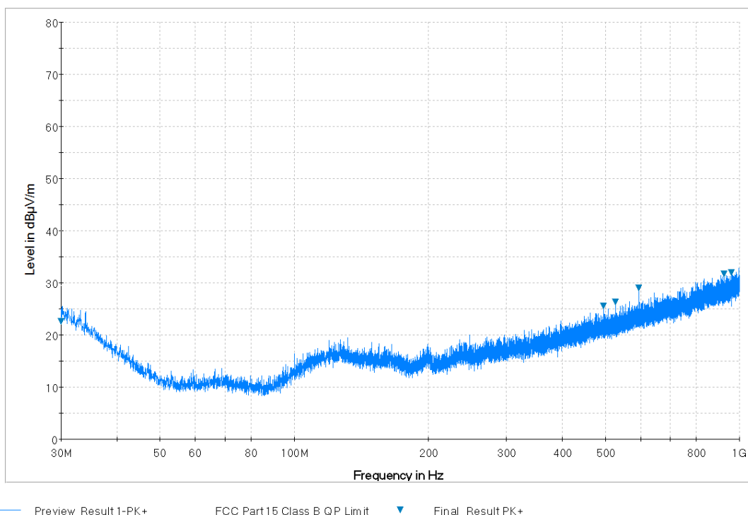
Plot 7-46. Radiated Spurious Plot from 30MHz - 1GHz (Whip Antenna: 14035-4440-01) (Pol. H)
