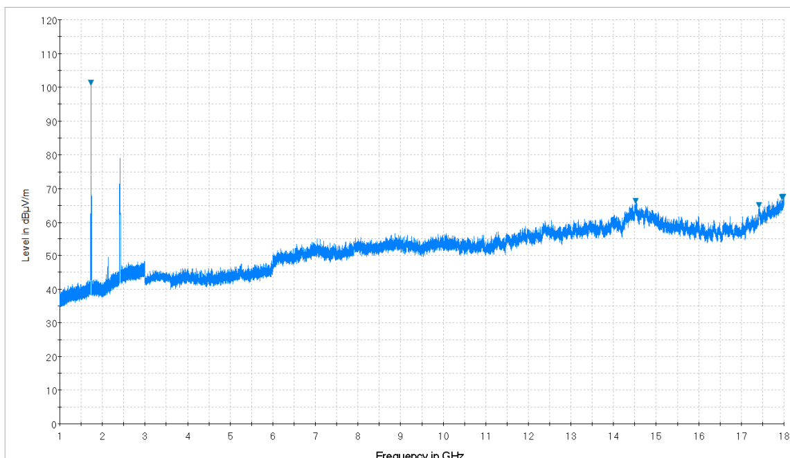
Plot 7-8. Radiated Spurious Plot from 1GHz – 18GHz (Whip Antenna: 14035-4440-02) (Pol. H)
