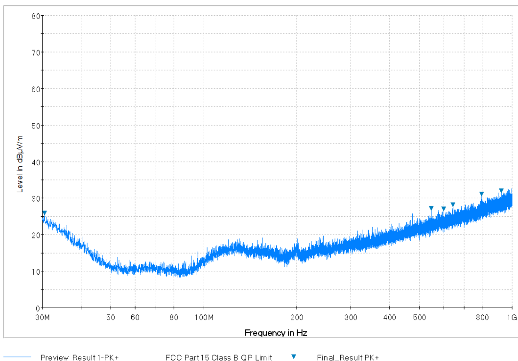
Plot 7-42. Radiated Spurious Plot from 30MHz - 1GHz (Whip Antenna: 14035-4000-01) (Pol. H)
