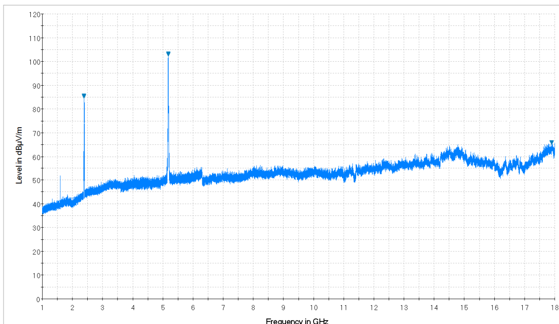
Plot 7-13. Radiated Spurious Plot from 1GHz – 18GHz (Whip Antenna: 14035-4420-01) (Pol. V)
