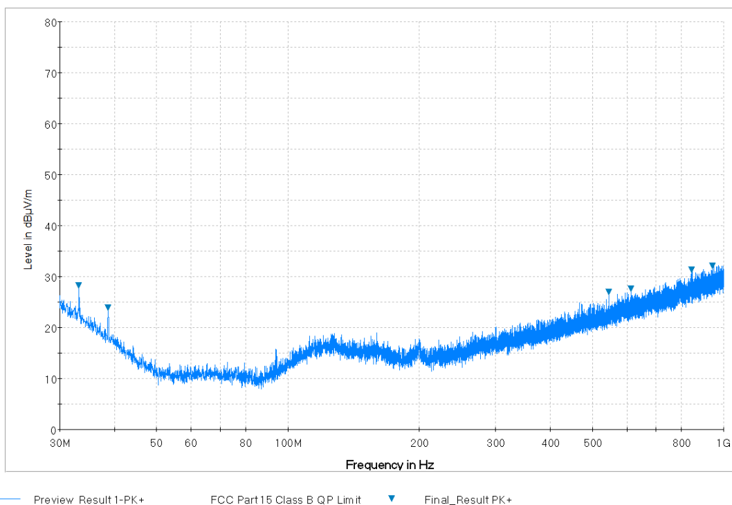
Plot 7-43. Radiated Spurious Plot from 30MHz - 1GHz (Whip Antenna: 14035-4000-01) (Pol. V)
