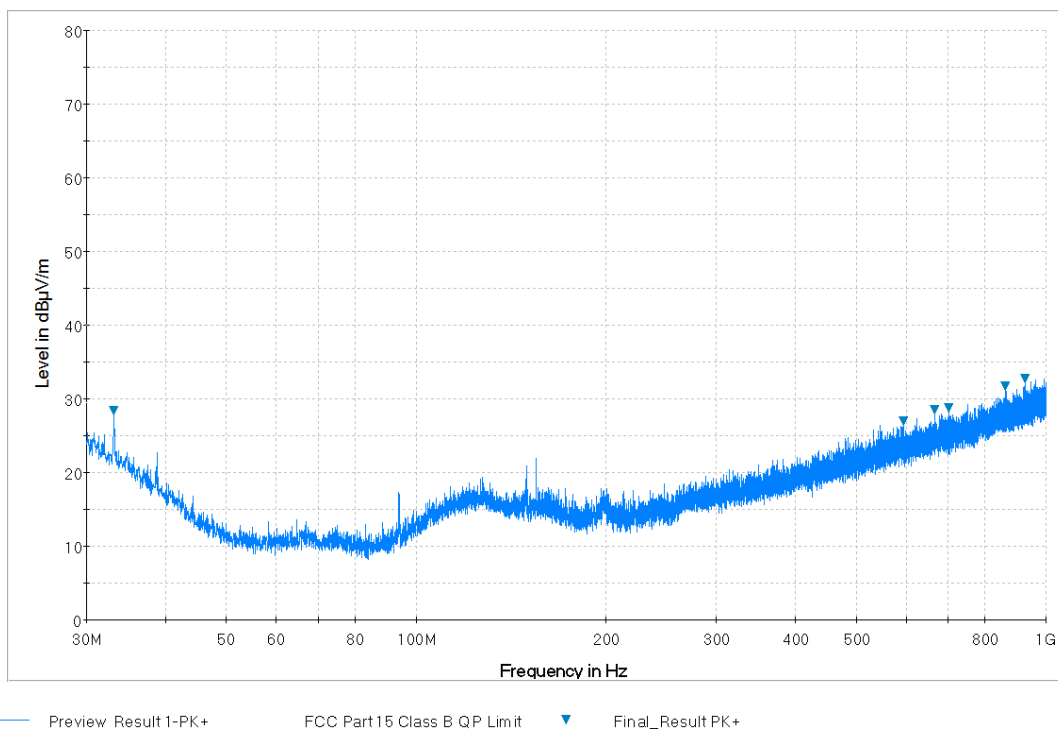
Plot 7-47. Radiated Spurious Plot from 30MHz - 1GHz (Whip Antenna: 14035-4440-01) (Pol. V)
