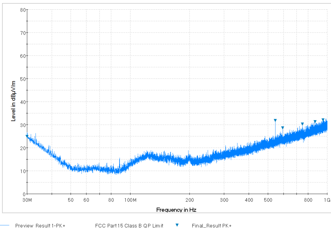
Plot 7-49. Radiated Spurious Plot from 30MHz - 1GHz (Whip Antenna: 14035-4440-02) (Pol. V)
