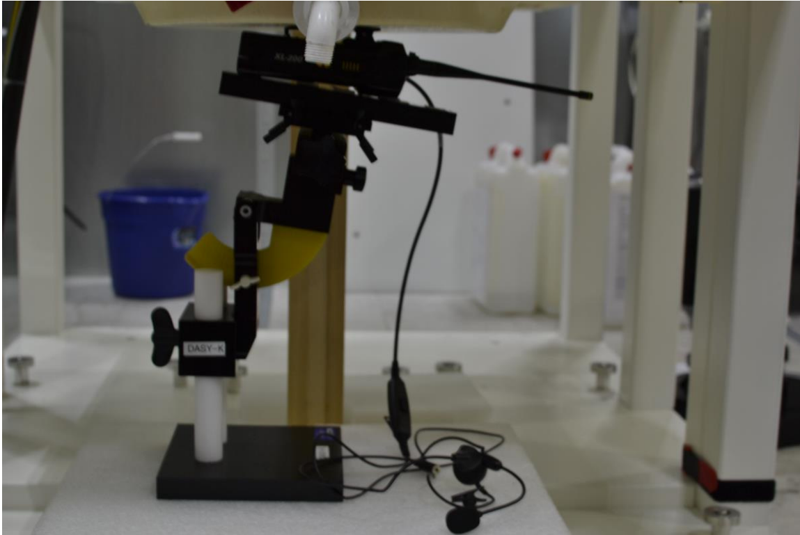
SAR Test Setup Photo 5 – Back Side at 0.0 cm with BW Grouping 1, Audio Accessory III
