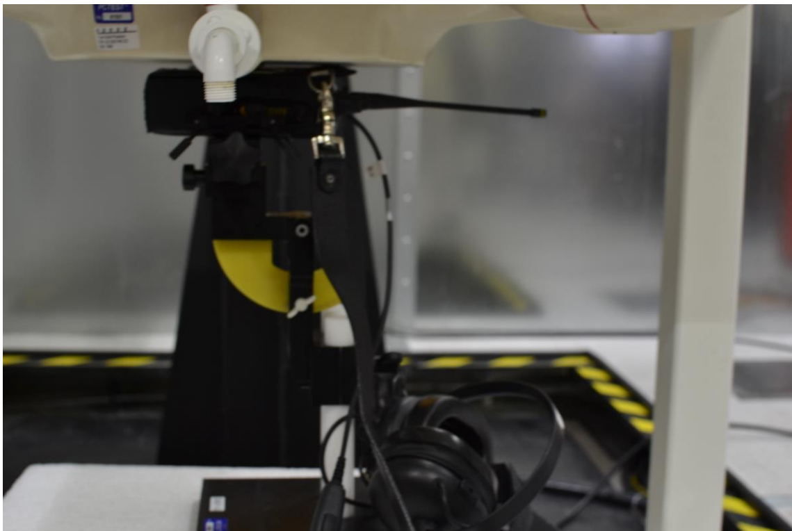
SAR Test Setup Photo 8 – Back Side at 0.0 cm with BW Grouping 2, Audio Accessory I
