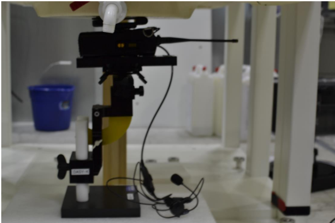
SAR Test Setup Photo 14 – Back Side at 0.0 cm with BW Grouping 3, Audio Accessory IV
