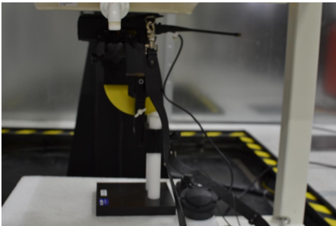
SAR Test Setup Photo 9 – Back Side at 0.0 cm with BW Grouping 2, Audio Accessory II
