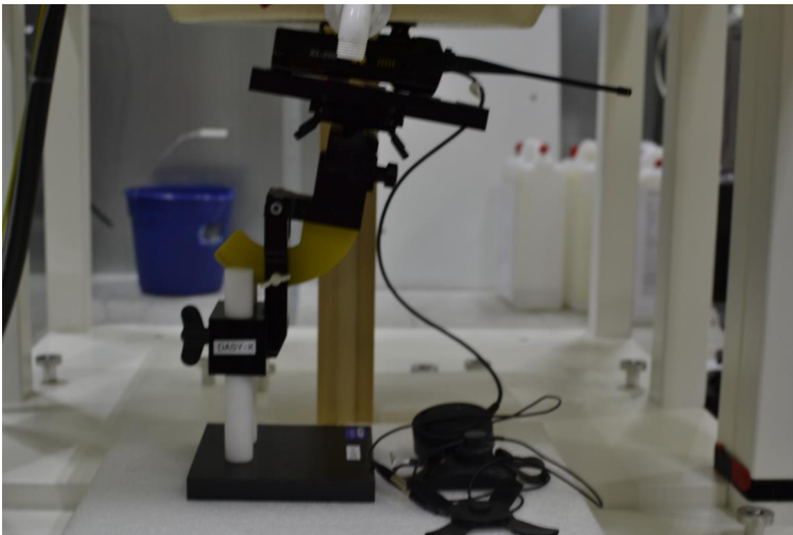
SAR Test Setup Photo 4 – Back Side at 0.0 cm with BW Grouping 1, Audio Accessory II
