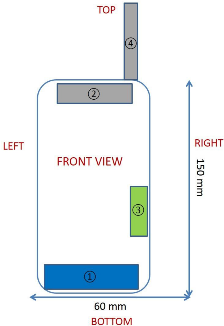
Figure F-1 DUT Antenna Locations
