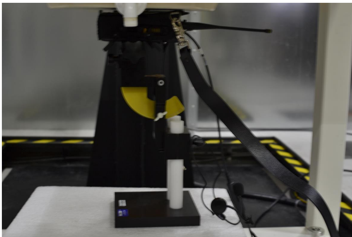
SAR Test Setup Photo 10 – Back Side at 0.0 cm with BW Grouping 2, Audio Accessory IV
