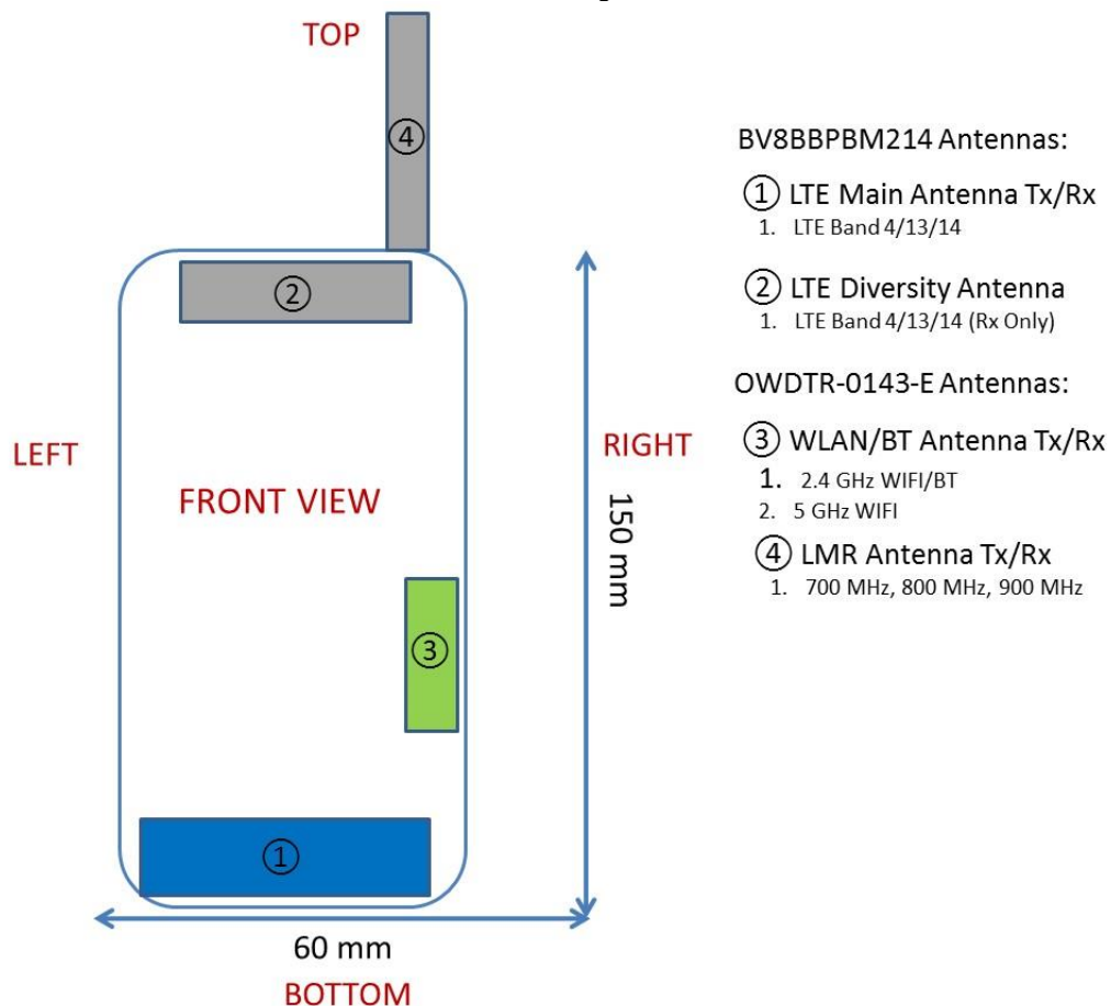
Figure F-1 DUT Antenna Locations
