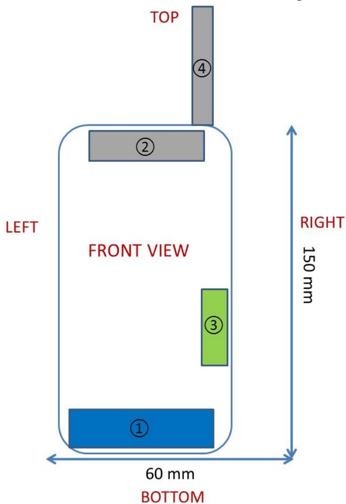
Figure F-1 DUT Antenna Locations
