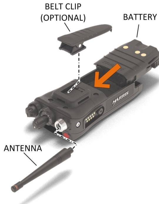
Figure 4-1: Radio Assembly
