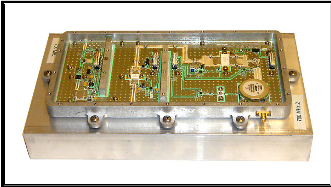
Photograph 18: 700 MHz Cell Site HPA RF Assembly – Cover Removed
