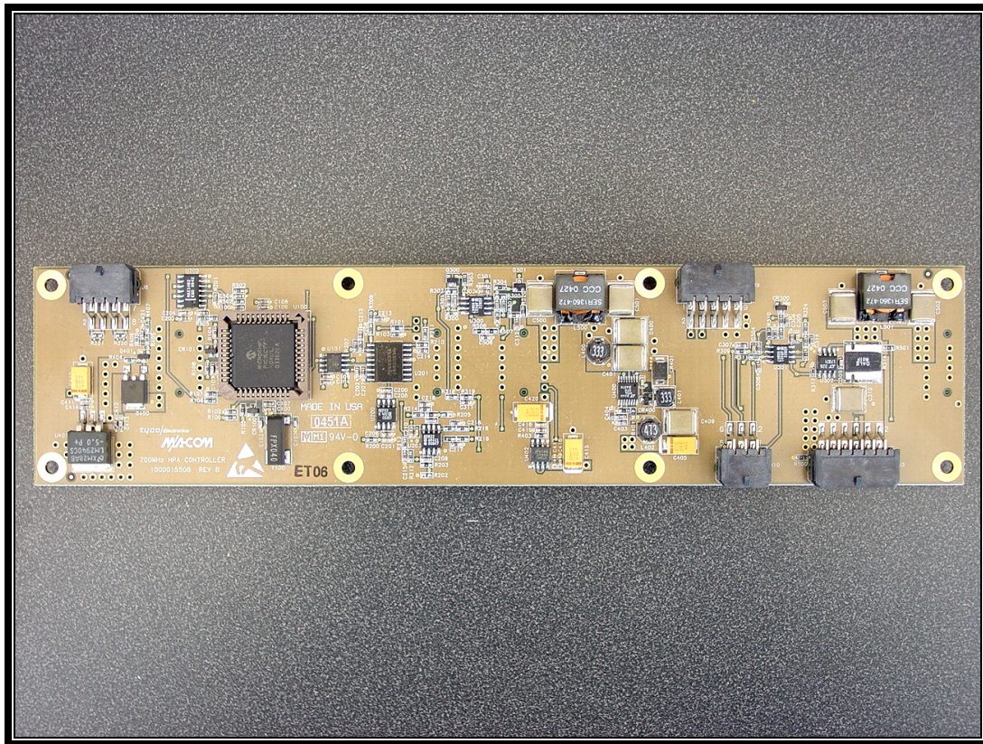
Photograph 19: HPA Controller – Power Distribution Board Front
