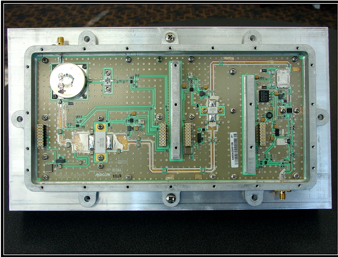
Photograph 21: Circuit Board
