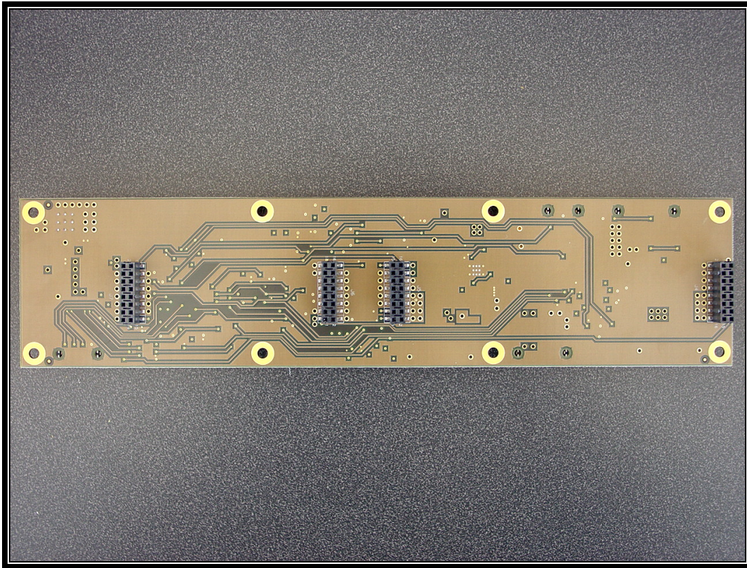
Photograph 20: HPA Controller – Power Distribution Board Back
