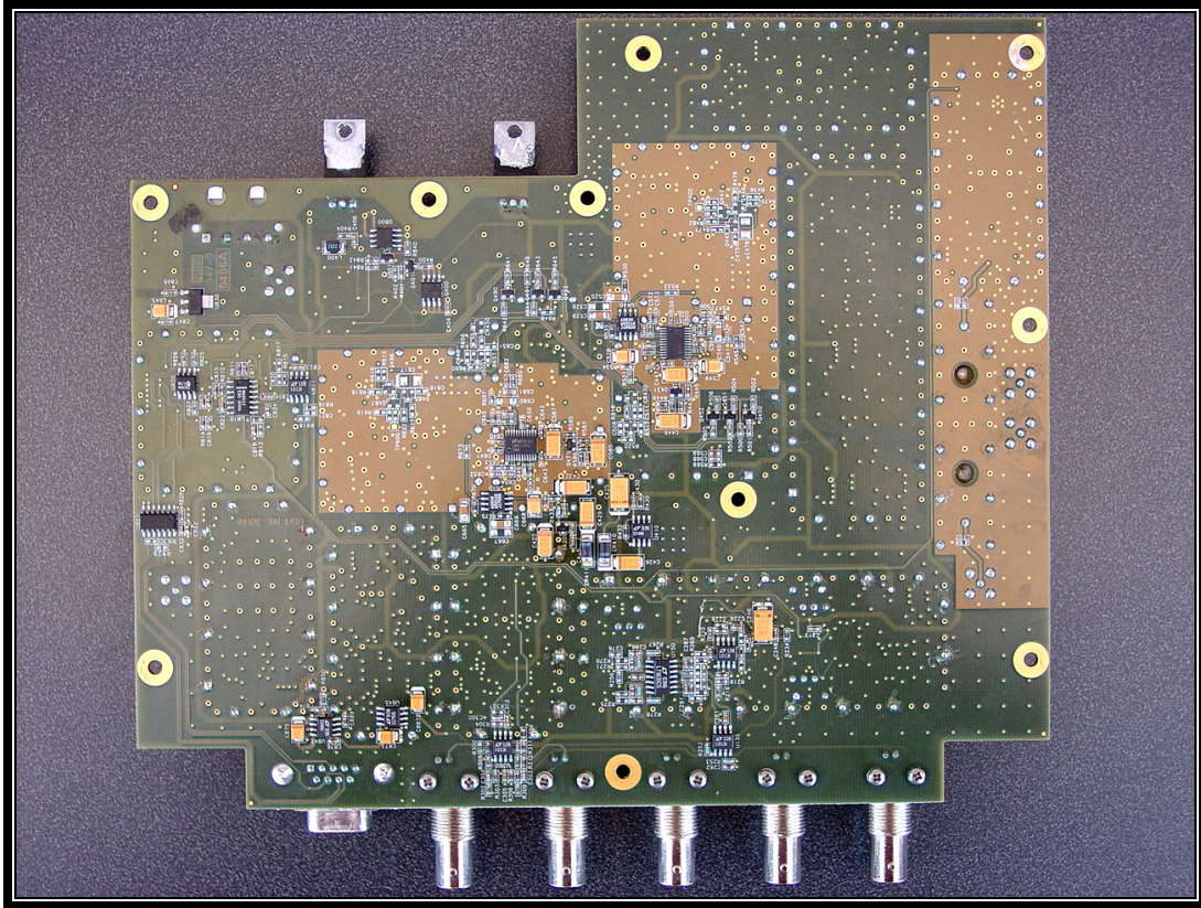
Photograph 27: BSX Board Back
