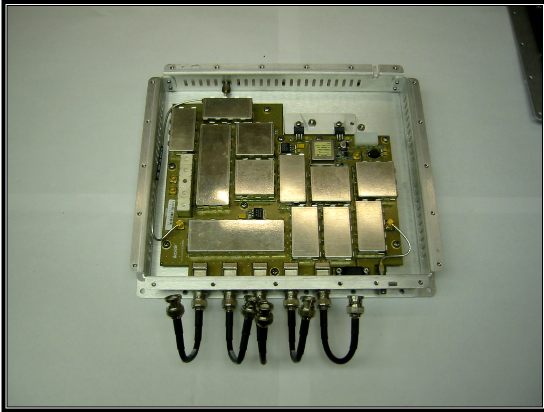
Photograph 23: DCX Enclosure Middle Cover Removed
