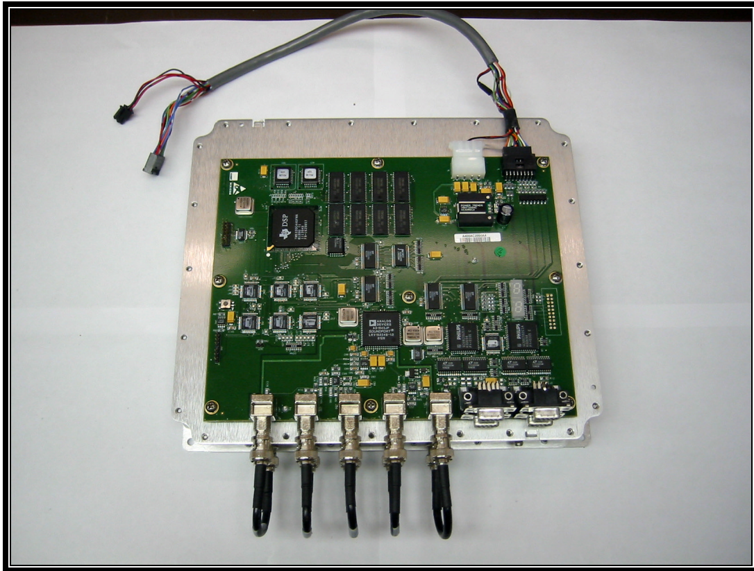
Photograph 22: DCX Enclosure Top Cover Removed
