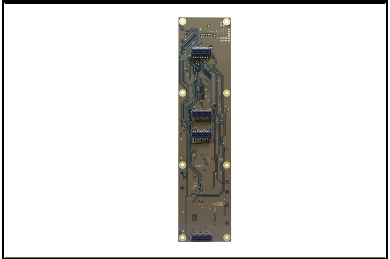
Photograph 27: HPA Controller PCB Bottom
