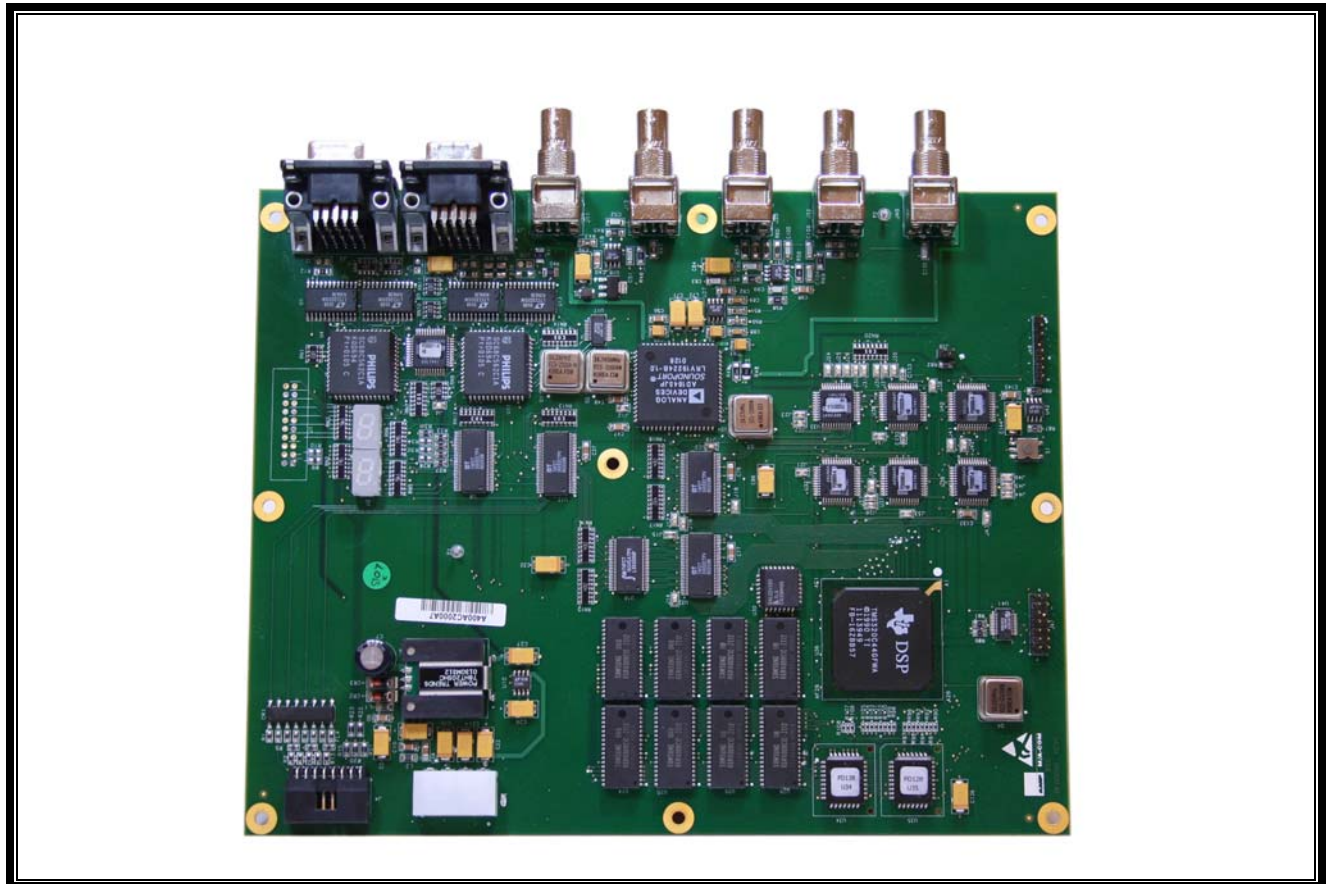
Photograph 16: BSC PCB Top
