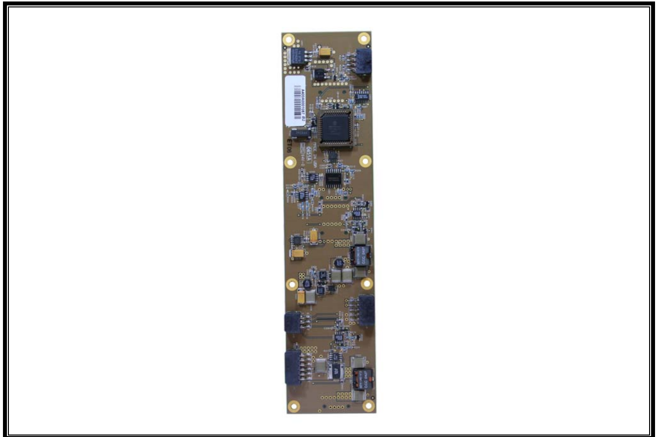
Photograph 26: HPA Controller PCB Top
