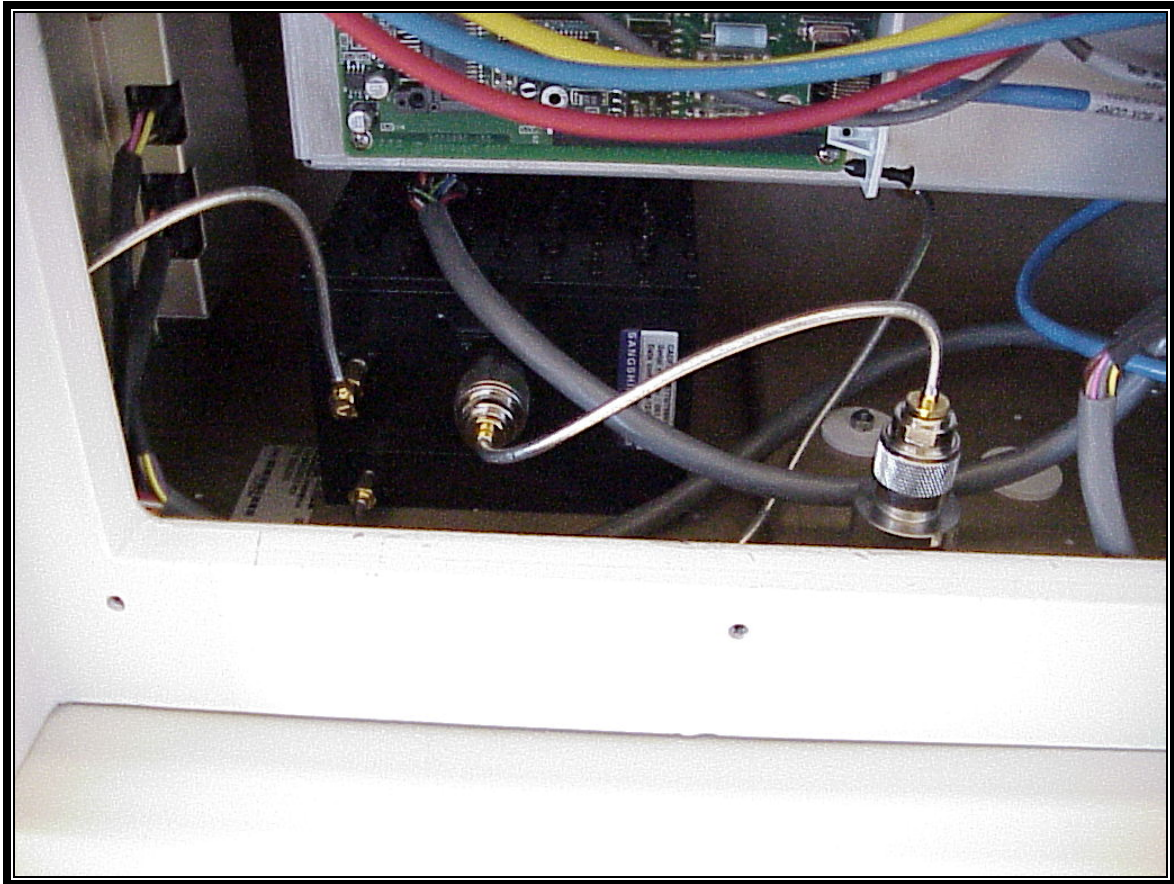
Photograph 11: Cell Site Interior – Configured for One Antenna
