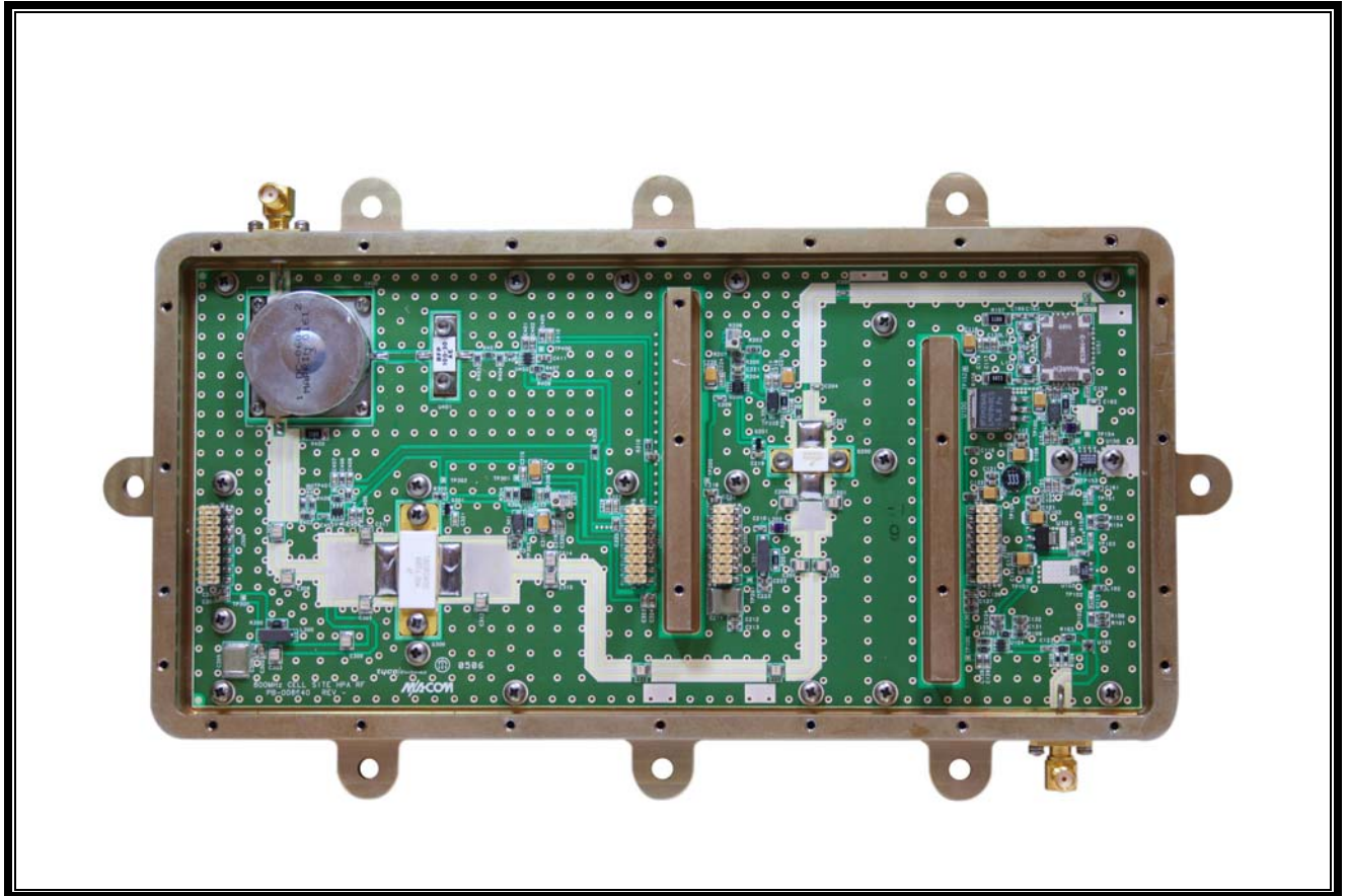
Photograph 28: HPA without RF Cover
