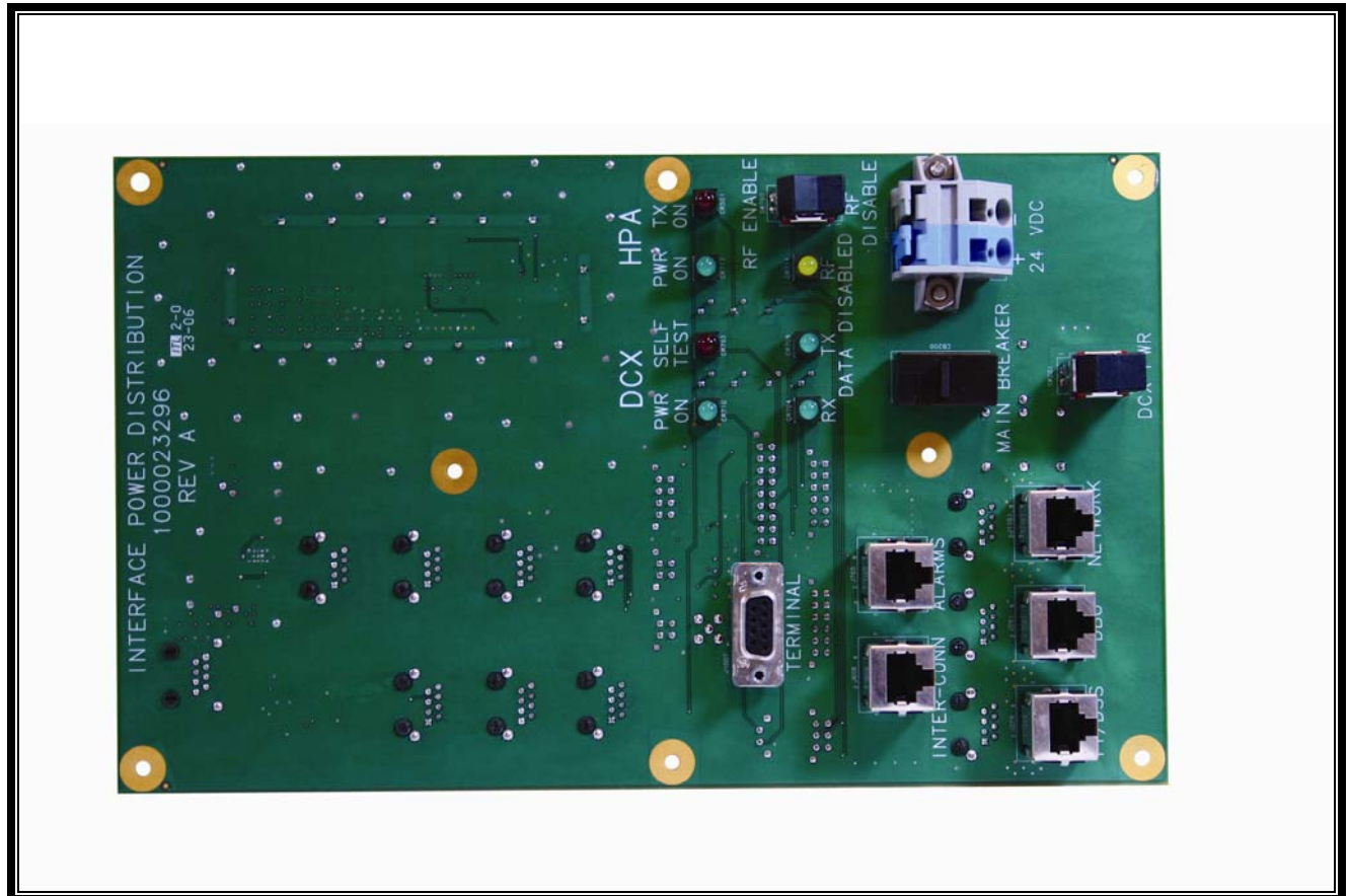
Photograph 21: CIBI PCB Top
