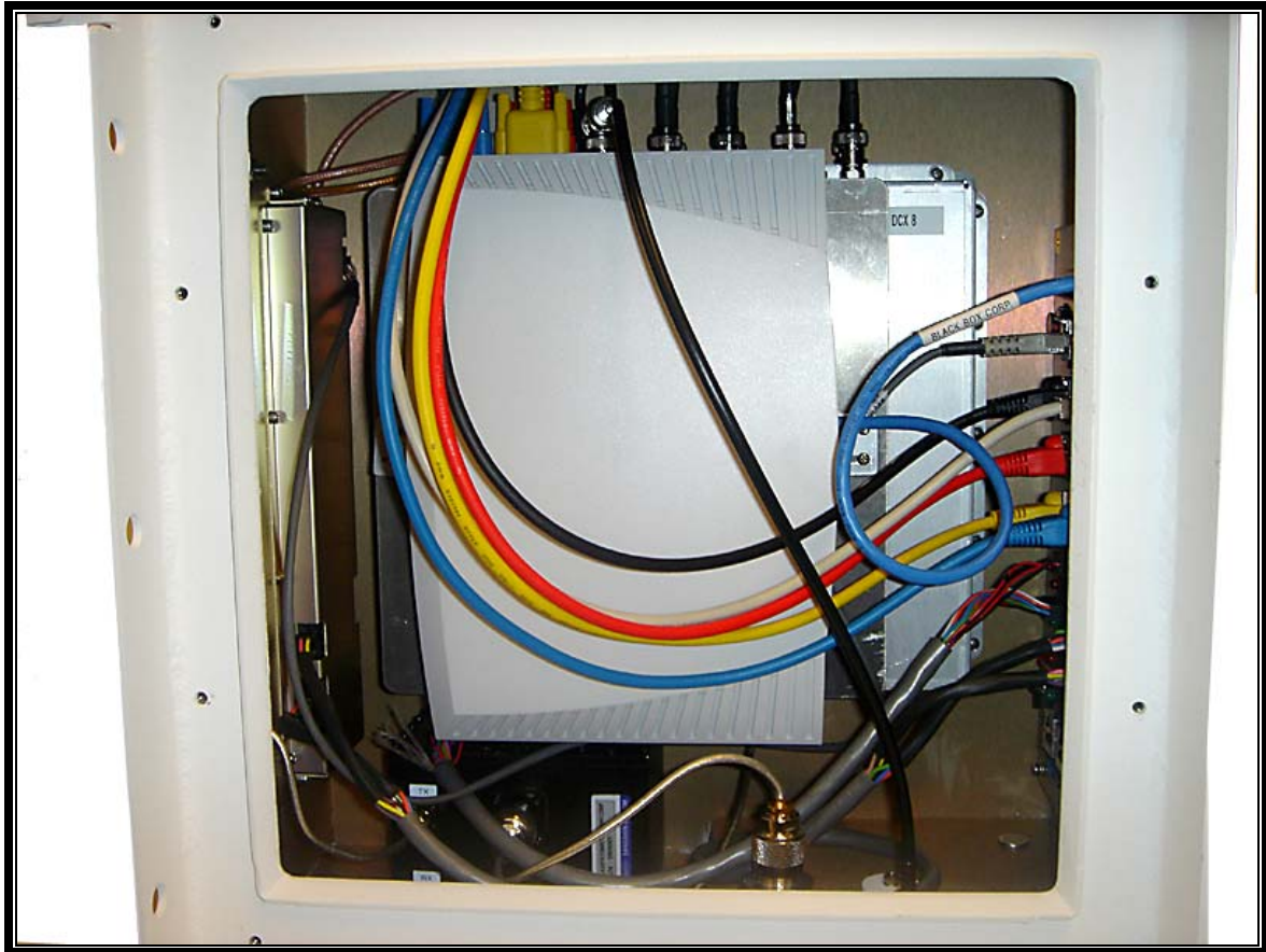
Photograph 9: Cell Site Interior – Side View
