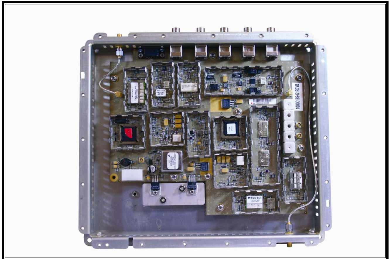
Photograph 18: BSX in DCX Chassis
