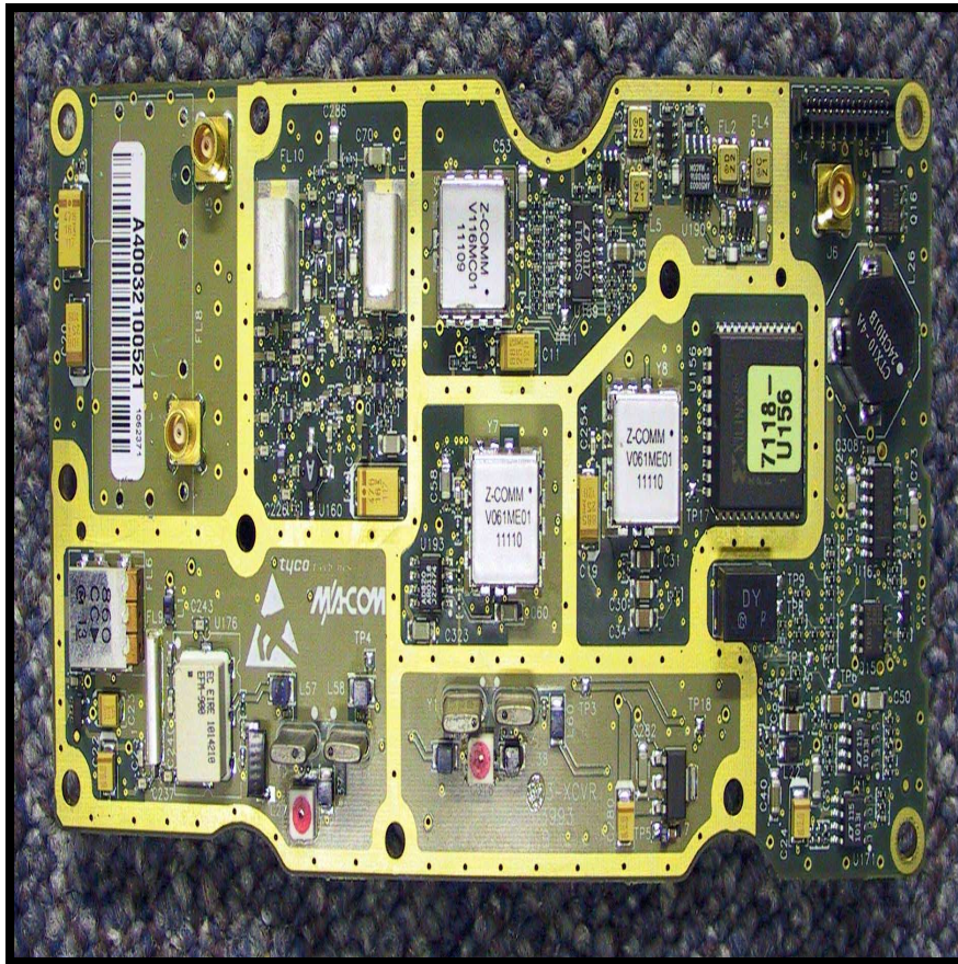
Fi Figure 4 FD Bottom View #2
