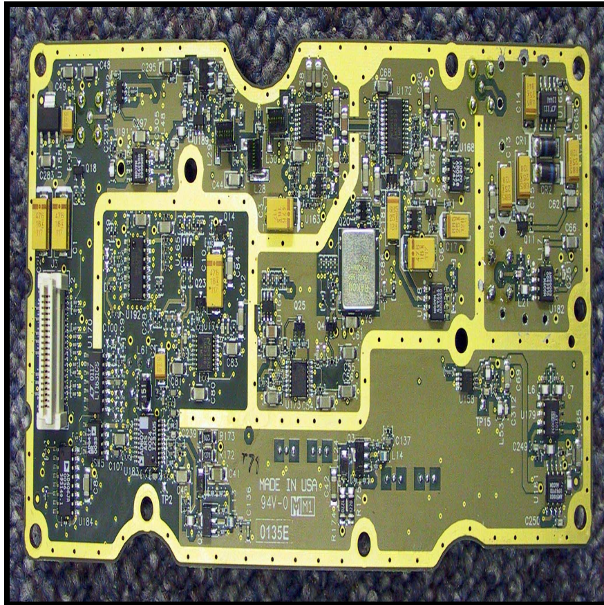
Figure 1 FD Top View#1
