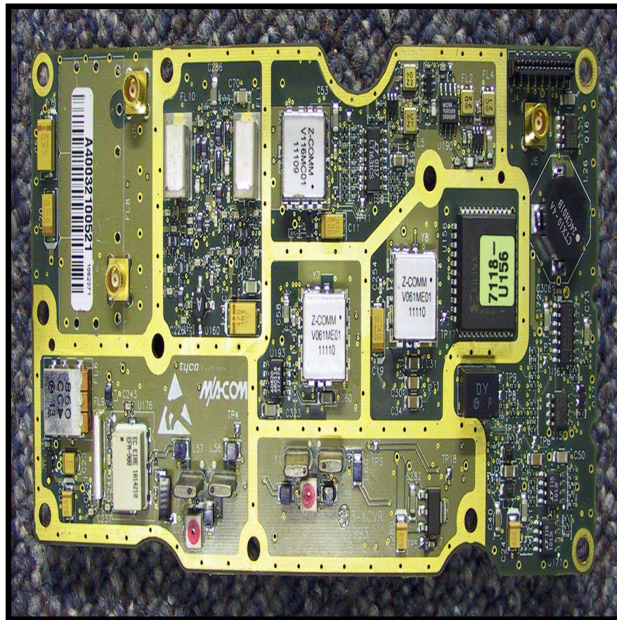
Figure 3 FD Bottom View #1
