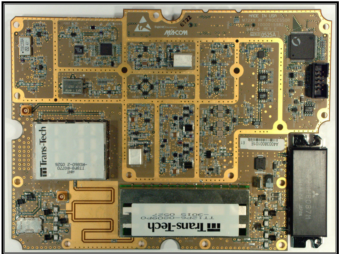
PHOTOGRAPH 8: RF BOARD TOP VIEW
