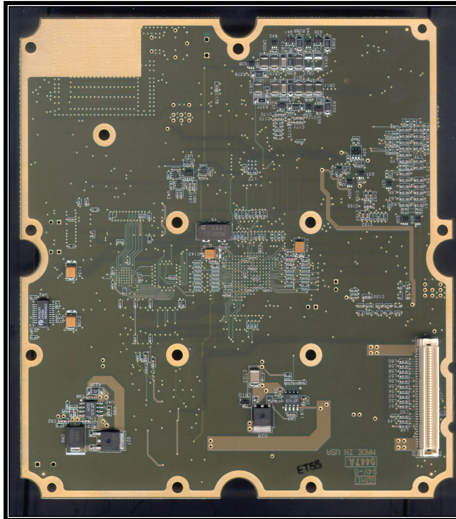
PHOTOGRAPH 11: PK BOARD BOTTOM VIEW
