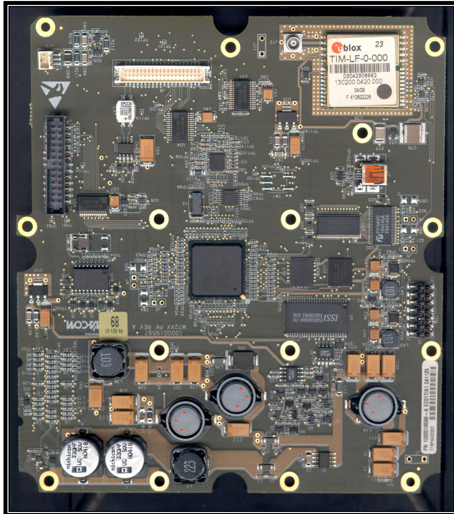
PHOTOGRAPH 10: PK BOARD TOP VIEW
