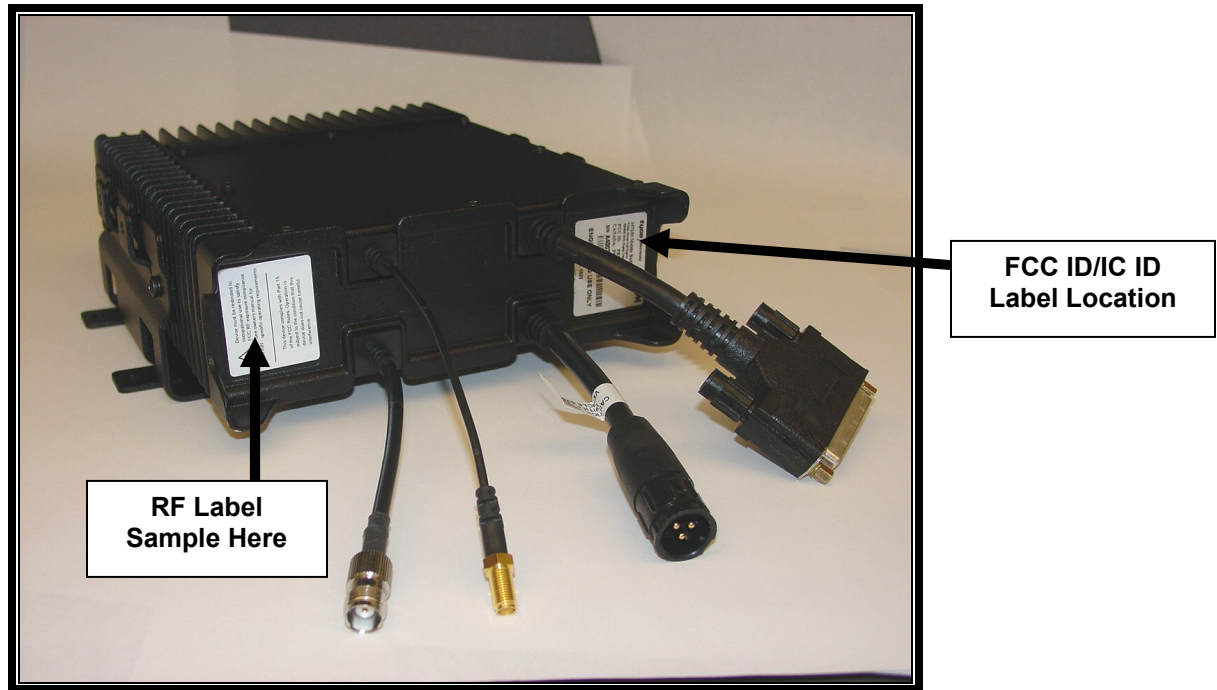
PHOTOGRAPH 3: ID AND RF LABEL LOCATIONS ON REAR OF UNIT
