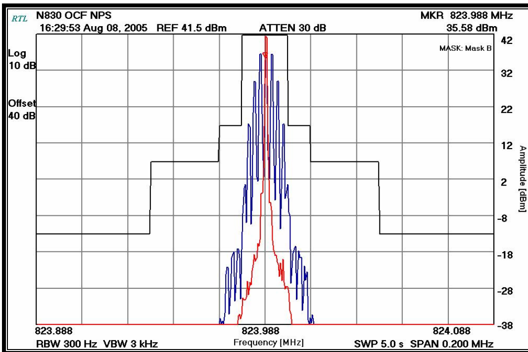
PLOT 9-3: OCCUPIED BANDWIDTH – 823.9875 MHz; OCF; NPSPAC (MASK B)
