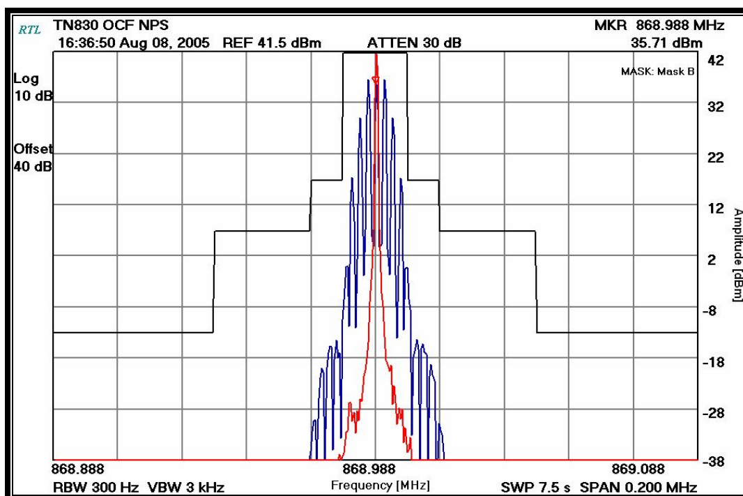
PLOT 9-7: OCCUPIED BANDWIDTH – 868.9875 MHz; OCF; NPSPAC; (MASK B)
