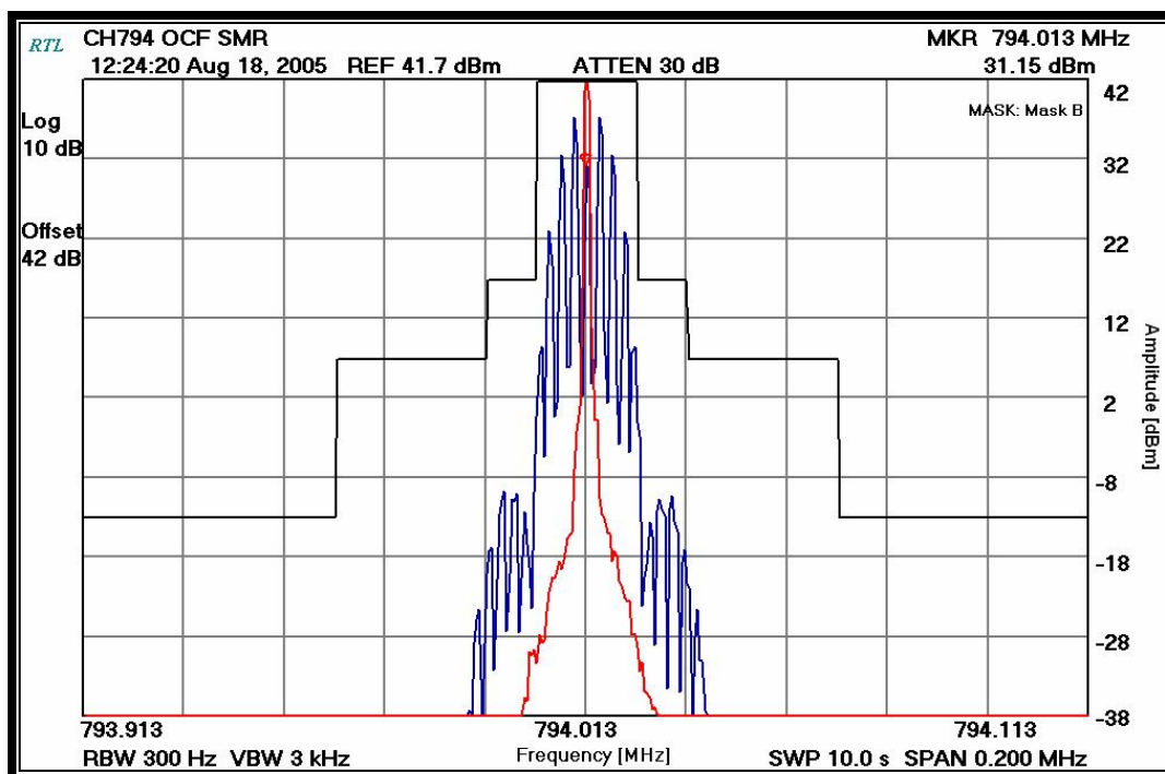
PLOT 9-9: OCCUPIED BANDWIDTH – 794.0125 MHz; OCF; (MASK B)
