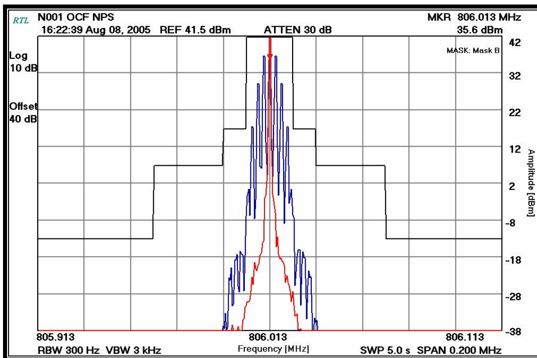
PLOT 9-1: OCCUPIED BANDWIDTH – 806.0125 MHz; OCF; NPSPAC (MASK B)
