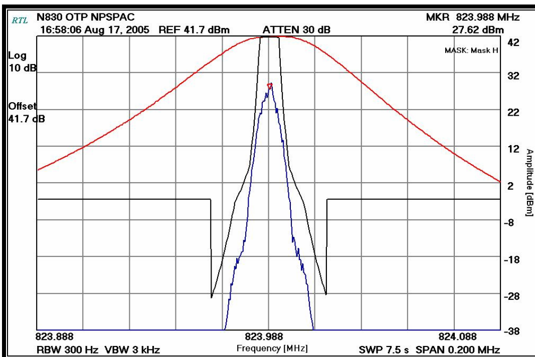
PLOT 9-15: OCCUPIED BANDWIDTH – 823.9875 MHz; OTP; NPSPAC; (MASK H)
