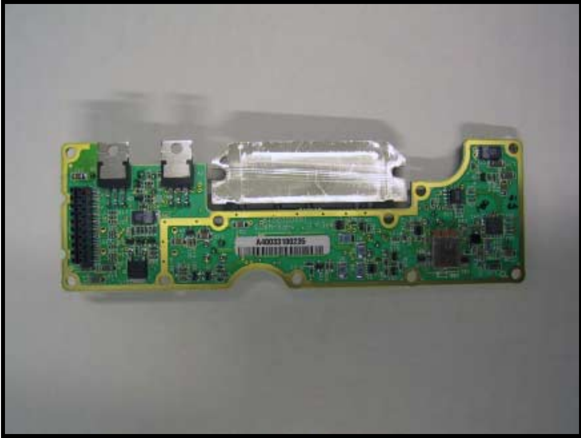
Figure 9 HPA Board Bottom View
