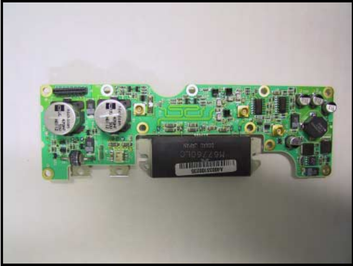
Figure 10 HPA Board View Top View
