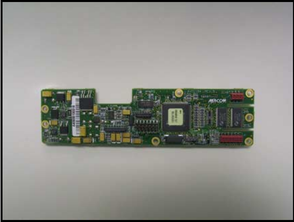
Figure 15 CH Board Top View
