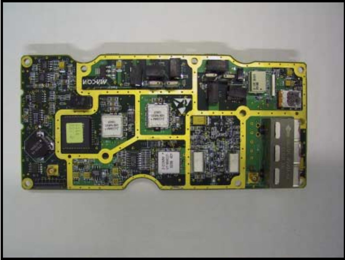
Figure 12 XCVR Board Top View
