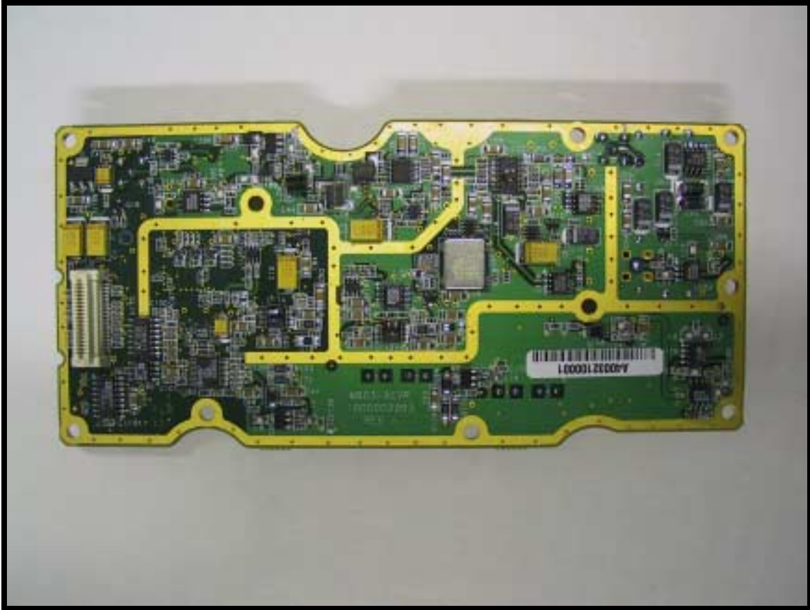
Figure 11 XCVR Board Bottom View
