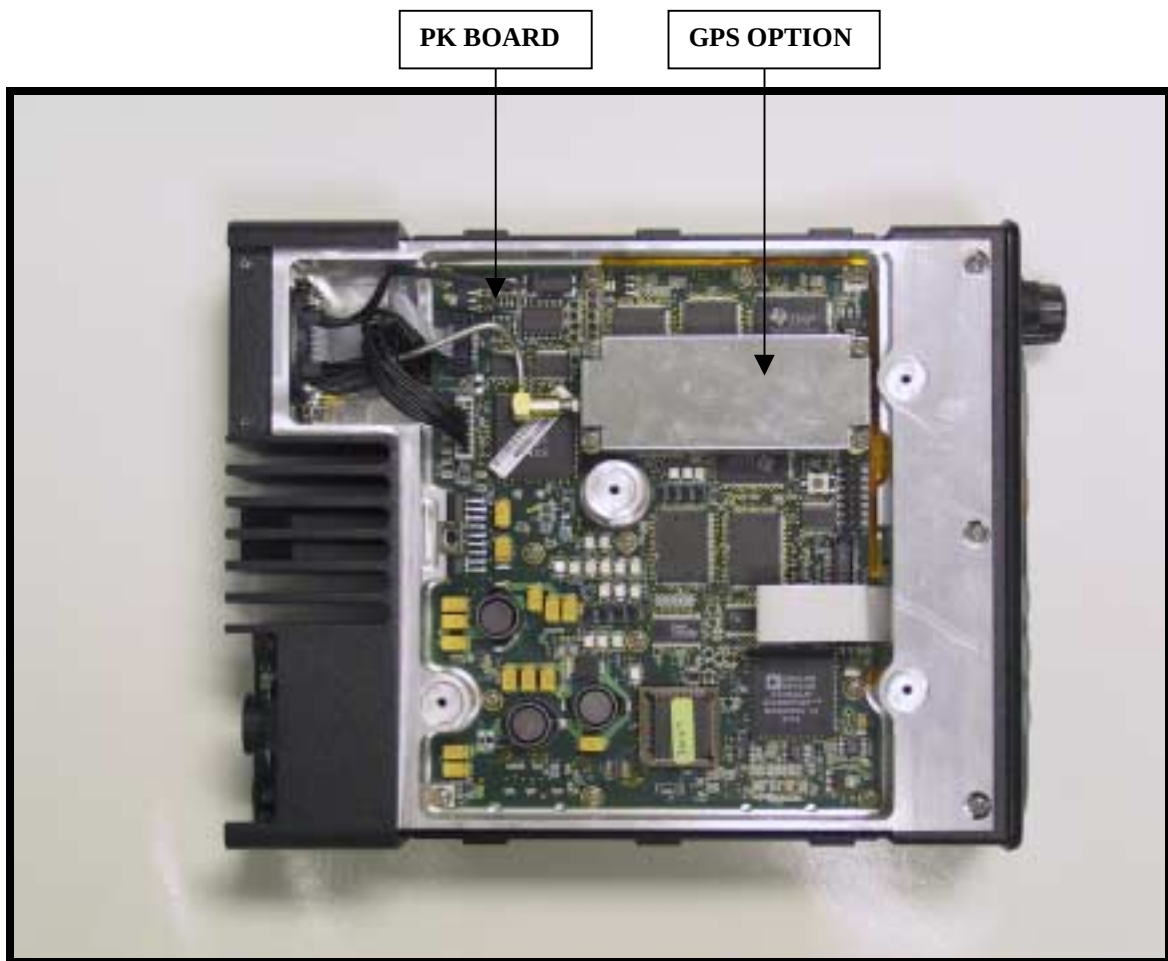
Figure 8 Radio Bottom View with Cover Removed
