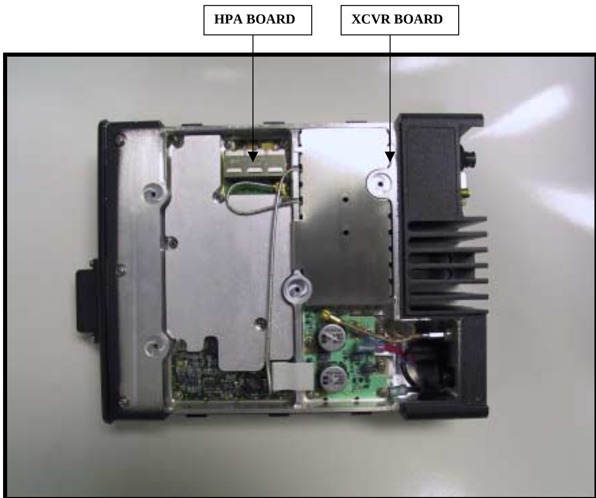
Figure 7 Radio Top View with Cover Removed
