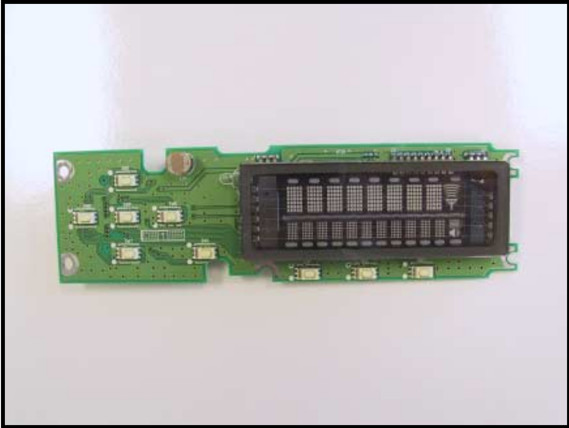
Figure 9 Display Board Top View
