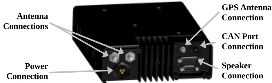
Figure 1 Rear Panel
