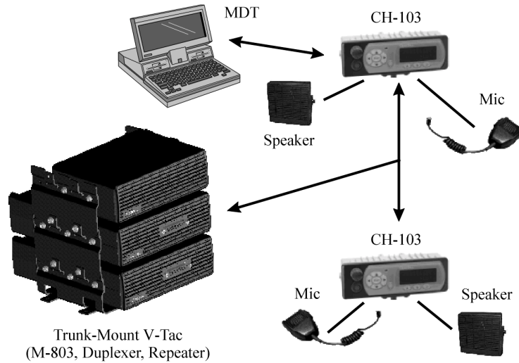
Figure 26 VTac Vehicular Tactical Network Sample Installation
