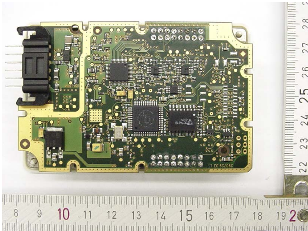
Photograph 5: Internal View of the EUT; Controller P.C.B.
