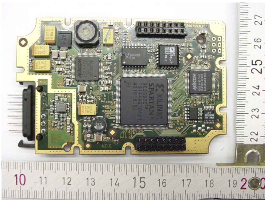
Photograph 6: Internal View of the EUT; Controller P.C.B.
