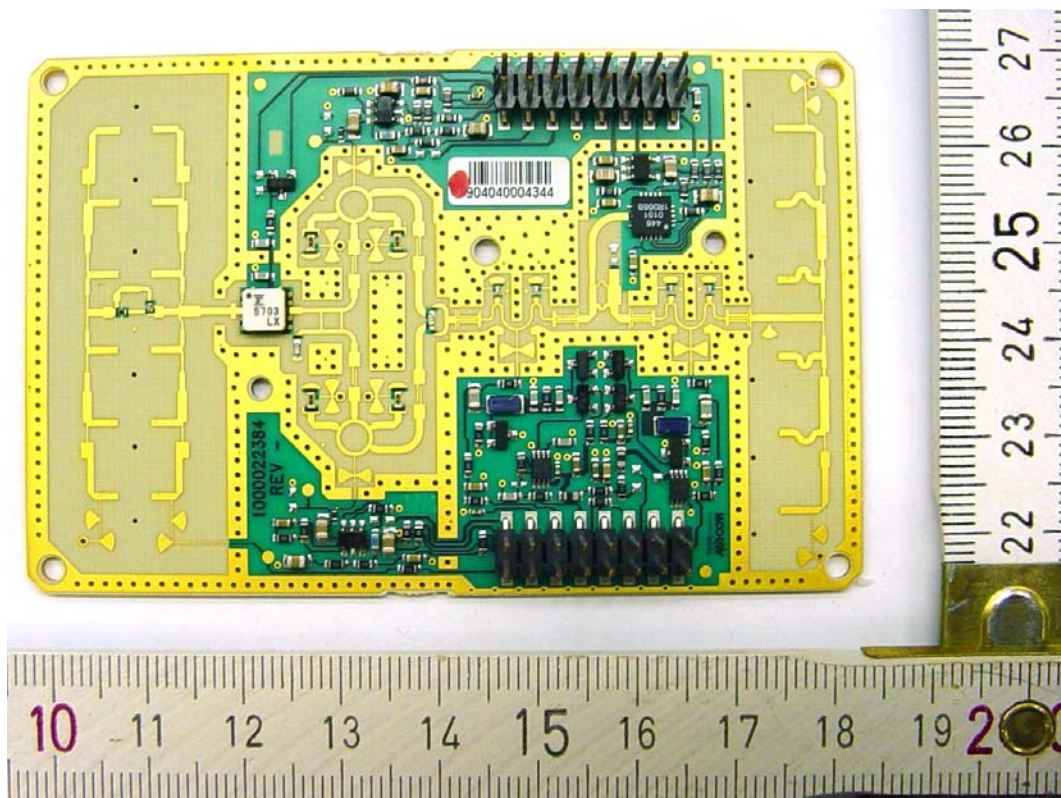
Photograph 3: Internal View of the EUT; RF P.C.B.
