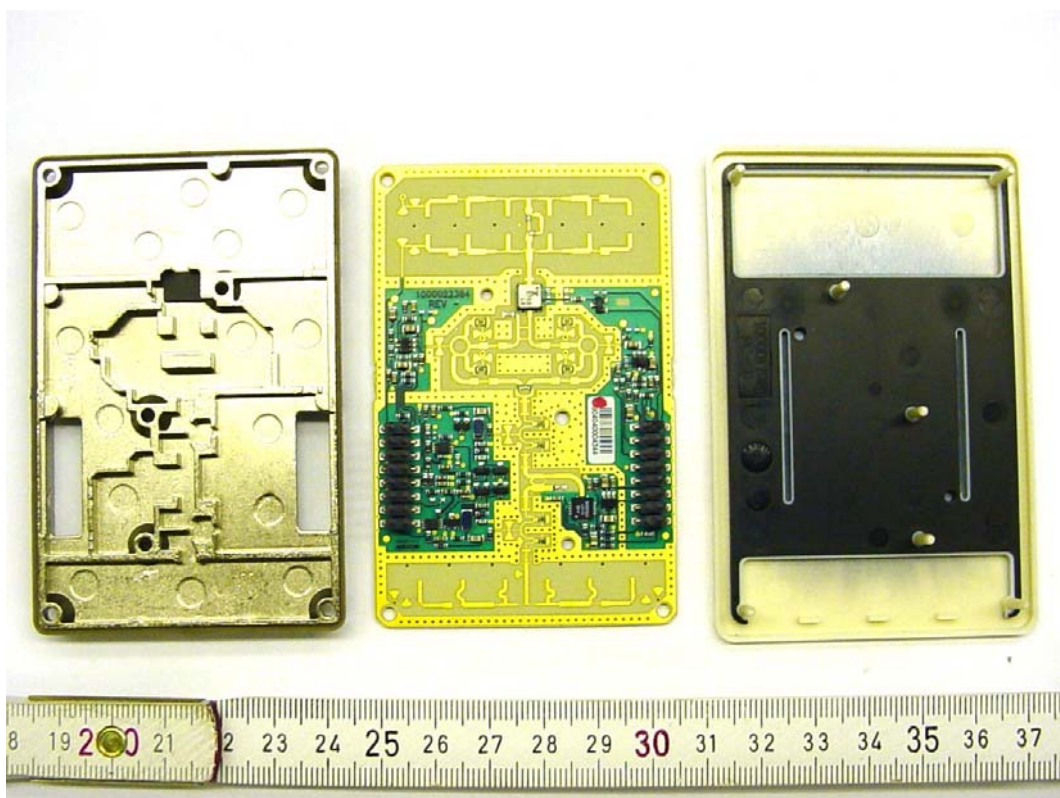
Photograph 2: Internal View of the EUT; RF Assembly
