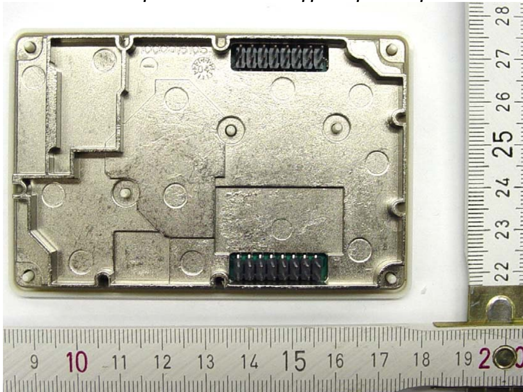
Photograph 1: Internal View of the EUT; RF Assembly
