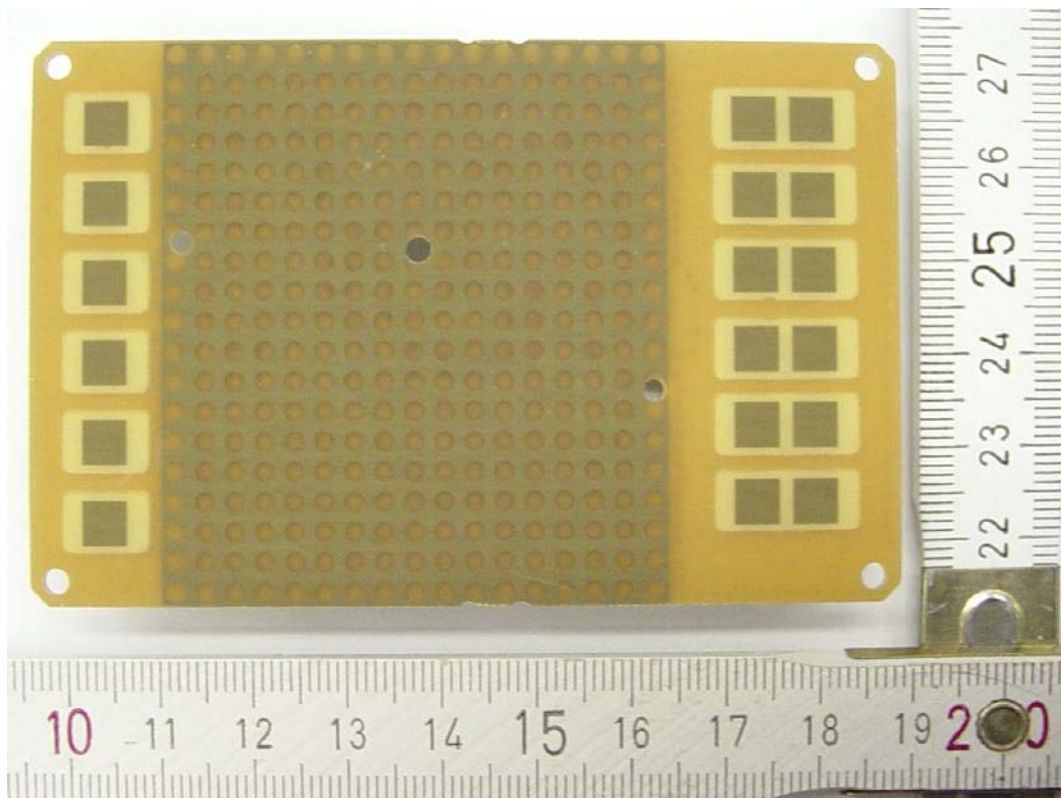
Photograph 4: Internal View of the EUT; RF P.C.B.
