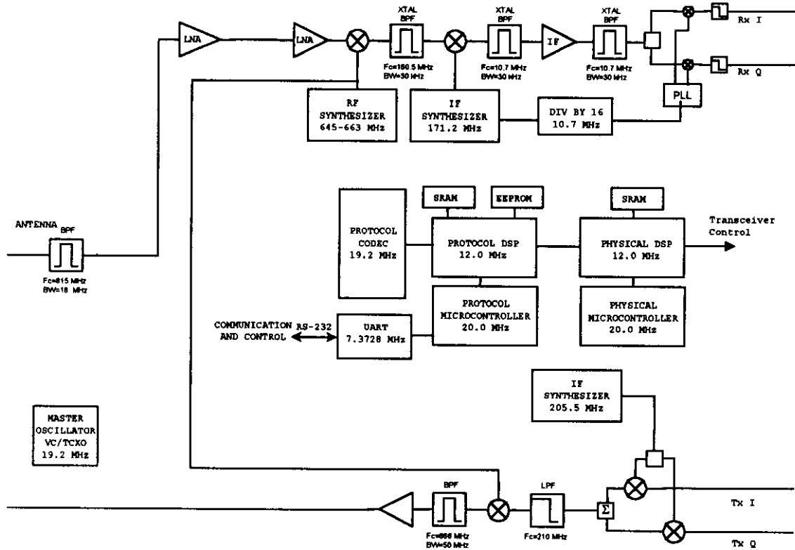
Transceiver Sub-Assembly Block Diagram showing Clock Frequencies
