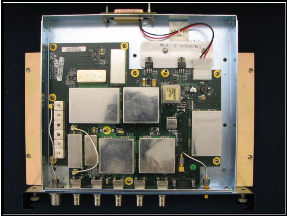
Photograph 4: BSX Configured for Passive Duplexer
