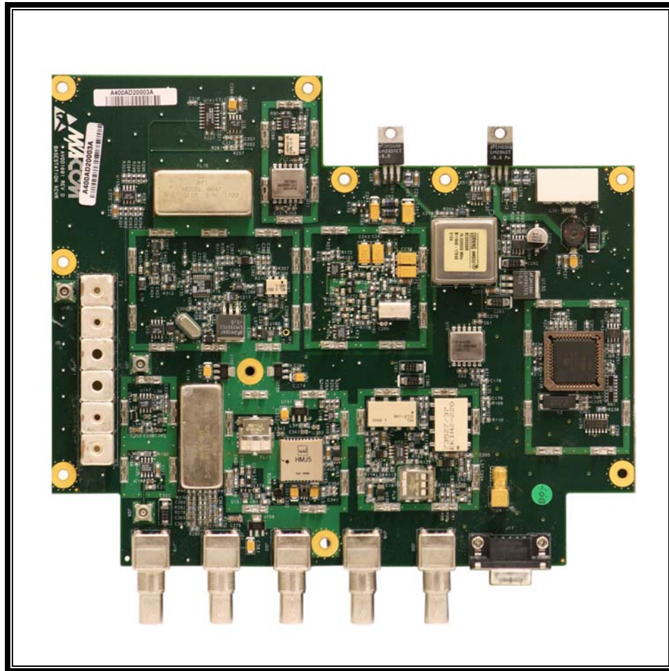
Photograph 5: BSX PCB Top View
