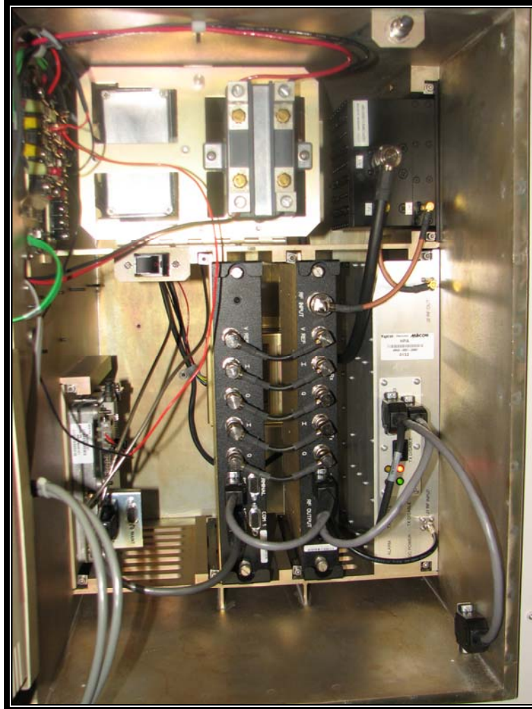
Photograph 3: 800 MHz Cell Site Interior with Passive Duplexer
