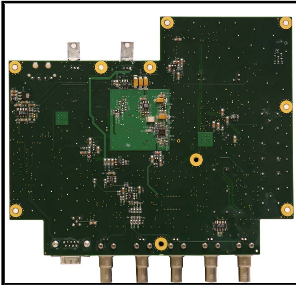
Photograph 6: BSX PCB Bottom View
