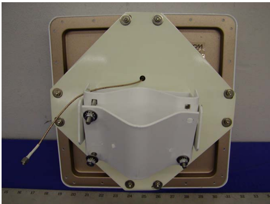
16dBi Directional Patch Antenna – Rear View
