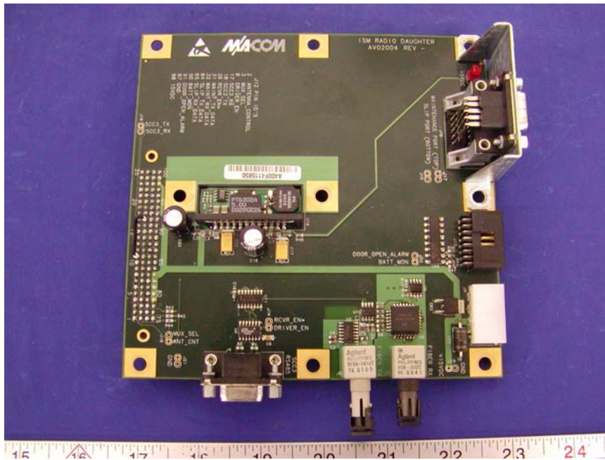
EUT – Layer 1 Main Board Component View
