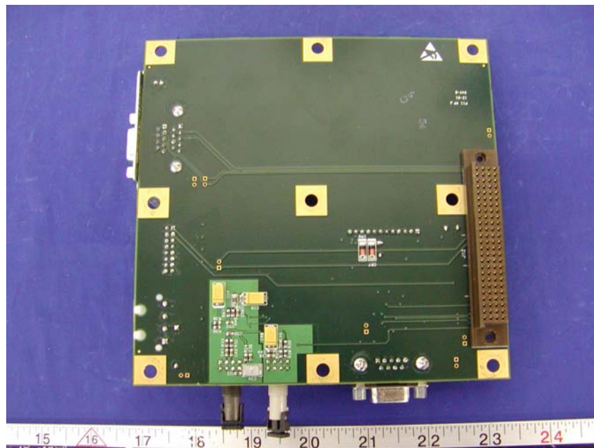
EUT – Layer 1 Main Board Solder View
