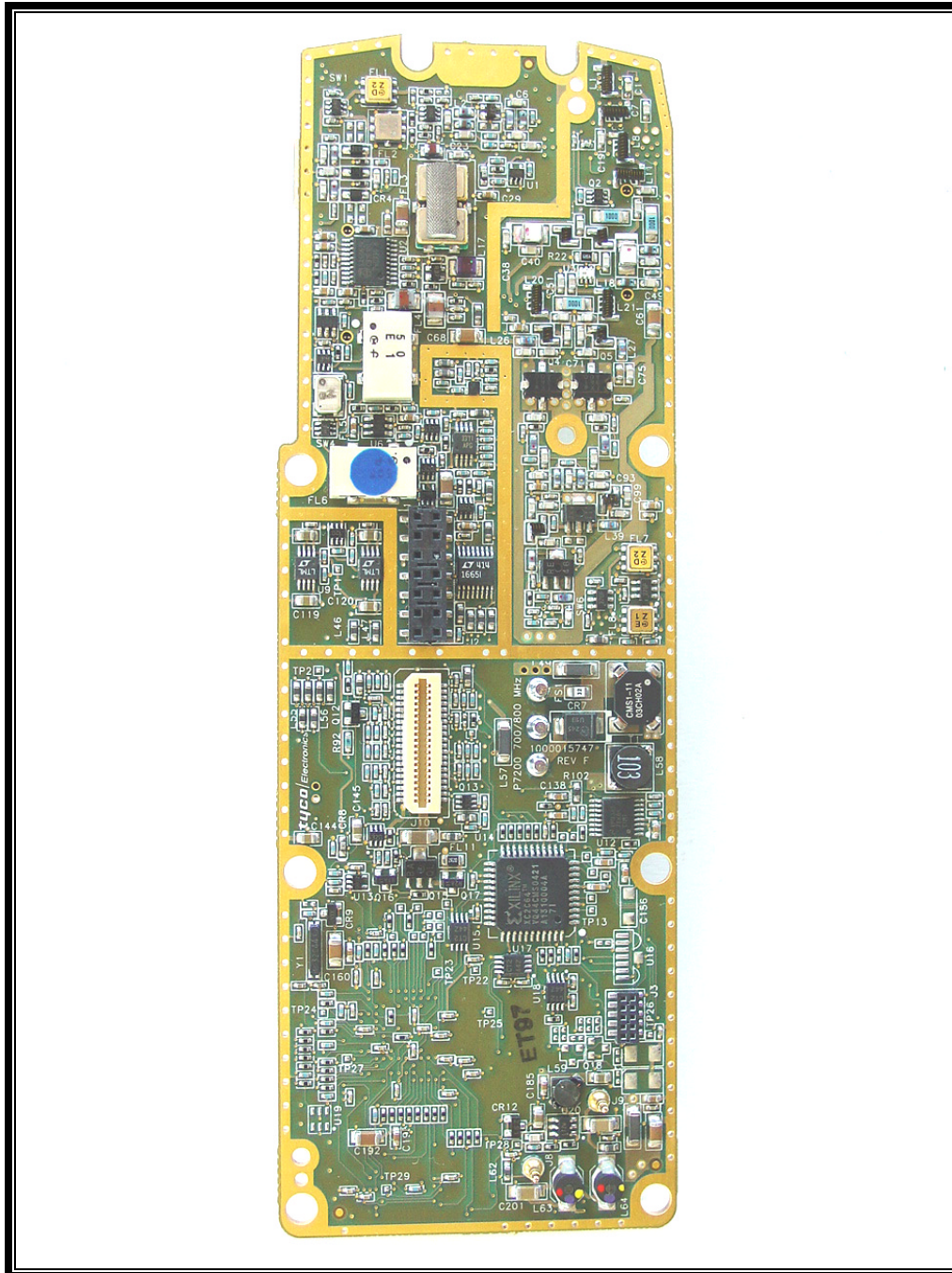
PHOTOGRAPH 11: PCB FRONT VIEW
