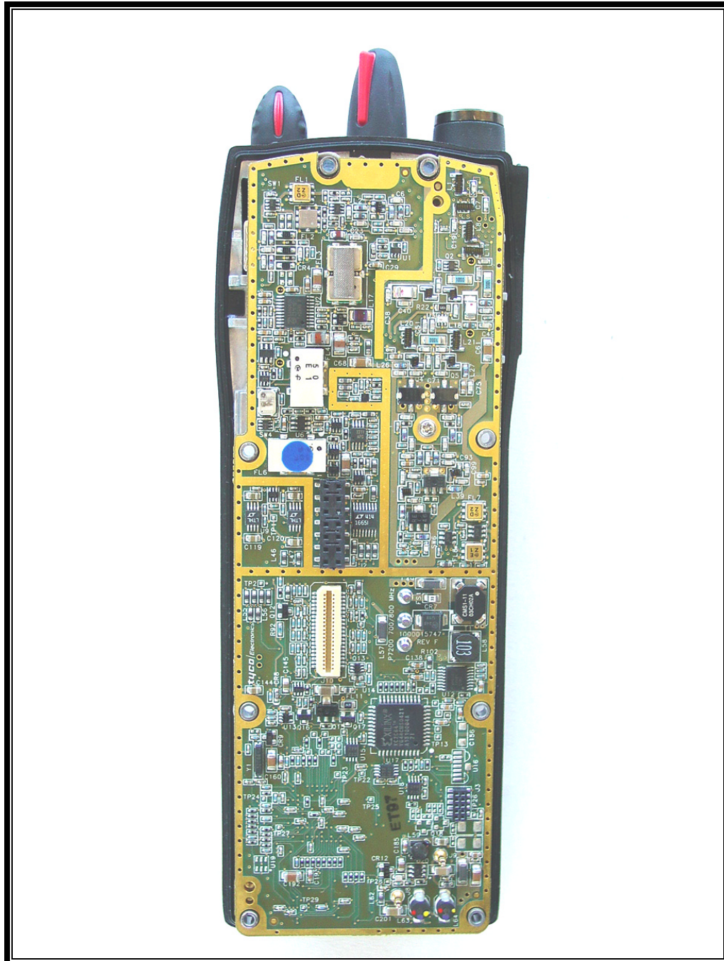
PHOTOGRAPH 10: MOUNTED BOARD
