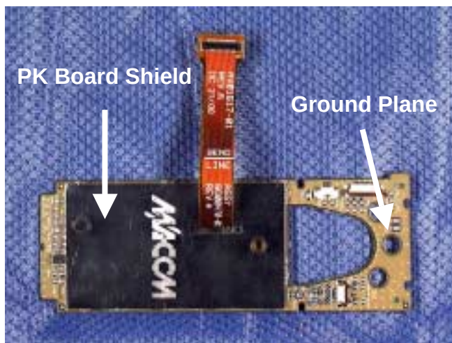
Figure 7a - Transceiver Side
