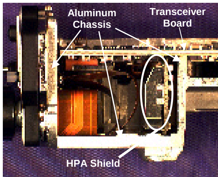
Figure 9 - BV8P800 Close-up Cross-Section Photograph - HPA Board Shielding
