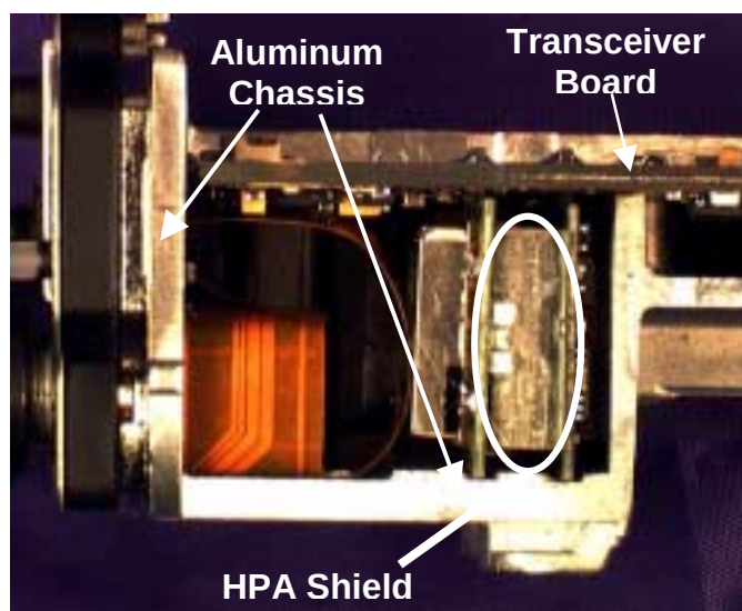
Figure A2-3 - BV8P-801T Close-up Cross-Section Photograph - HPA Board Shielding
