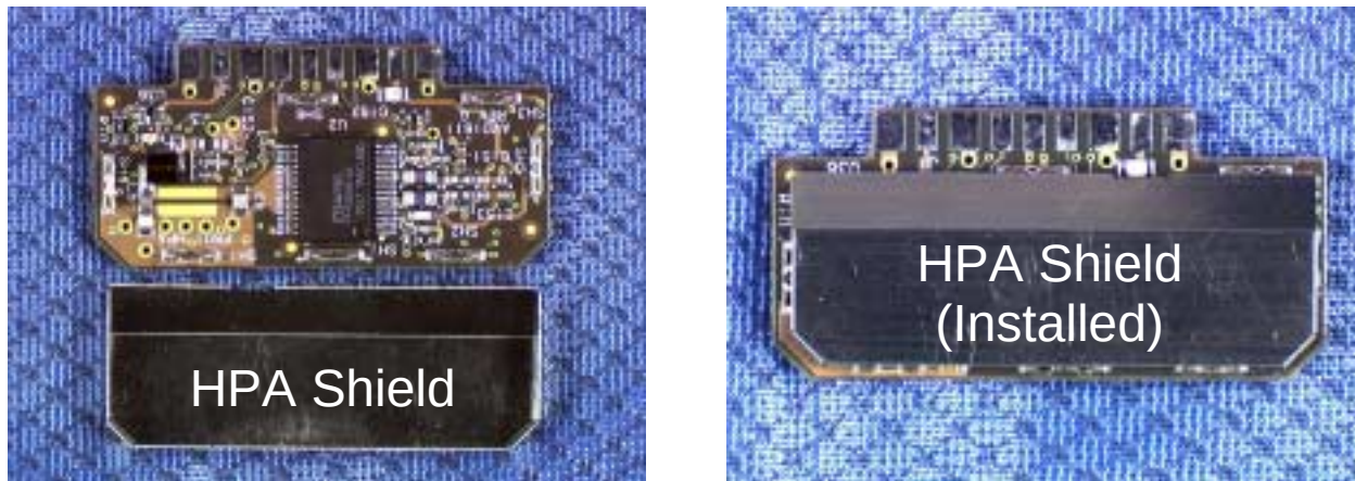
Figure 3 - HPA Board &amp; Shield
