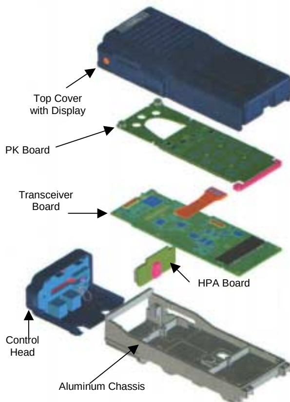
Figure 1 - BV8P800 Exploded Assembly Sketch
