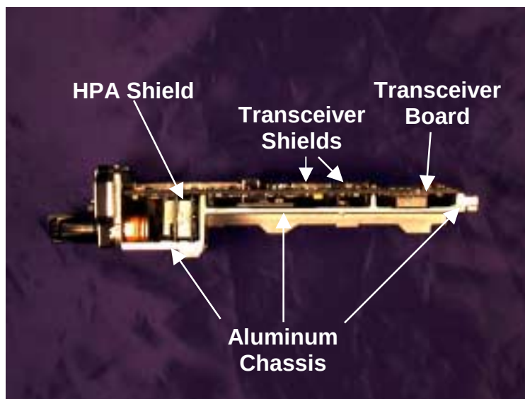
Figure A2-2 - BV8P-801T Cross-Section Photograph (Keypad and PK Board Removed)
