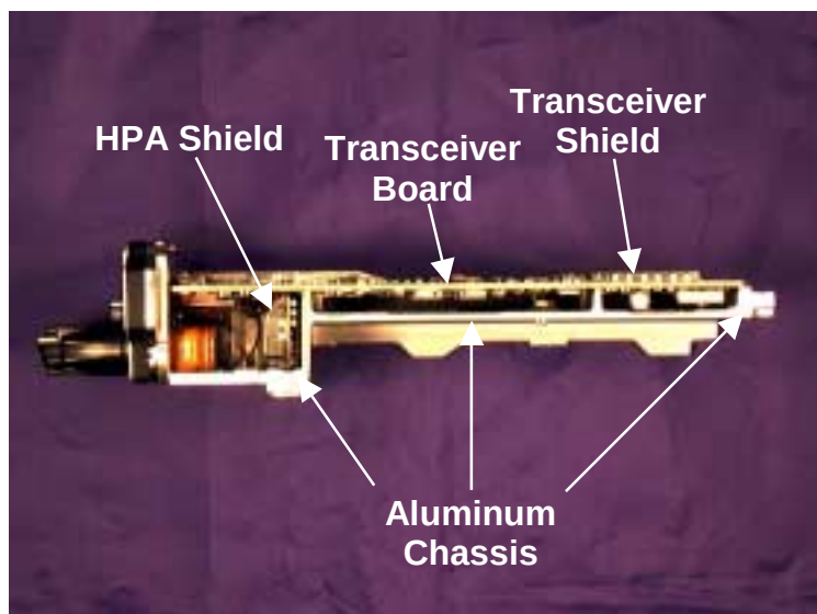
Figure 8 - BV8P801T Cross-Section Photograph (Top Cover and PK Board Removed)
