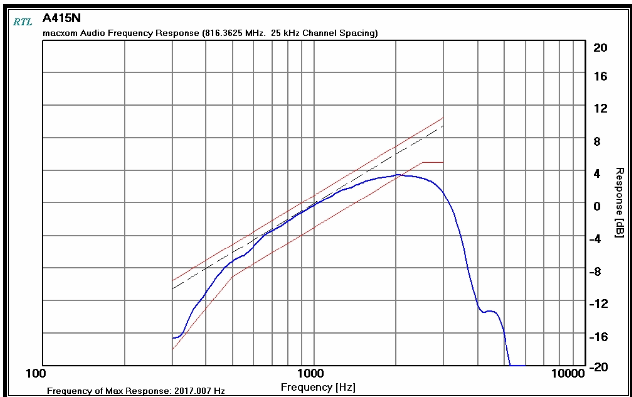
PLOT 4-1: AUDIO FREQUENCY RESPONSE
