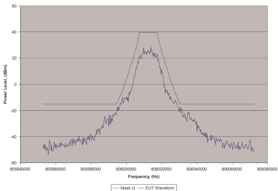
Emissions Mask G Channel 1
