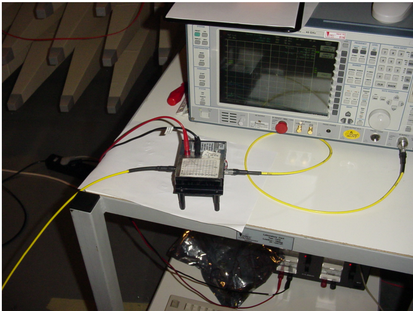
Photograph 3: Radiated Emissions Tests; Setup with Preamplifier and EMI Receiver
