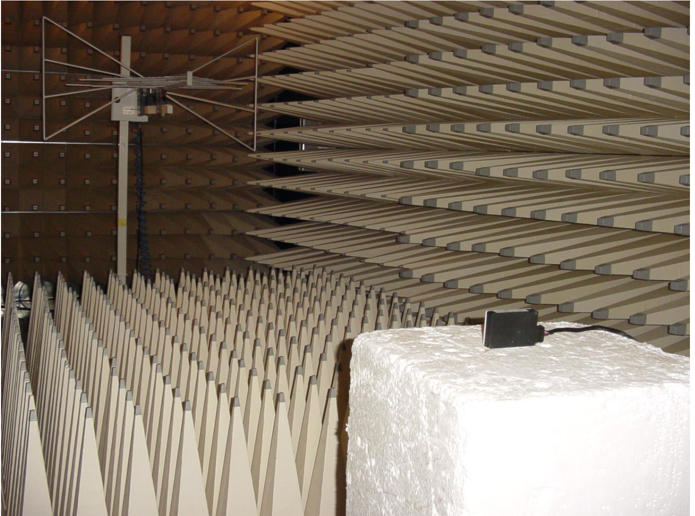
Photograph 1: Radiated Emissions Prescan up to 1 GHz
