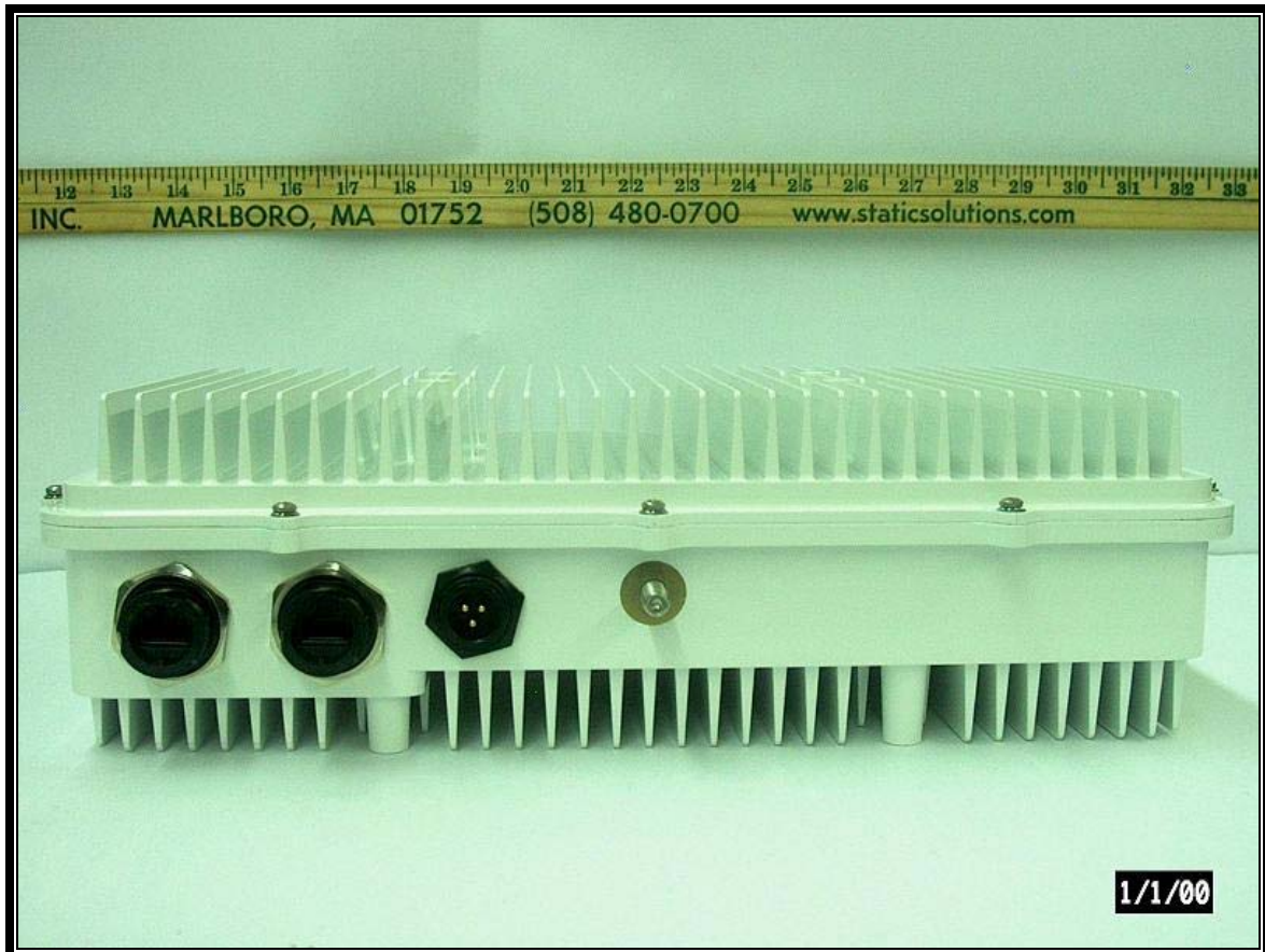
Photograph 7: Chassis Back
