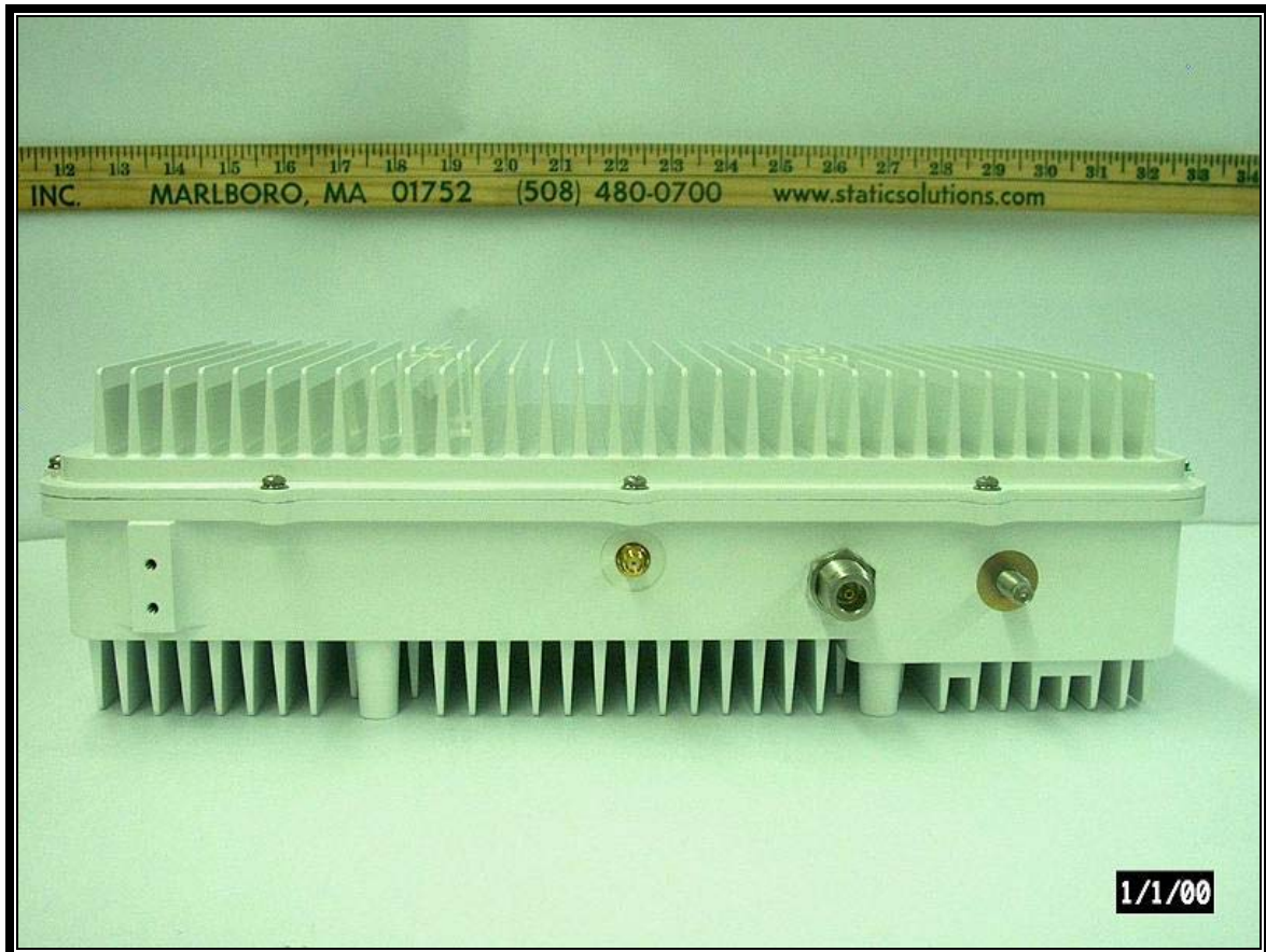
Photograph 6: Chassis Front
