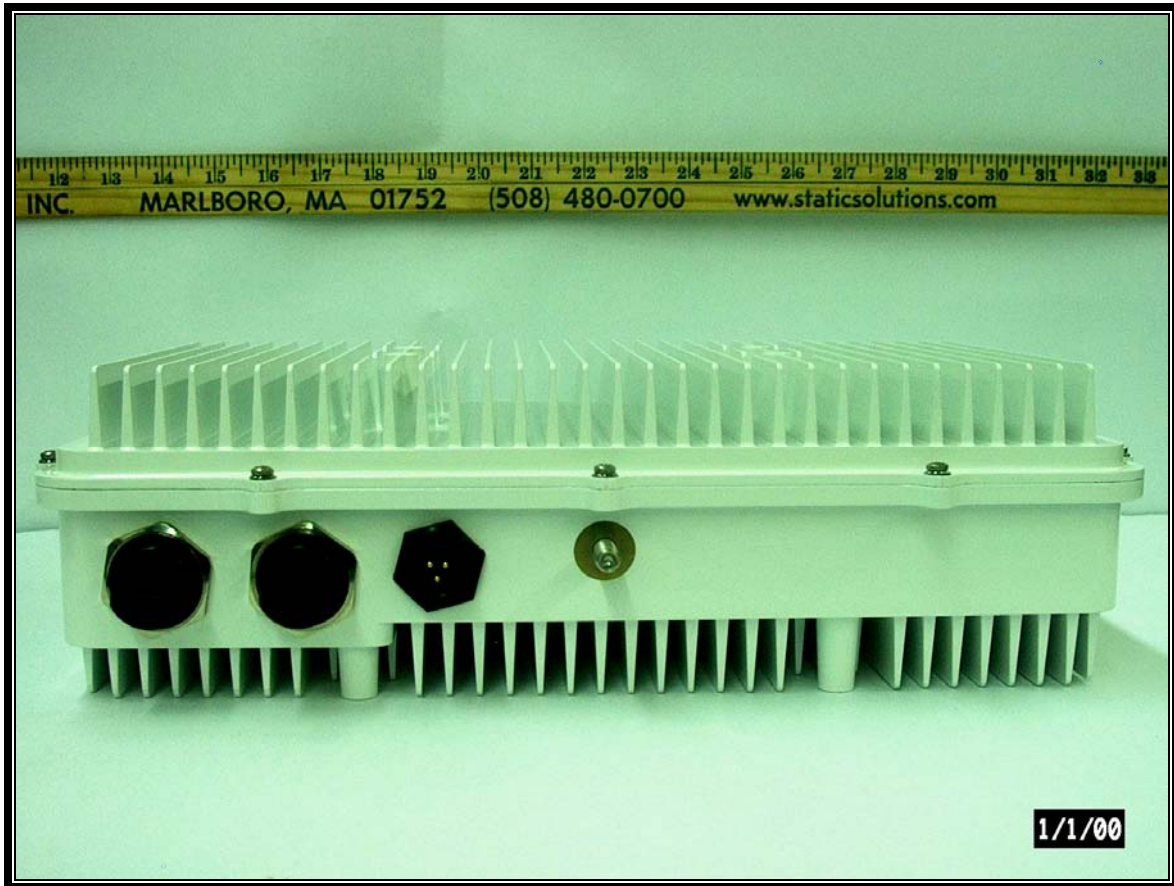
Photograph 4: Back
