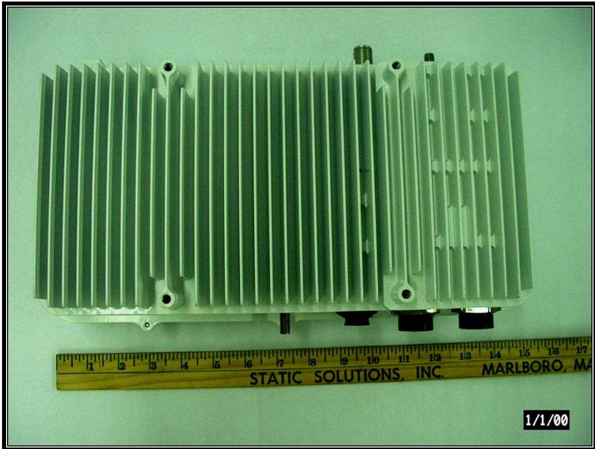
Photograph 2: Bottom
