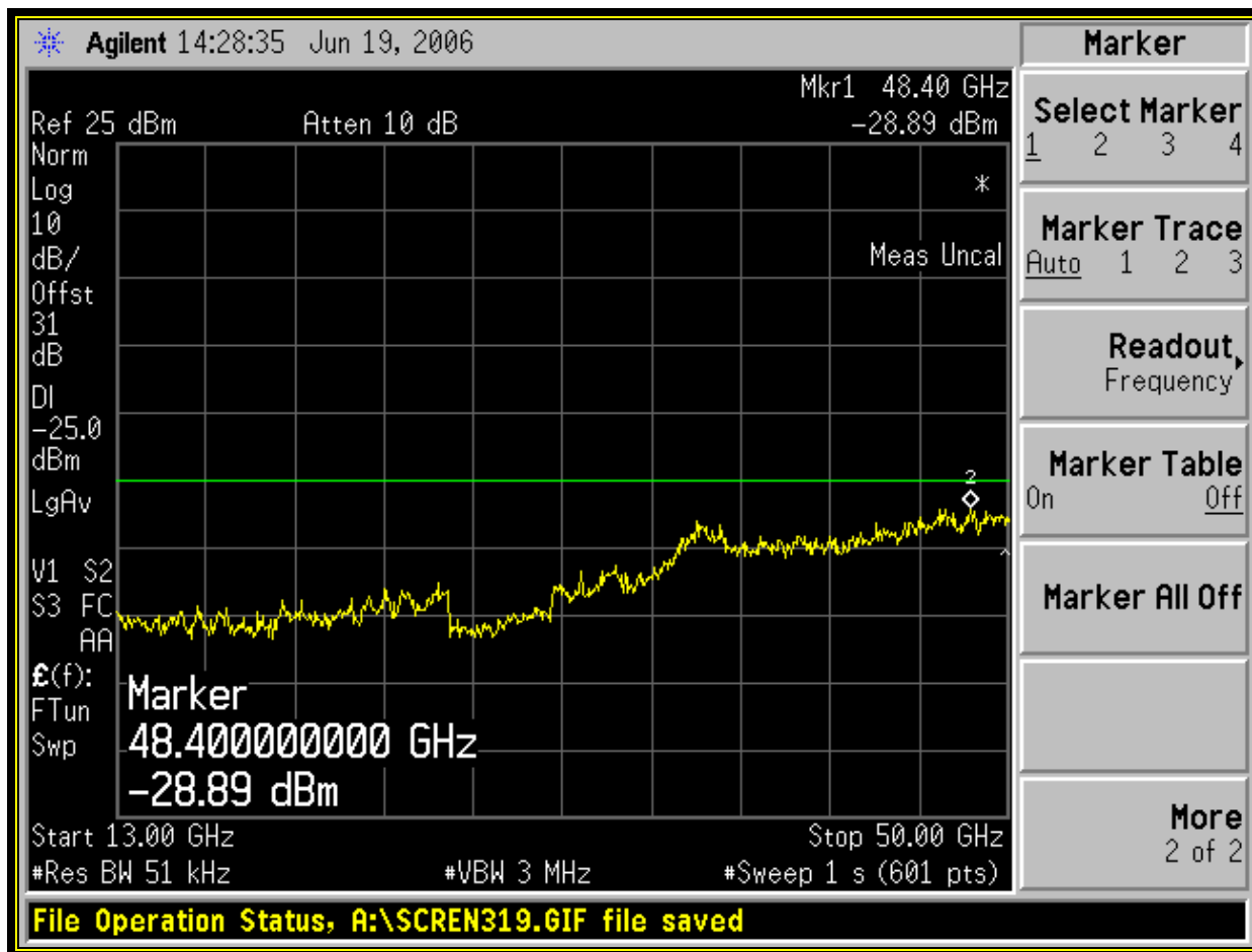
Plot 6-6: Conducted Spurious Emissions; Channel 9 – 4962.5 MHz; 13 GHz – 50 GHz
