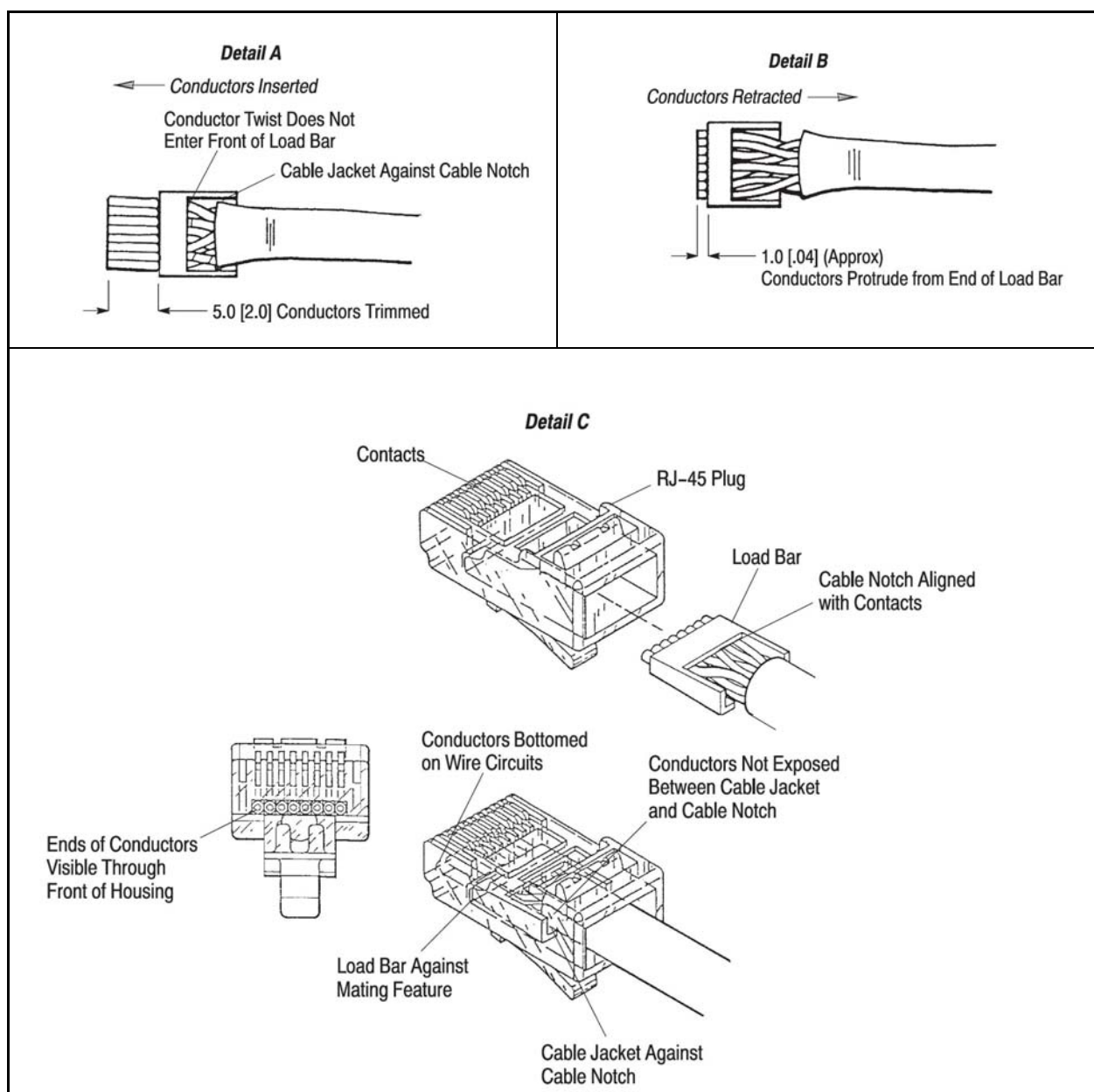
Figure 11-4: Termination Requirements
