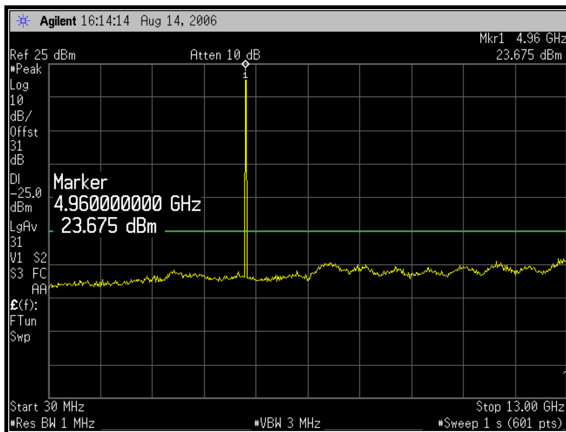
Plot 6-5: Conducted Spurious Emissions; Channel 9 – 4962.5 MHz; 30 MHz – 13 GHz
