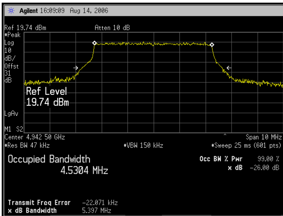
Plot 6-1: Occupied Bandwidth; Channel 3 - 4942.5 MHz
