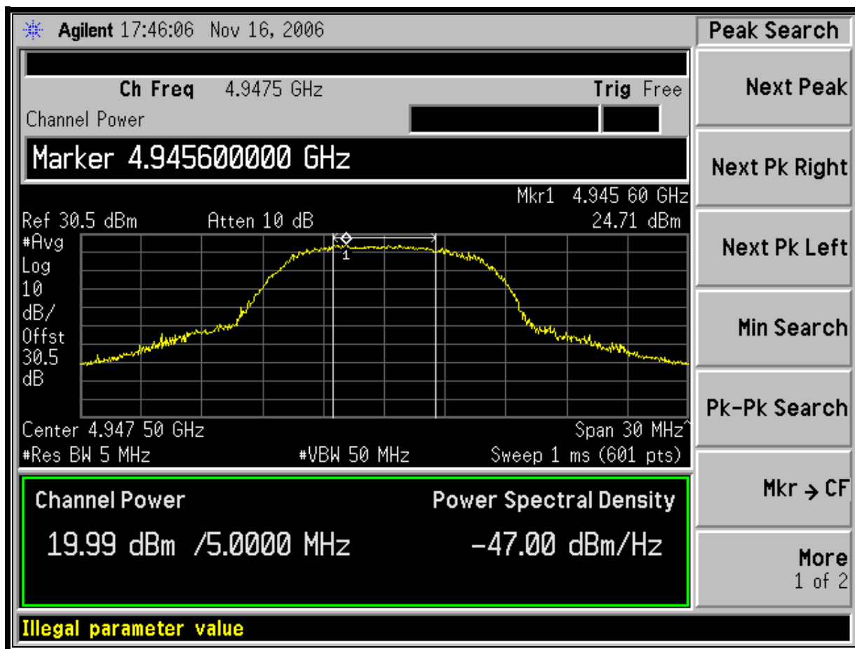
Plot 4-2: Channel Power Output; Channel 6 - 4947.5 MHz
