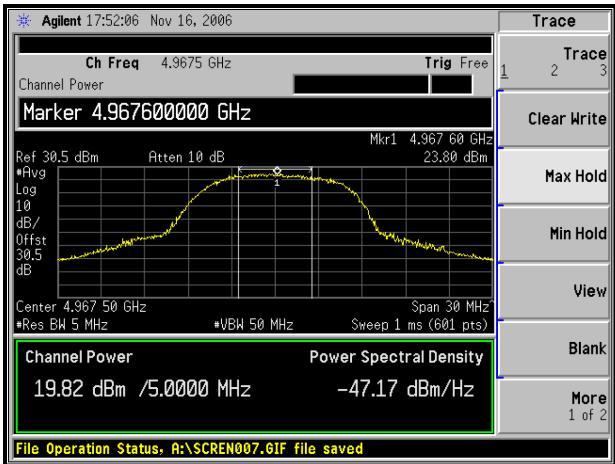
Plot 4-6: Channel Power Output; Channel 10 - 4967.5 MHz
