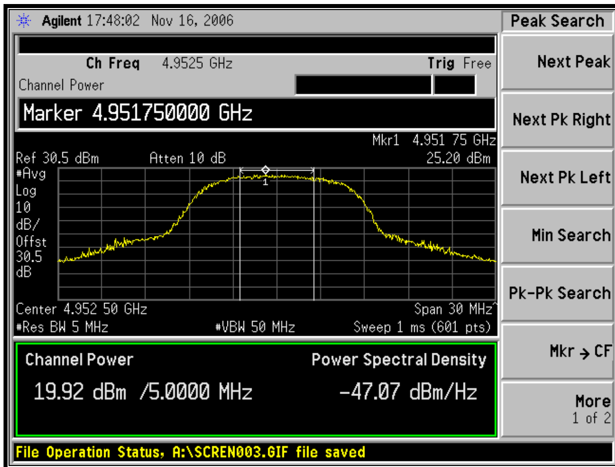
Plot 4-3: Channel Power Output; Channel 7 - 4952.5 MHz
