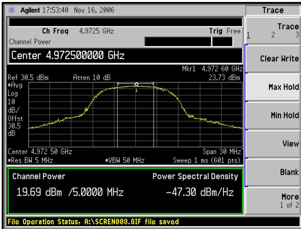
Plot 4-7: Channel Power Output; Channel 11 - 4972.5 MHz
