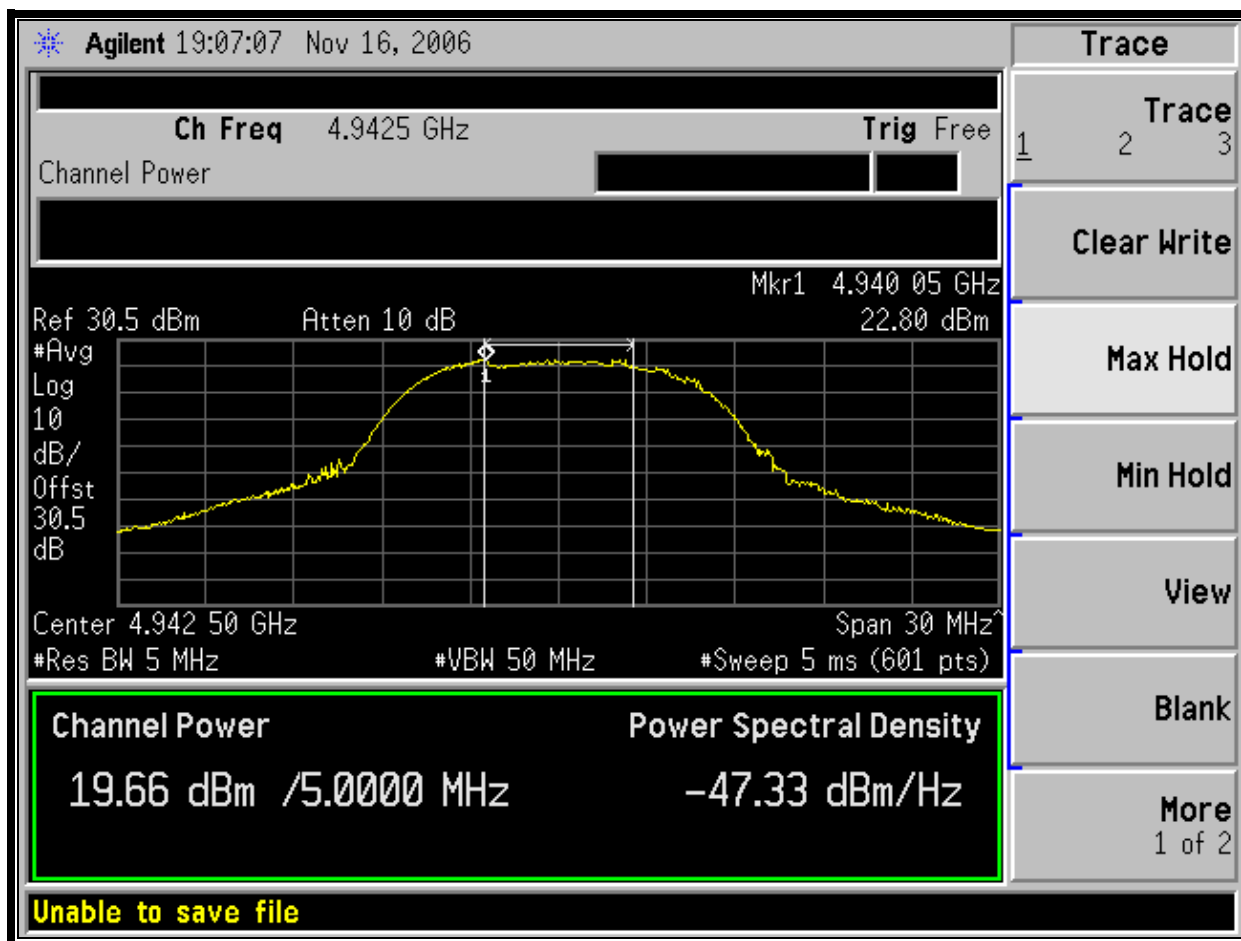
Plot 4-1: Channel Power Output; Channel 3 - 4942.5 MHz
