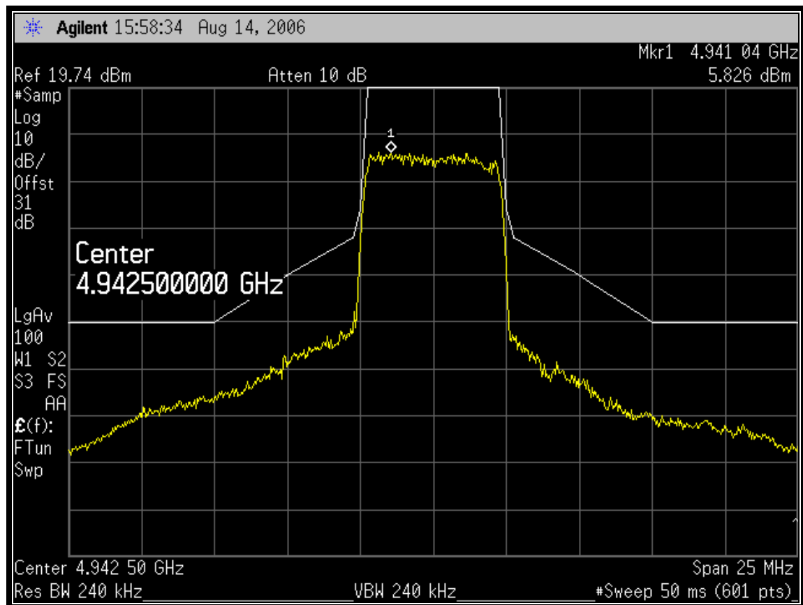
Plot 6-2: Emissions Mask M; Channel 3 - 4942.5 MHz
