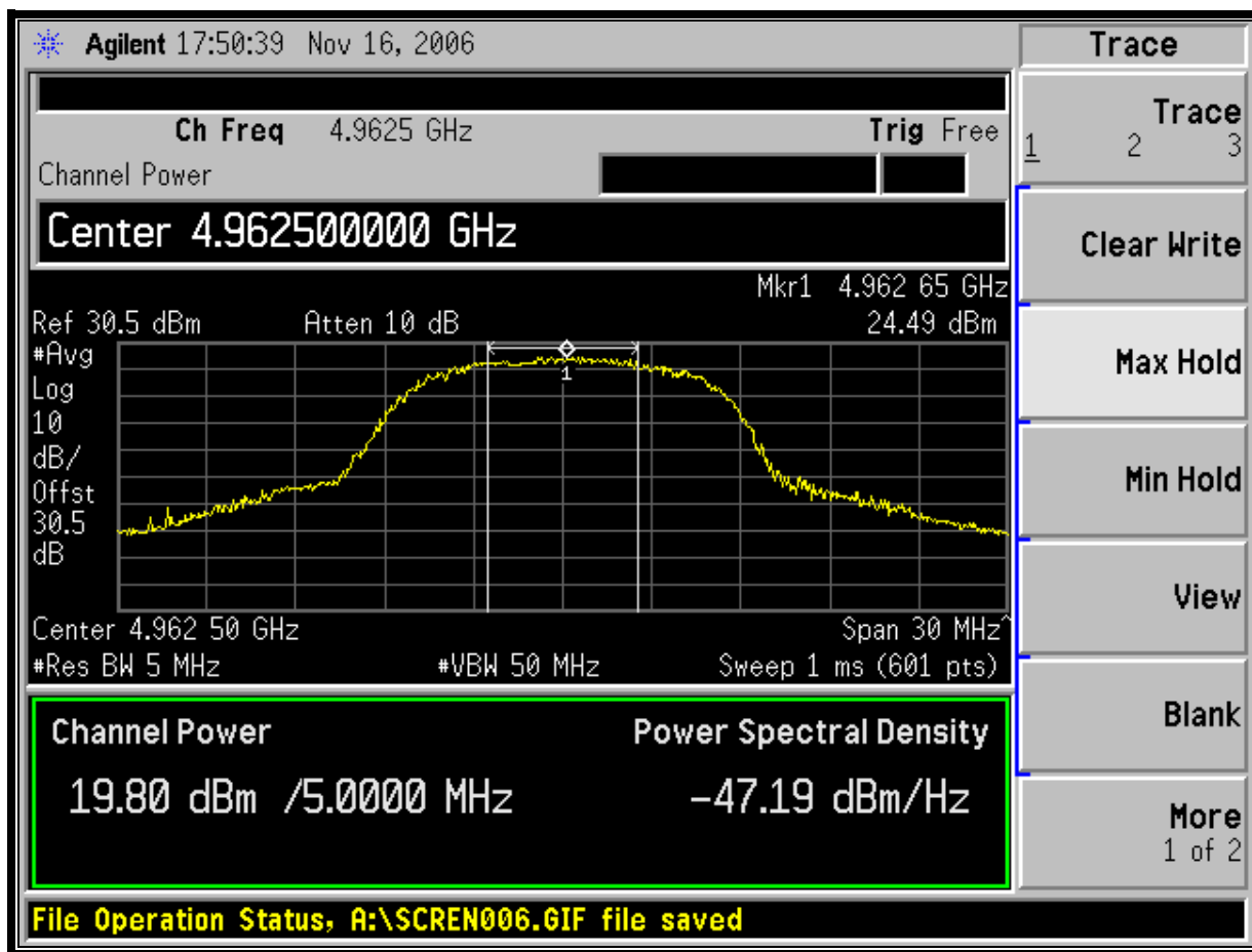
Plot 4-5: Channel Power Output; Channel 9 - 4962.5 MHz
