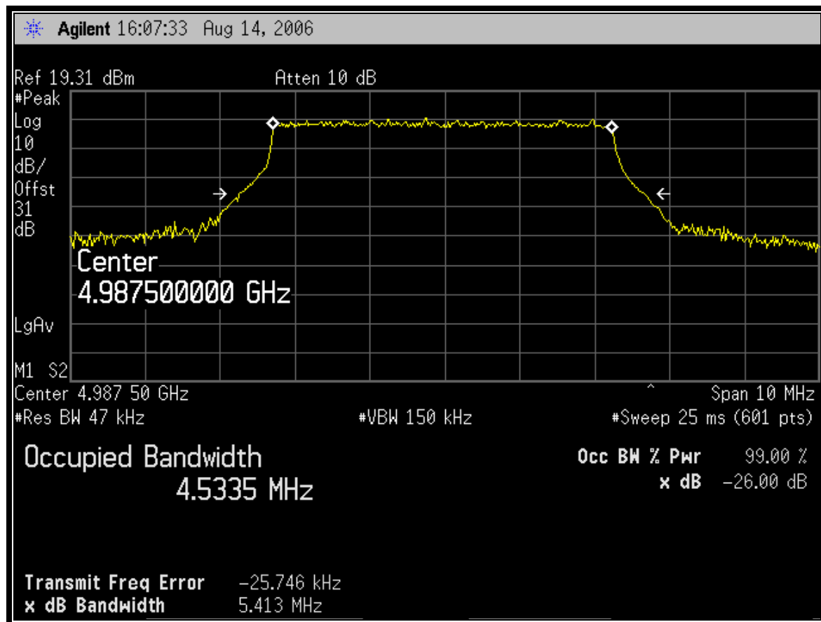
Plot 6-3: Occupied Bandwidth; Channel 16 - 4987.5 MHz
