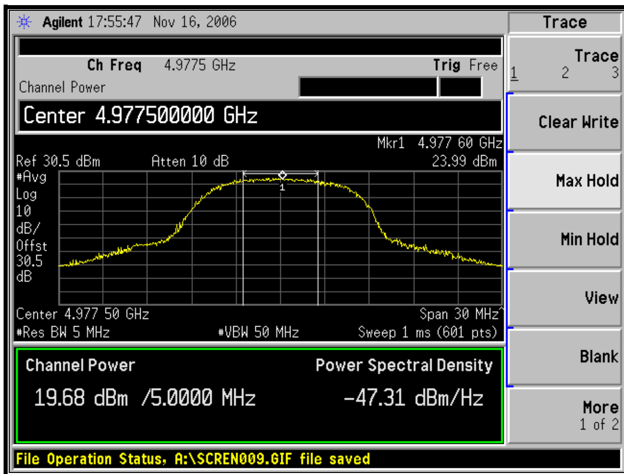
Plot 4-8: Channel Power Output; Channel 12 - 4977.5 MHz
