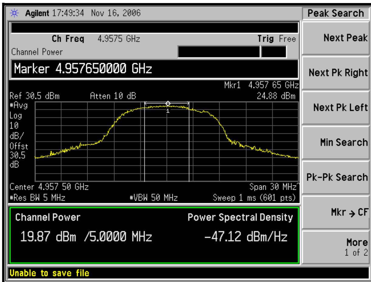
Plot 4-4: Channel Power Output; Channel 8 - 4957.5 MHz
