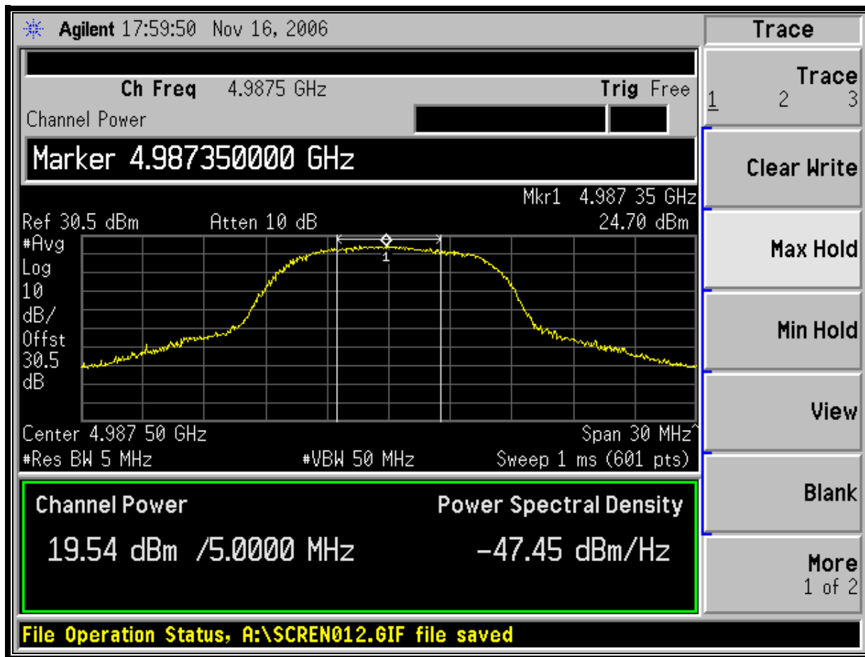
Plot 4-10: Channel Power Output; Channel 16 - 4987.5 MHz
