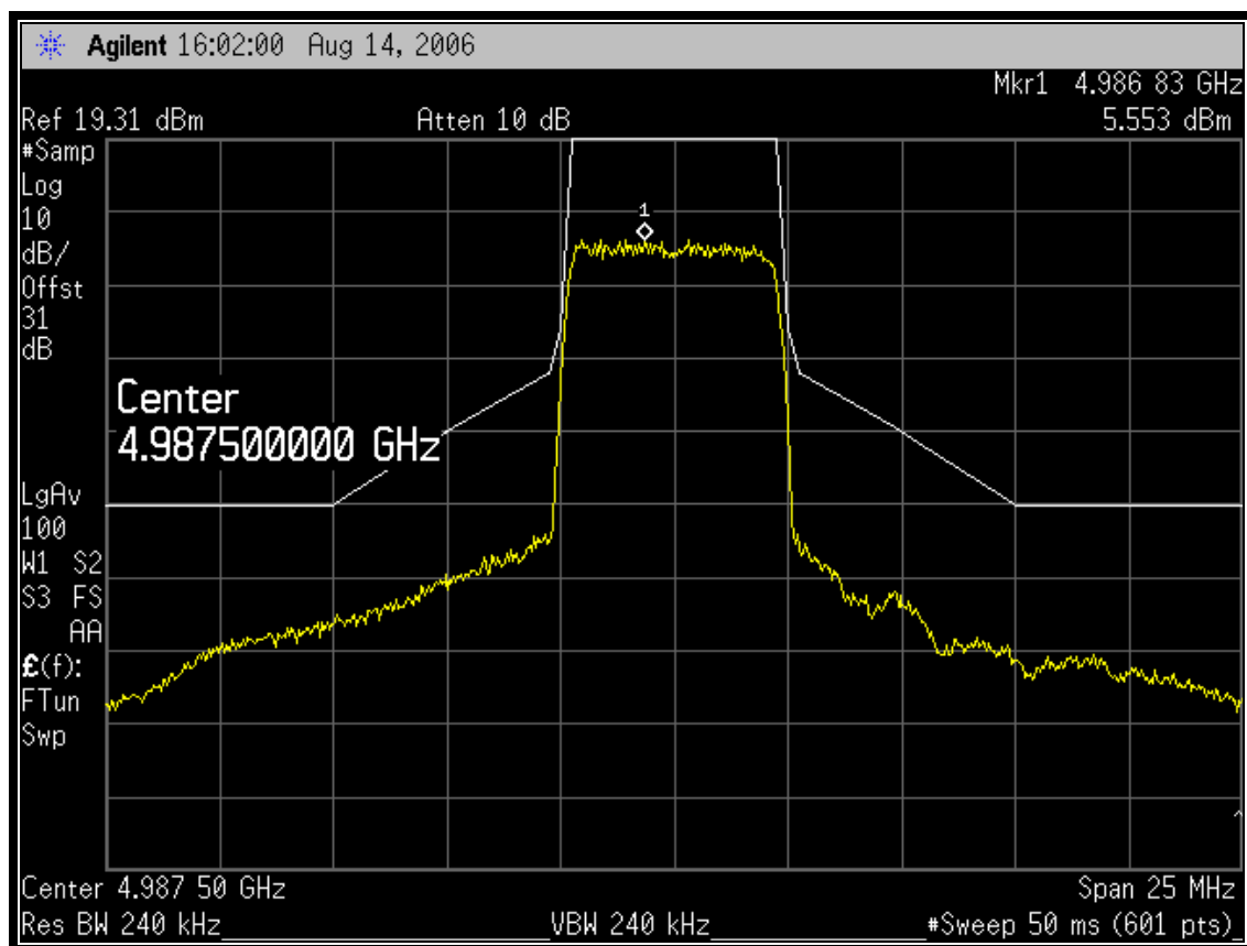
Plot 6-4: Emissions Mask M; Channel 16 - 4987.5 MHz
