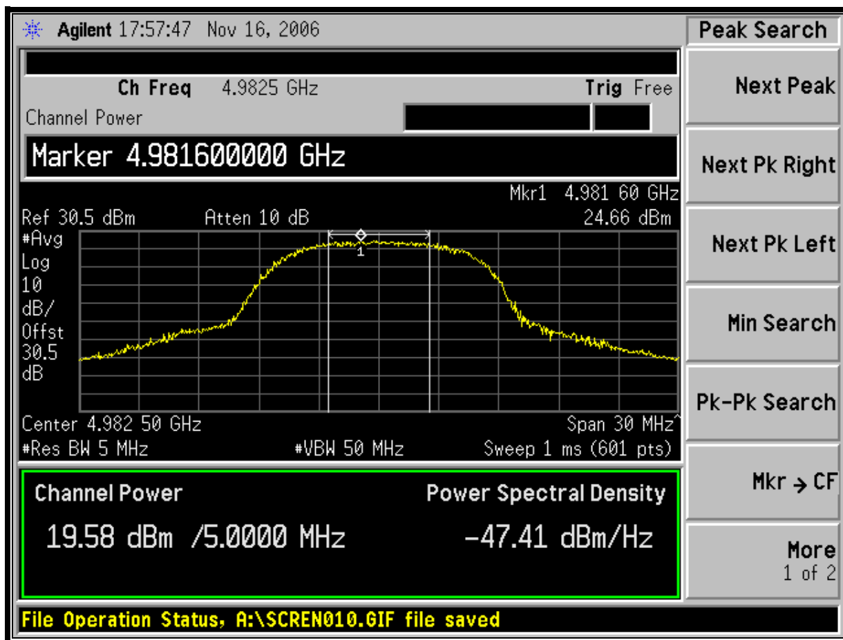
Plot 4-9: Channel Power Output; Channel 13 - 4982.5 MHz
