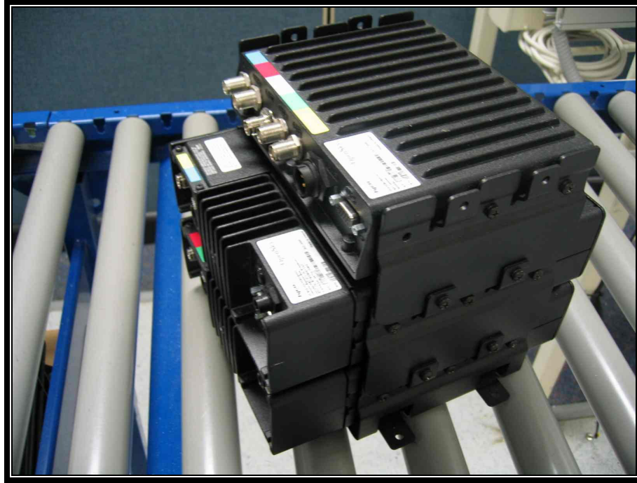
PHOTOGRAPH 7: V-TAC STACK-UP REAR VIEW
