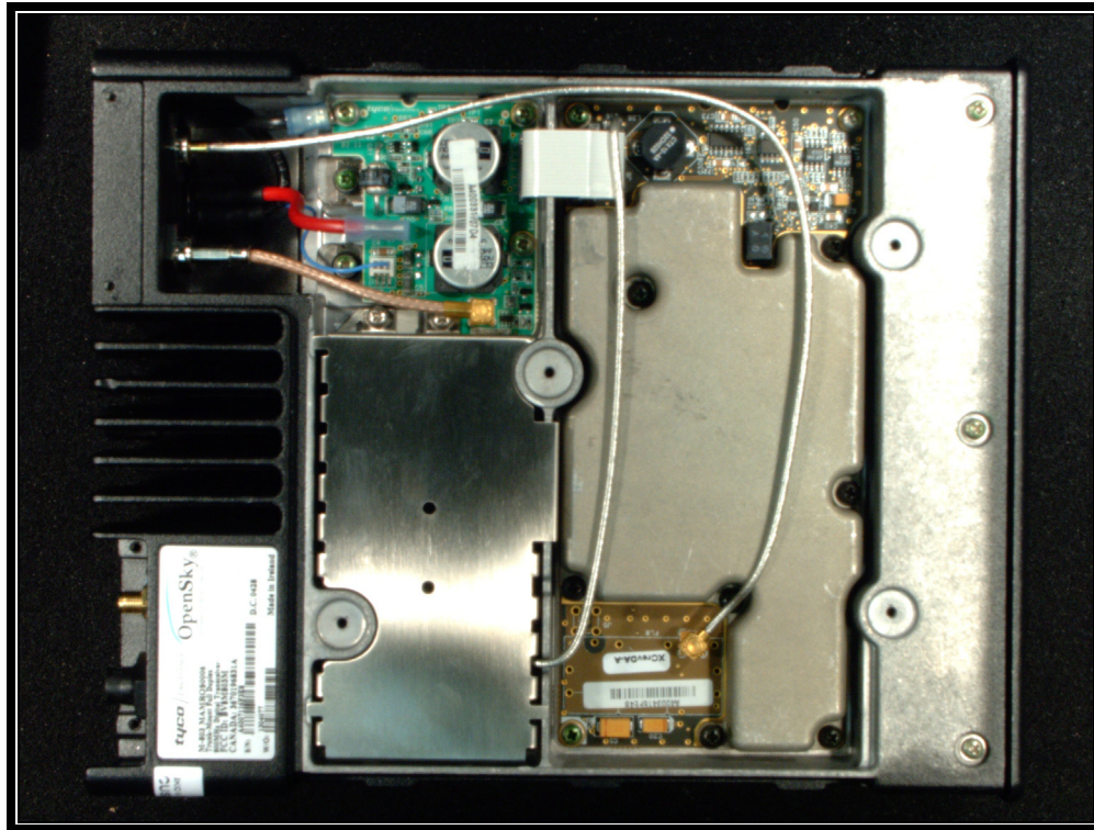
PHOTOGRAPH 9: RADIO TOP VIEW WITH SHIELDS
