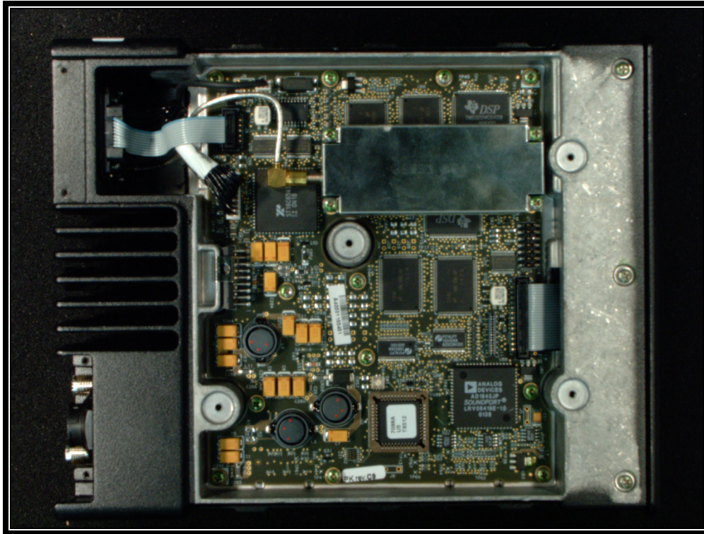
PHOTOGRAPH 11: RADIO BOTTOM VIEW WITH GPS UNIT
