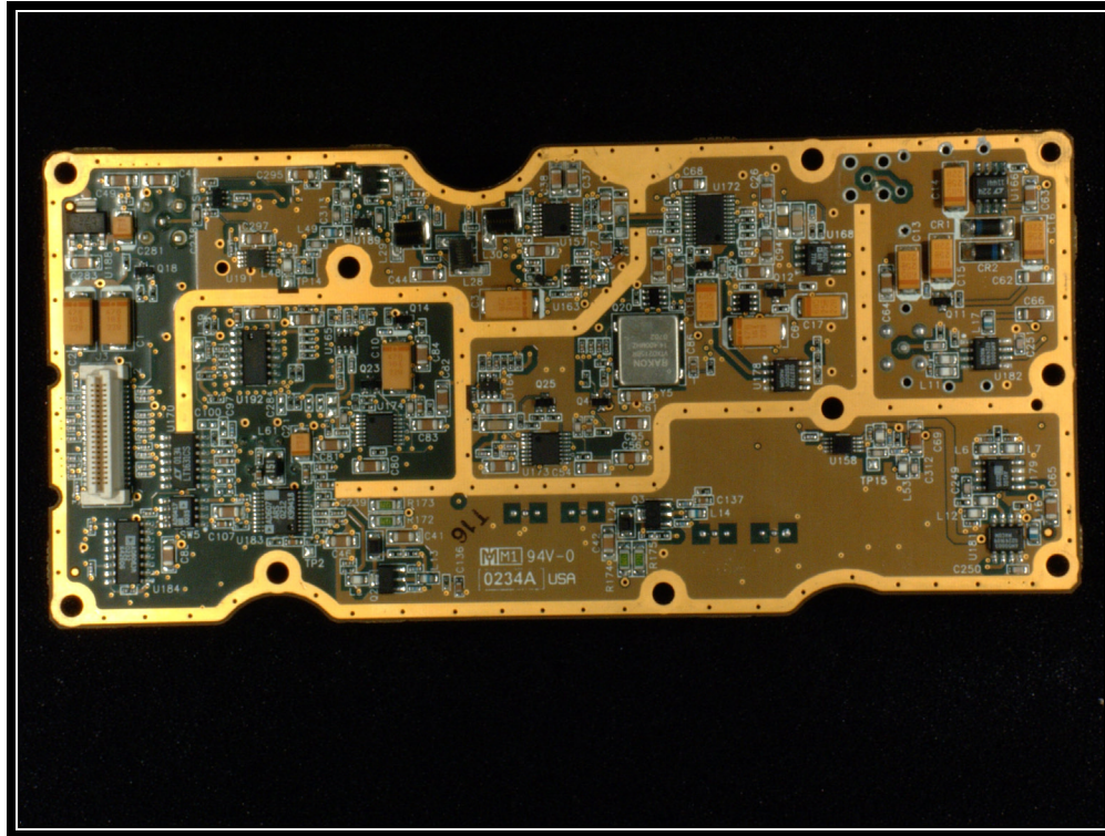
PHOTOGRAPH 17: XCVR PCB BOTTOM VIEW
