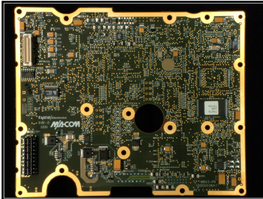
PHOTOGRAPH 15: PK PCB BOTTOM VIEW
