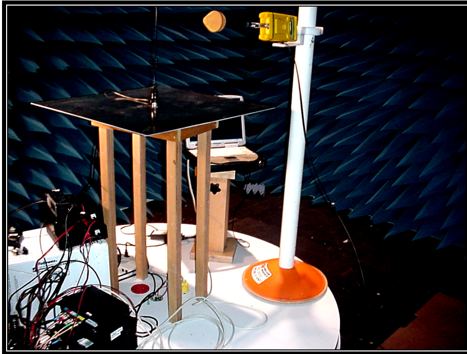
PHOTOGRAPH 5.2: TEST SETUP FOR MPE MEASUREMENTS FOR UNCONTROLLED ENVIRONMENT
