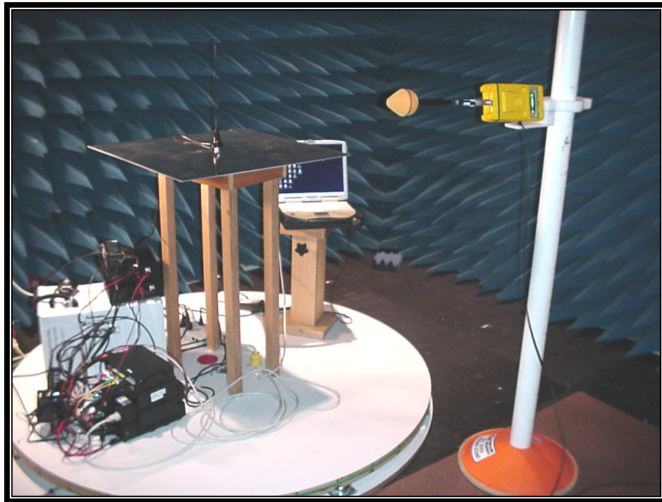
PHOTOGRAPH 5.1: TEST SET UP FOR MPE MEASUREMENTS FOR CONTROLLED ENVIRONMENT
