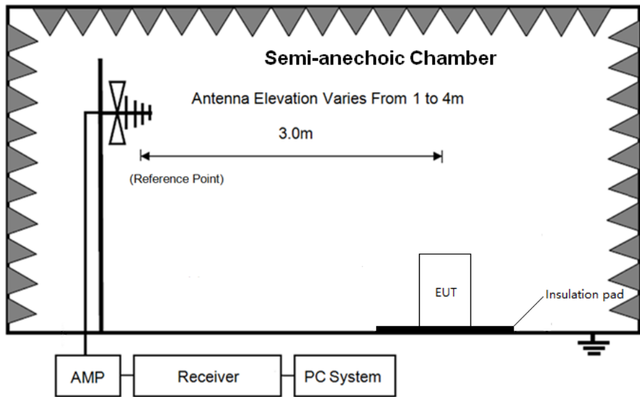
Test Setup Diagram for 30MHz~1GHz
