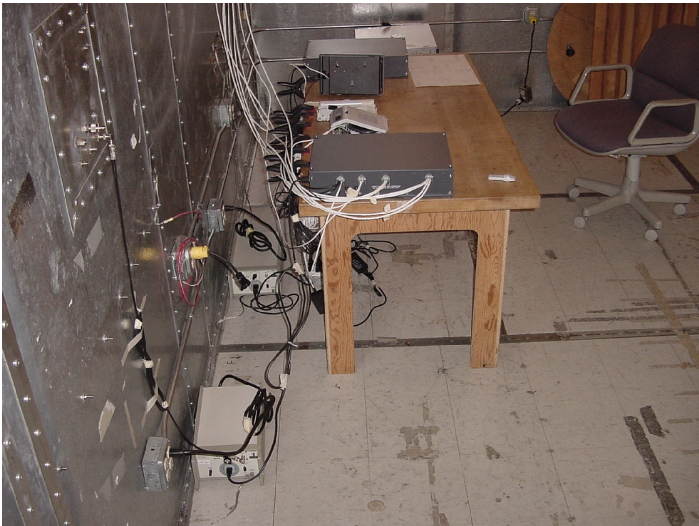
Measuring LISN, Accessory LISN and connections
