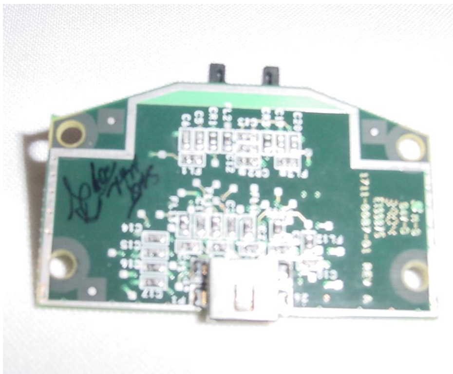
Internal Photo 5 – Base Interconnect PCB Bottom View
