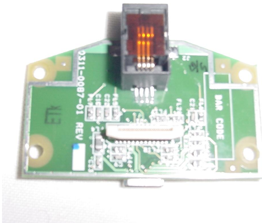
Internal Photo 6 – Base Interconnect PCB Top View
