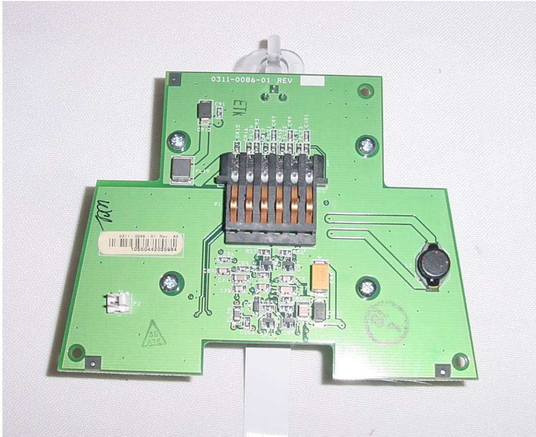
Internal Photo 1 – Base Charger PCB Top View
