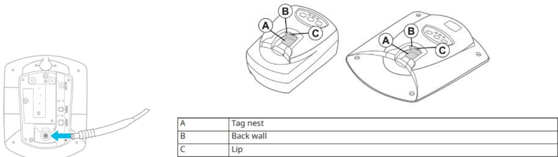
Figure 1: Components of an IDKM SuperTag detacher
